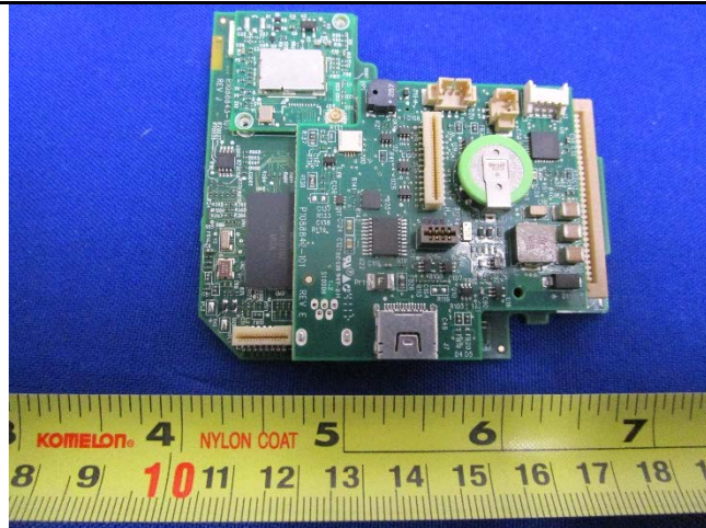
PCBA 1 View with radio module
