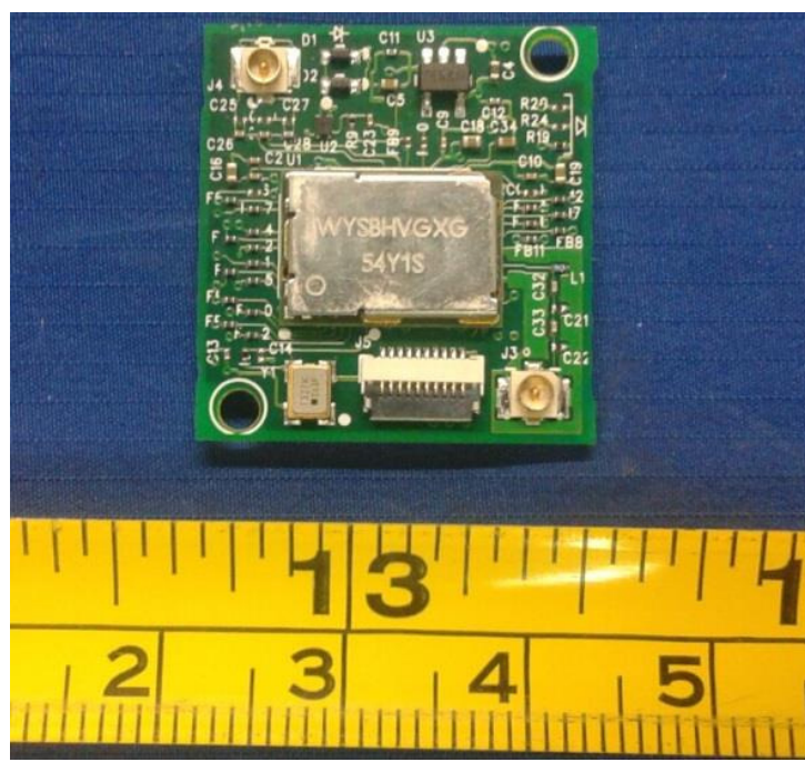
EUT Radio with Shielding Top View
