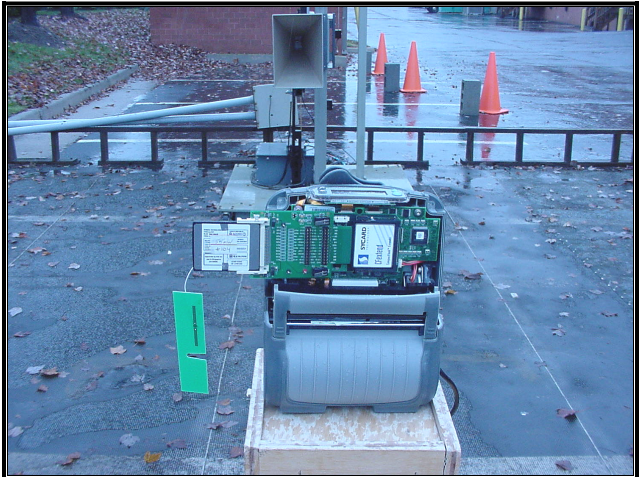
PHOTOGRAPH 3: RADIATED EMISSION FRONT VIEW USING CQ17110 ANTENNA
