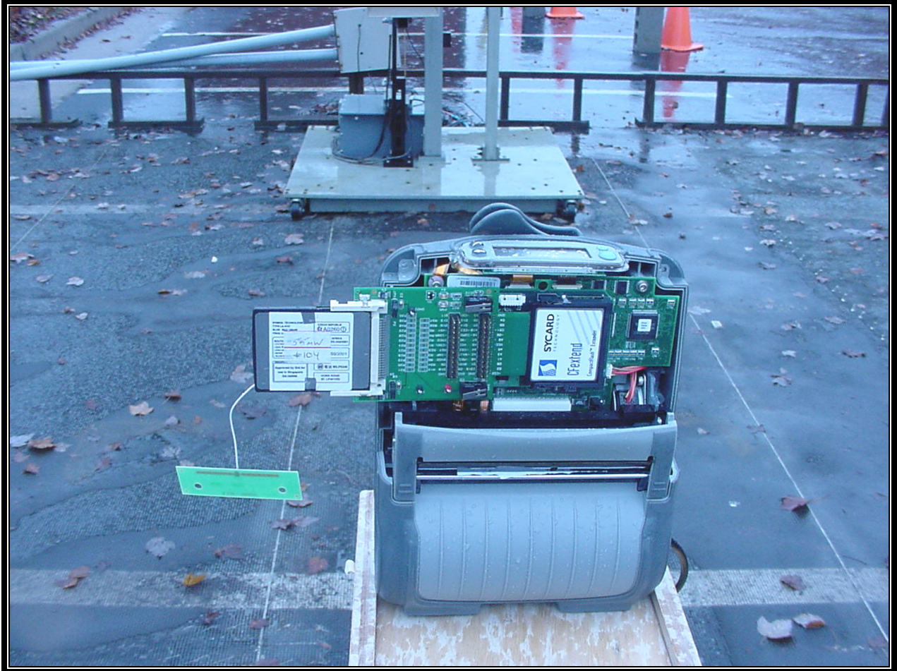
PHOTOGRAPH 1: RADIATED EMISSION FRONT VIEW USING CQ16688 ANTENNA
