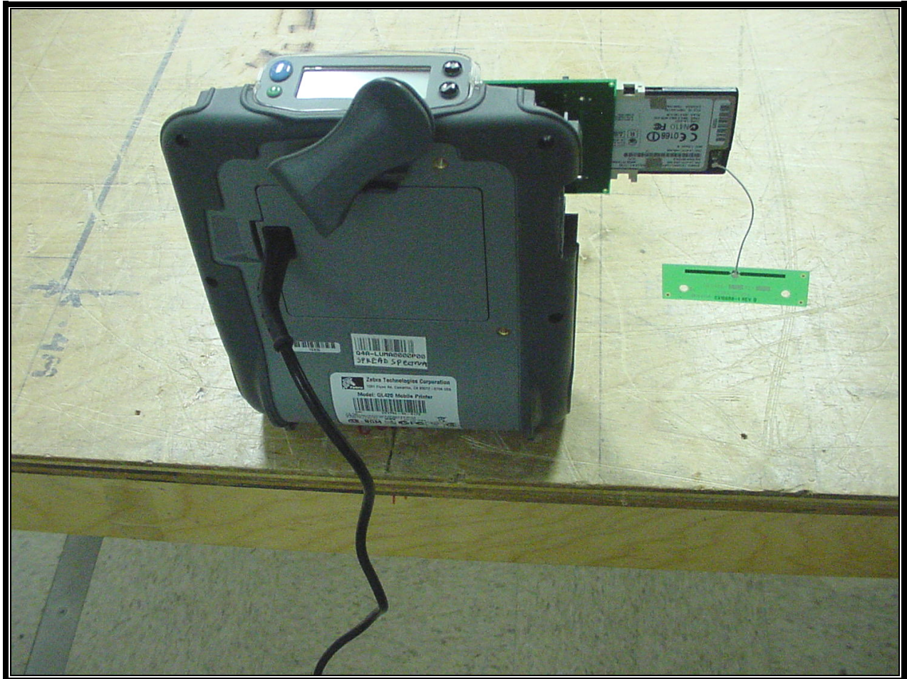
PHOTOGRAPH 6: CONDUCTED EMISSION REAR VIEW USING CQ16688 ANTENNA
