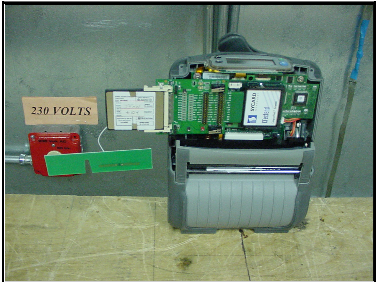
PHOTOGRAPH 7: CONDUCTED EMISSION FRONT VIEW USING CQ17110 ANTENNA
