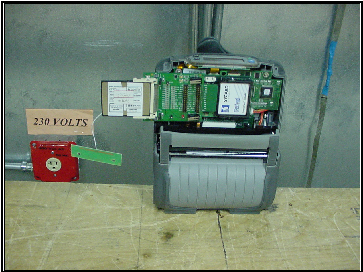
PHOTOGRAPH 5: CONDUCTED EMISSION FRONT VIEW USING CQ16688 ANTENNA
