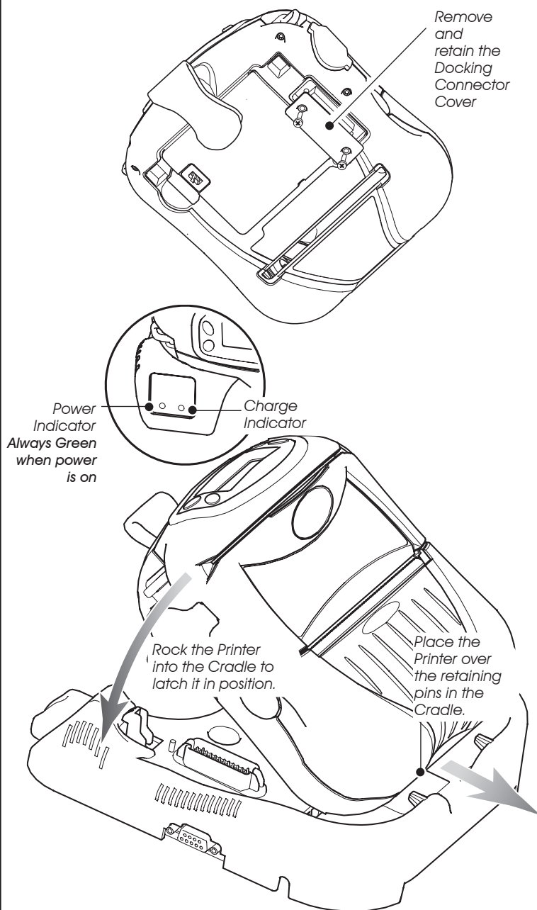
Figure 20: Installing the Printer into the Cradle
