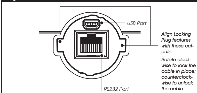
Figure 11: Communications Port
