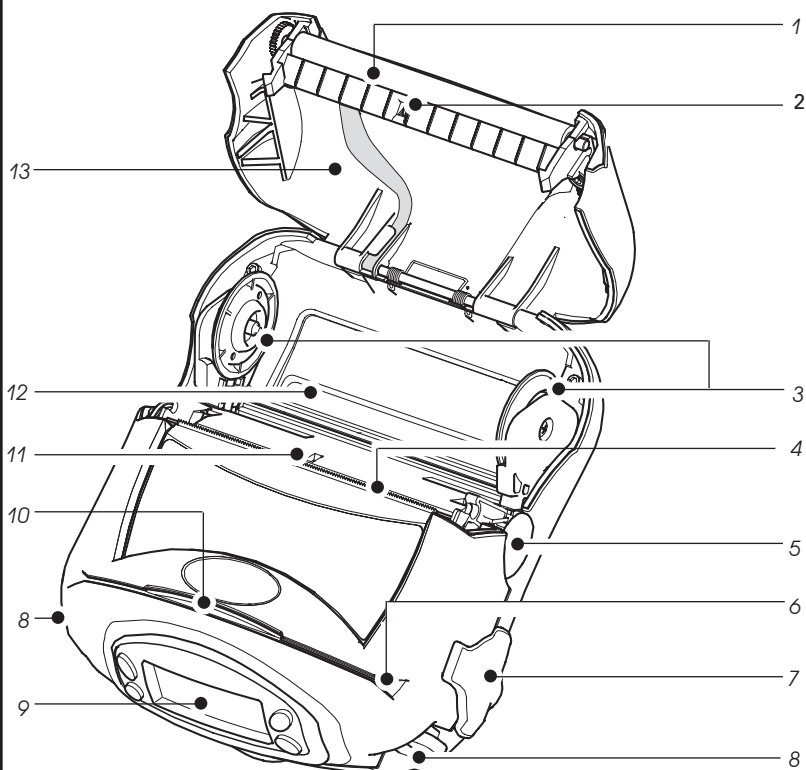
Figure 1: RW 420 Overview
