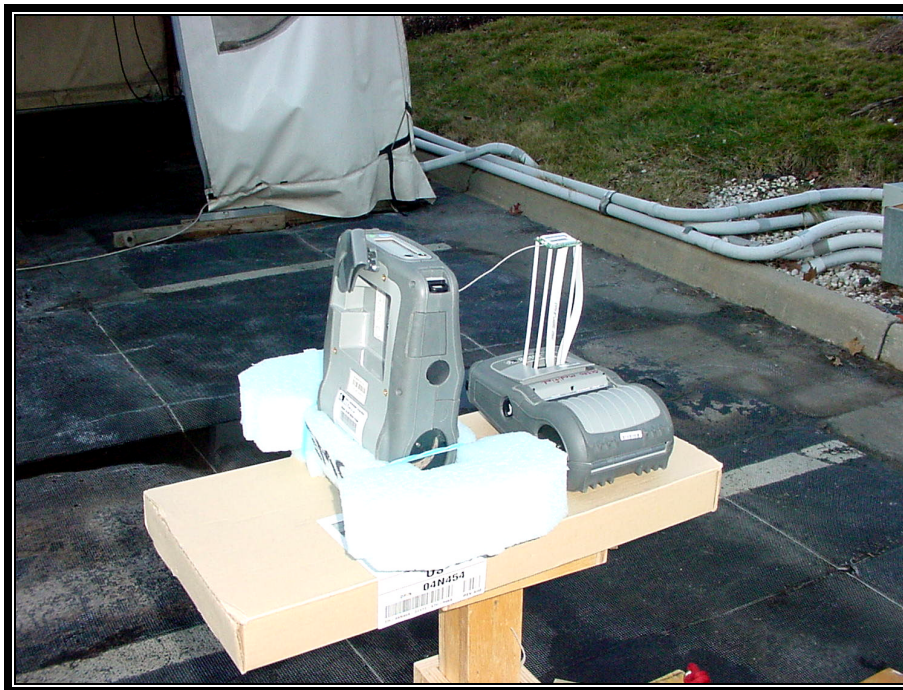
PHOTOGRAPH 6: RADIATED EMISSIONS REAR VIEW USING QL-420 CQ17383-1 ANTENNA
