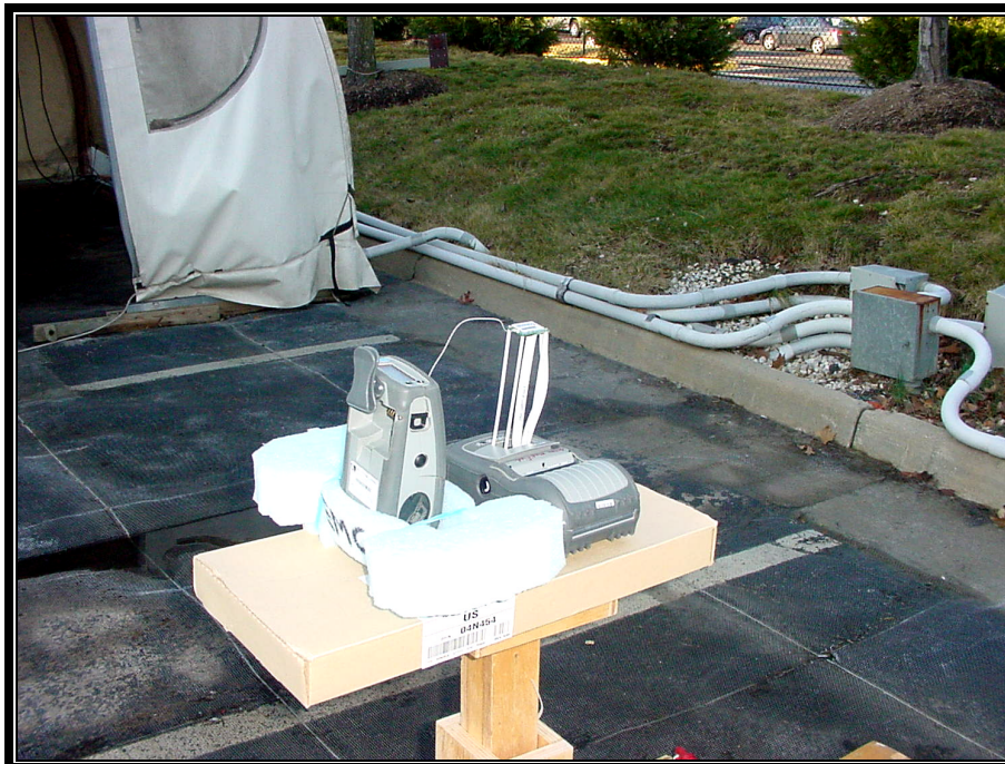
PHOTOGRAPH 4: RADIATED EMISSIONS REAR VIEW USING QL-220 CQ17383-1 ANTENNA
