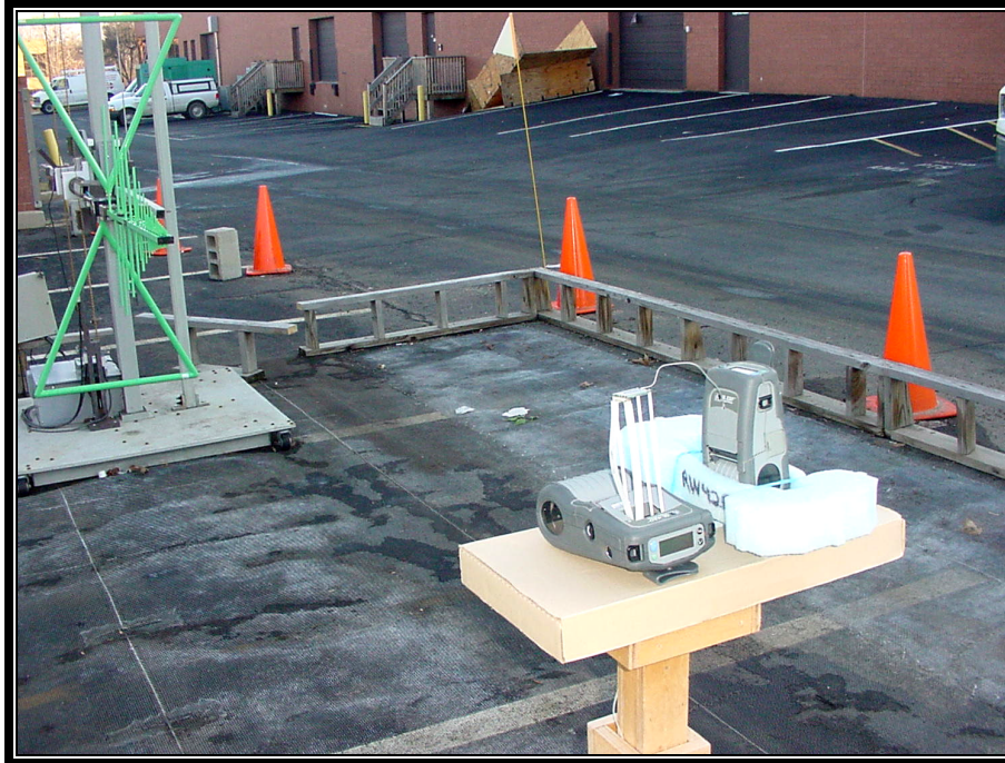
PHOTOGRAPH 3: RADIATED EMISSIONS FRONT VIEW USING QL-220 CQ17383-1 ANTENNA
