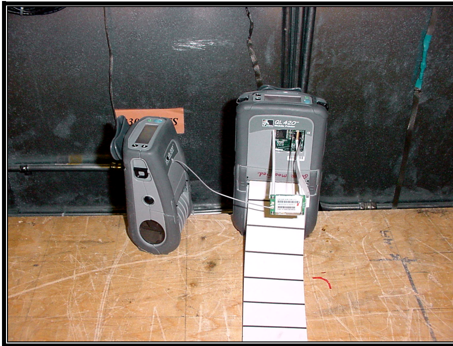
PHOTOGRAPH 9: CONDUCTED EMISSIONS FRONT VIEW USING QL-220 CQ17383-1 ANTENNA
