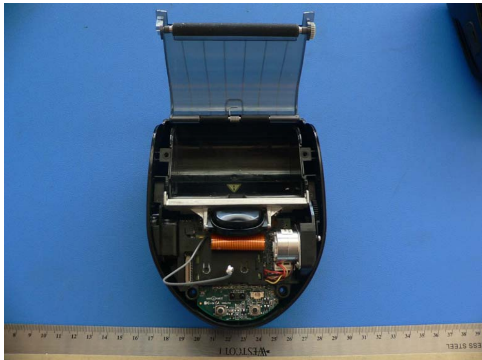
Host Chassis off View
