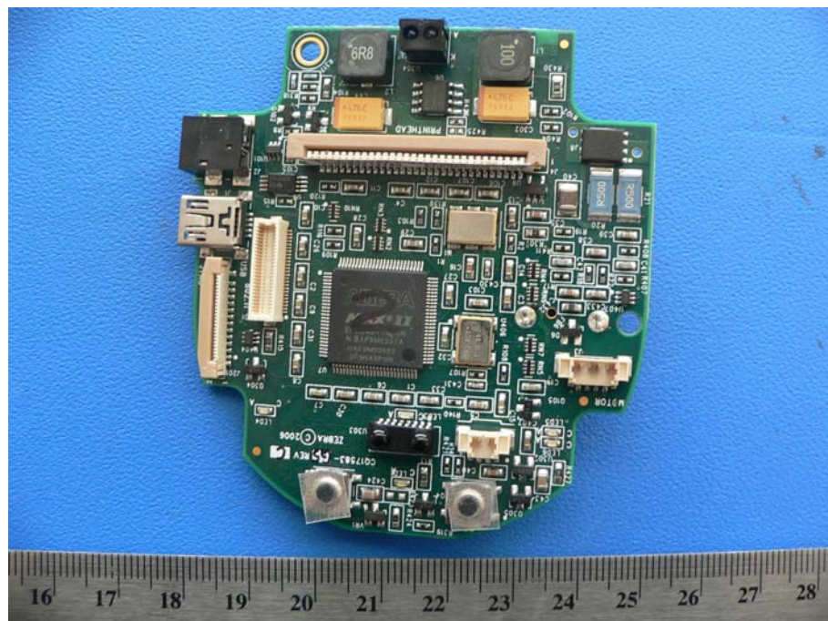
Host PCB Component Side View
