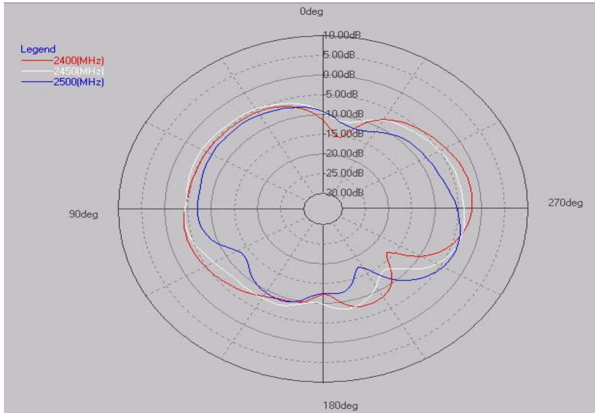
RW220 ZLAN11G antenna (CQ18317) - X-Z Plane
