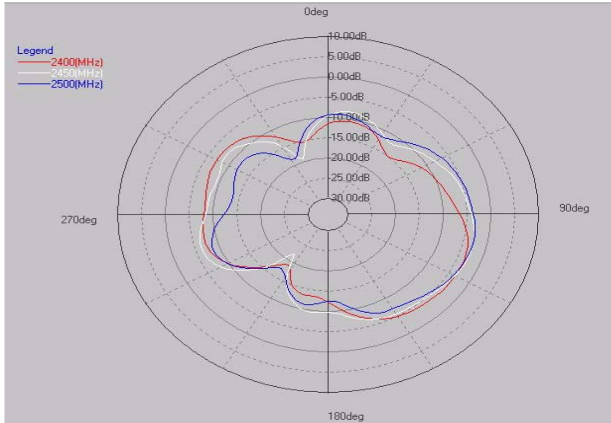
RW220 ZLAN11G antenna (CQ18317) - Y-Z Plane
