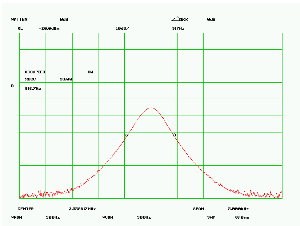
Plots: 13.56 MHz
