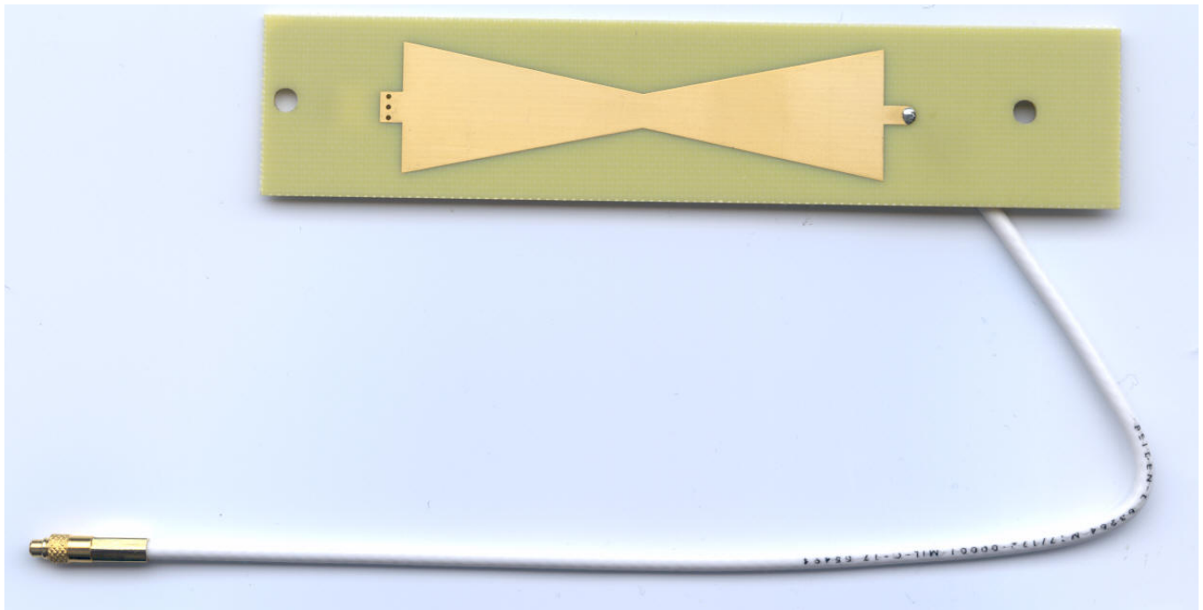
19630-099 CONDUCTOR SIDE
