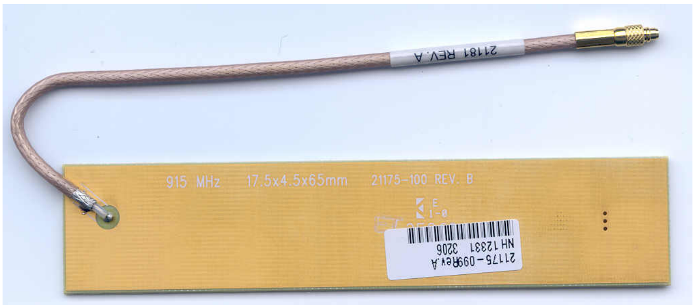
21175-099 GROUND PLANE SIDE
