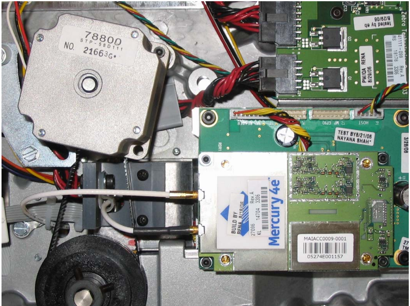
RA400 DUAL COUPLER IN PRINTER
