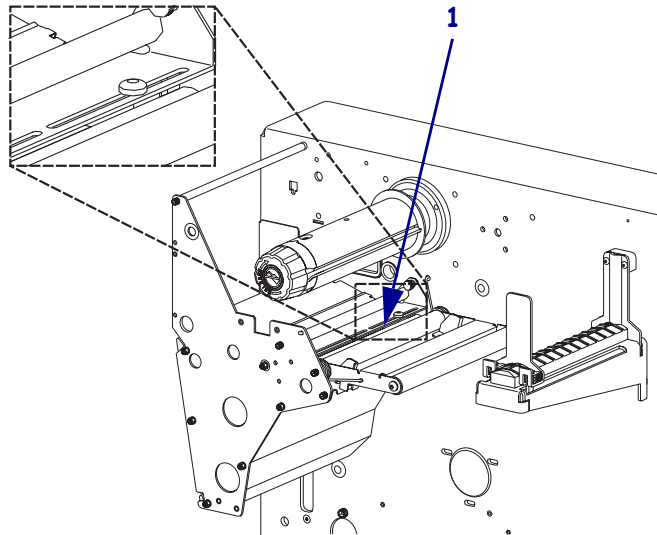
Figure 42 • Upper Media Sensor
