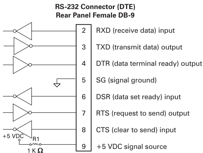
Figure 32 • RS-232 Connections
