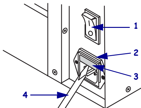
Figure 45 • AC Power Entry Module
