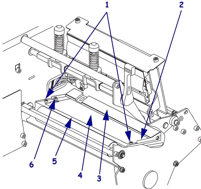
Figure 44 • Snap Plate
