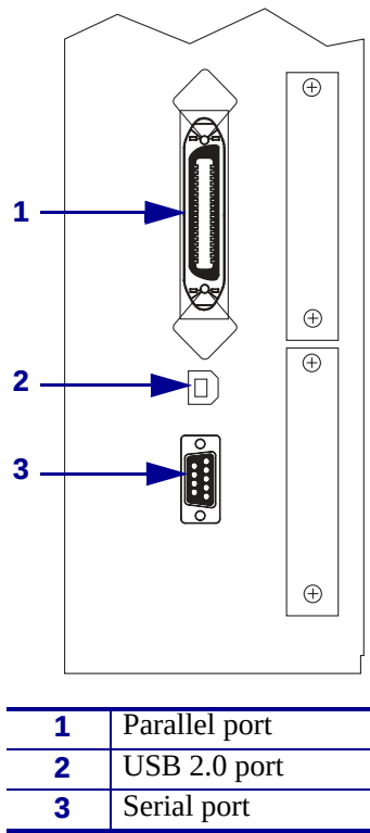
Figure 8 • Communication Interfaces
