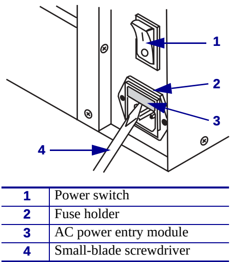
Figure 49 • AC Power Entry Module
