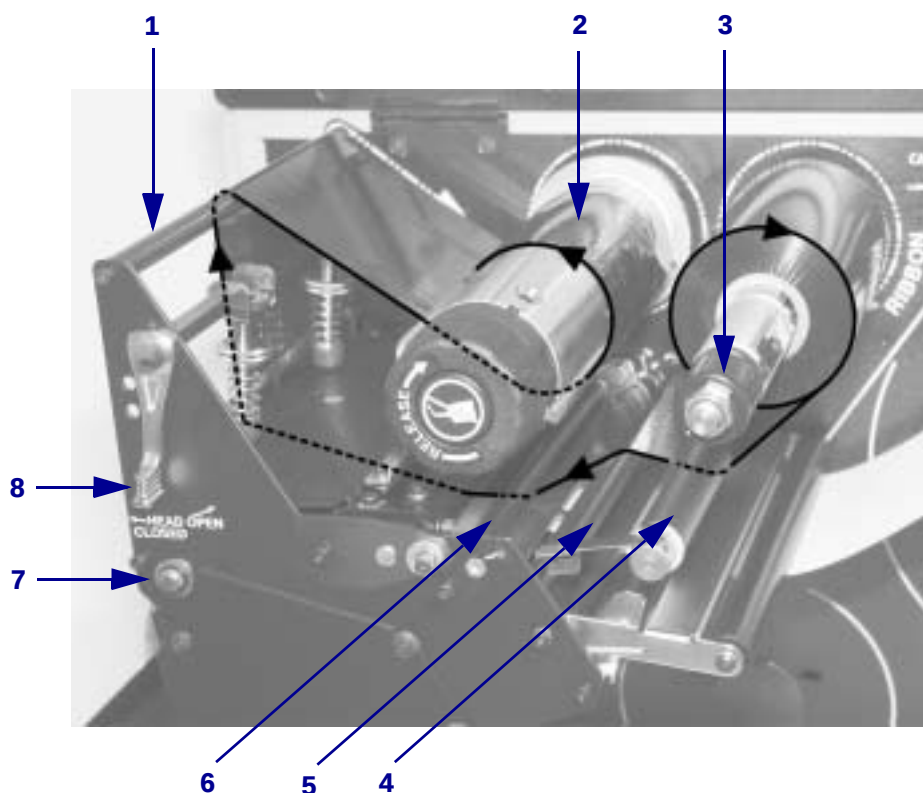
Figure 18 • Ribbon Path
