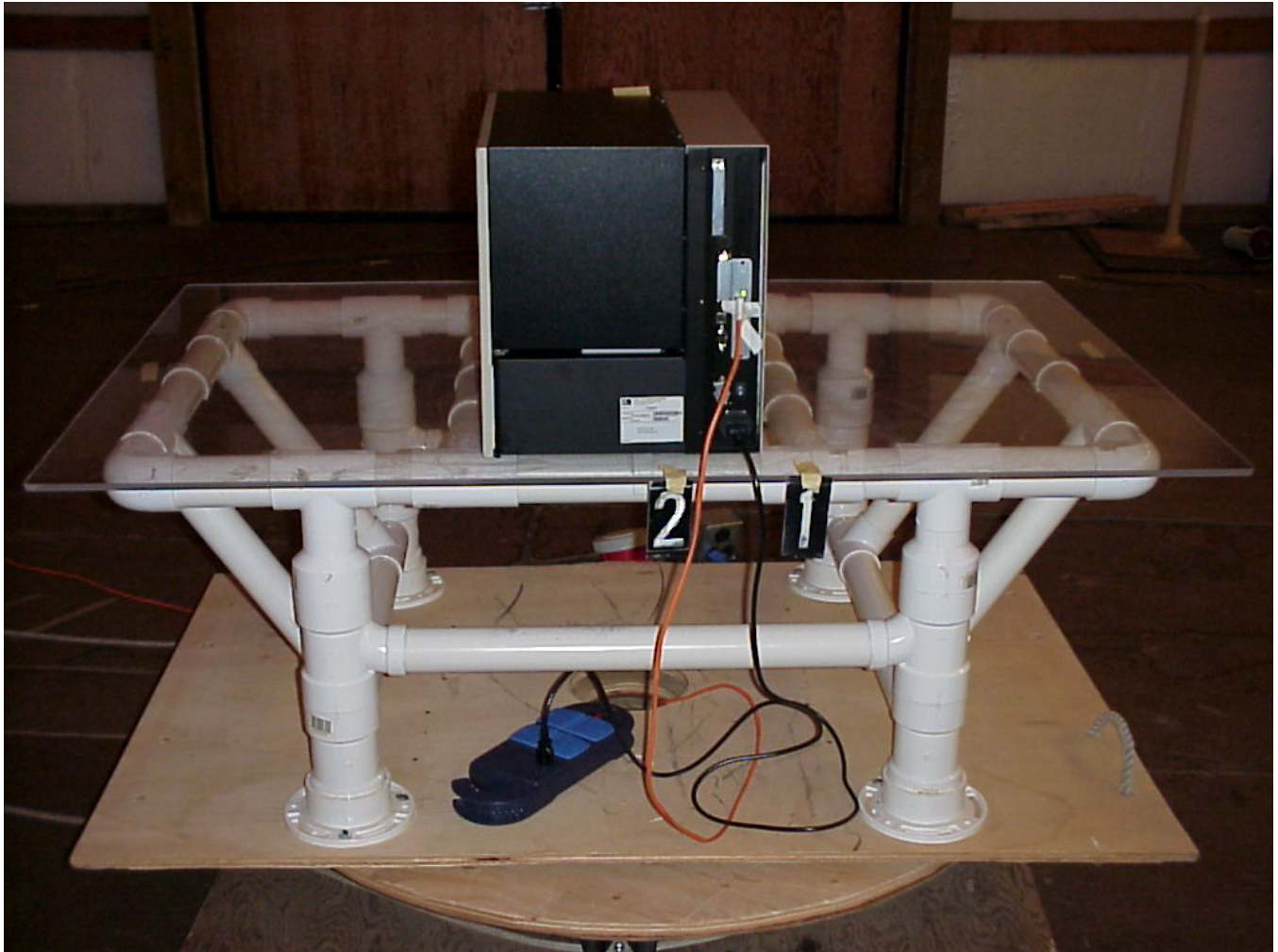
Radiated Emissions (Rear View)
