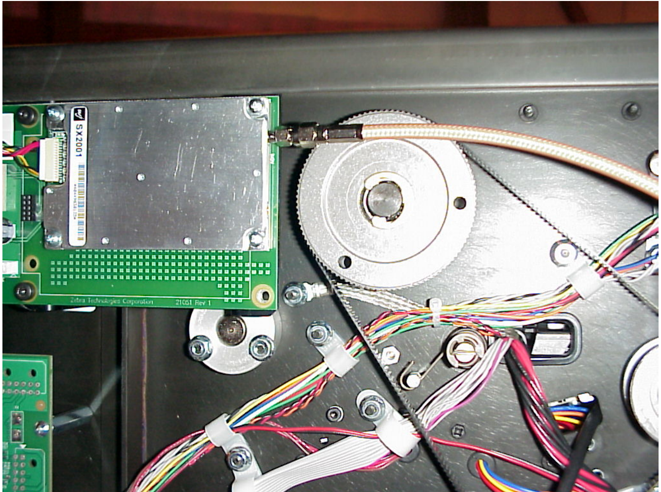
Antenna Direct Connect
