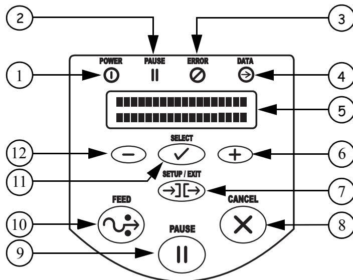
Figure 12 • Front Panel
