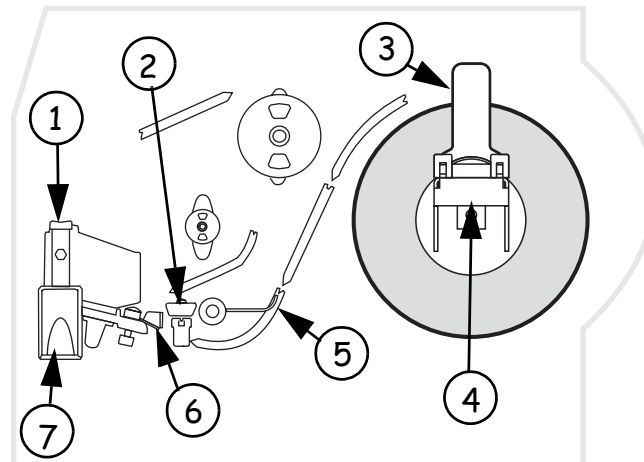
Figure 3 • Media Compartment
