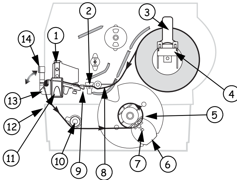
Figure 19 • Rewind Mode
