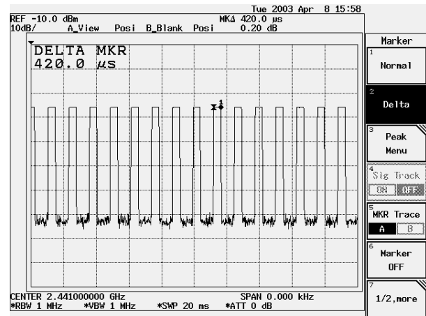
2441MHz
