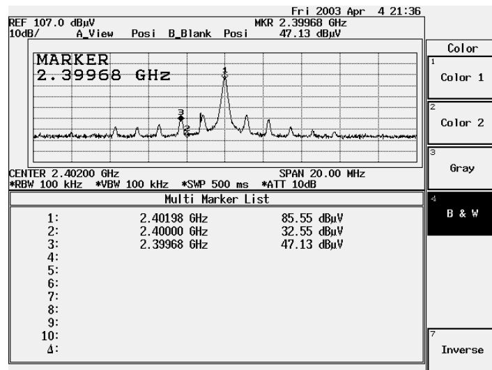
Figure Channel 00: (Vertical)
