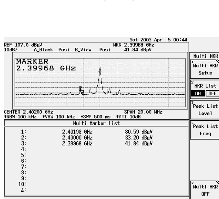
Figure Channel 00: (Vertical)
