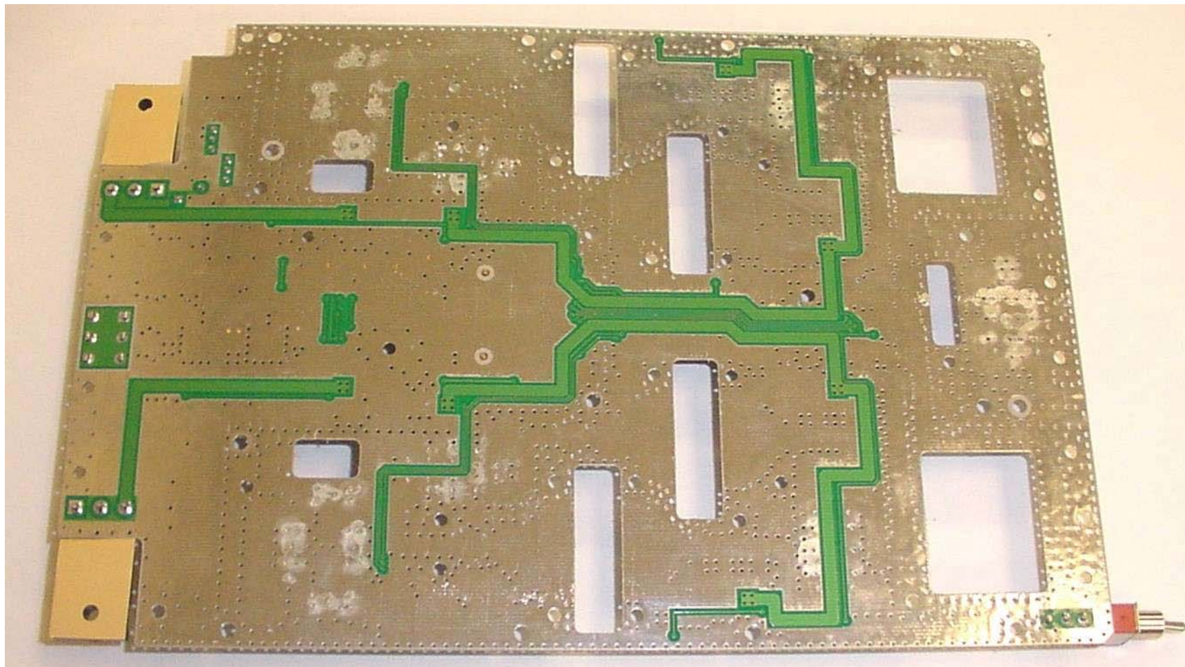
BOTTOM SIDE OF AMPLIFER BOARD
