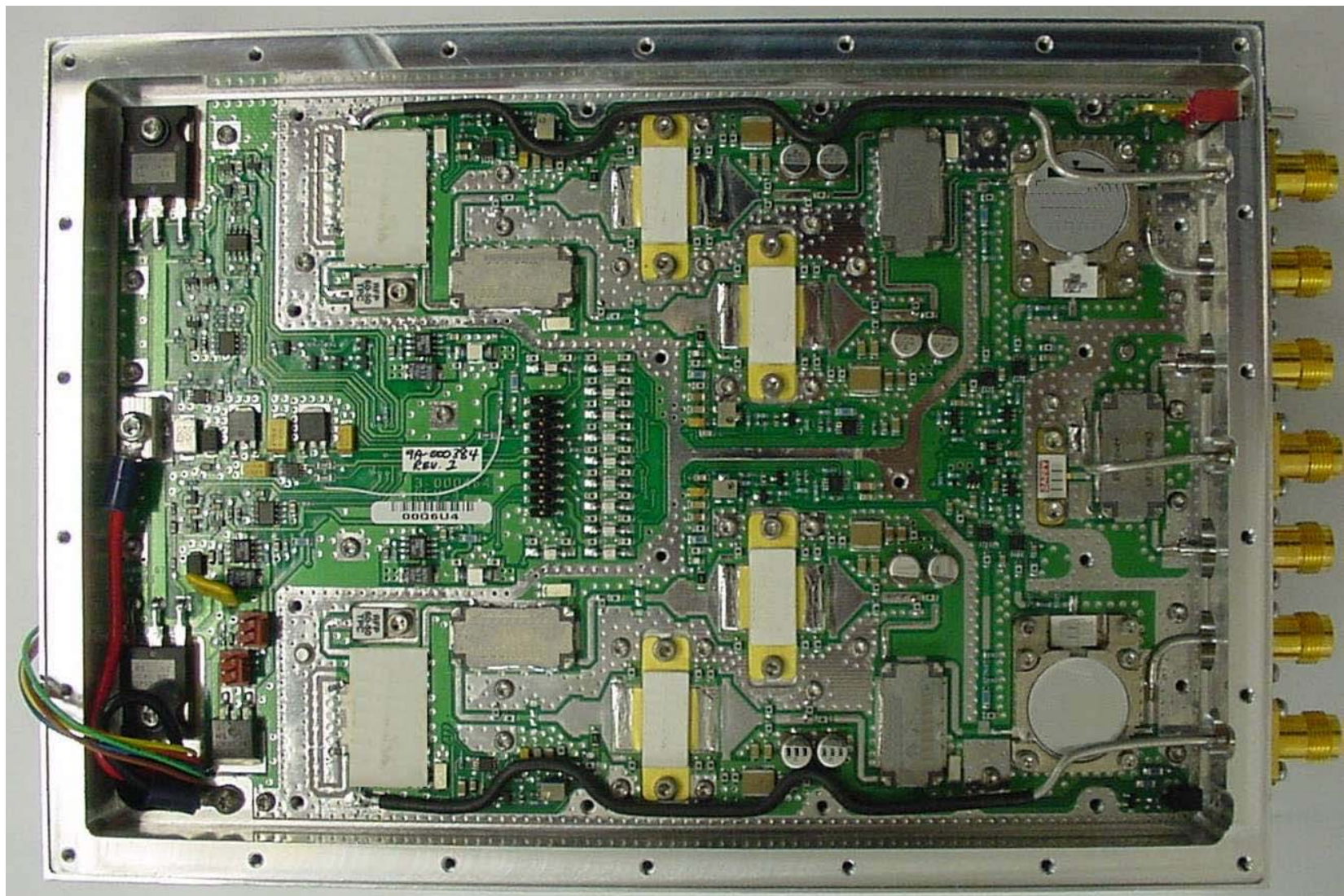
TOP SIDE OF AMPLIFIER BOARD
