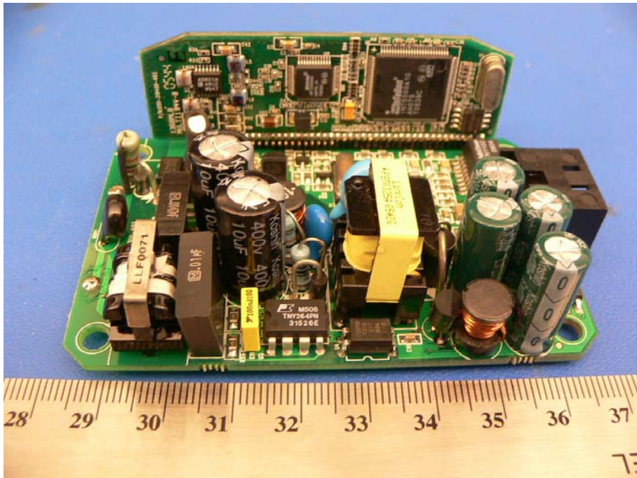
Adapter Component View
