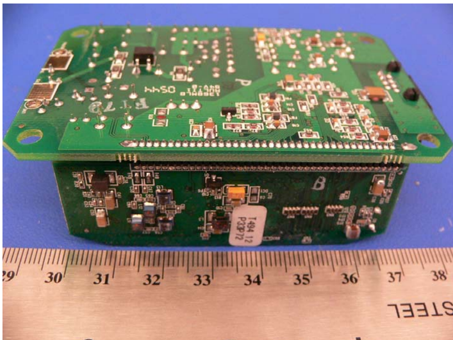
Adapter Solder View
