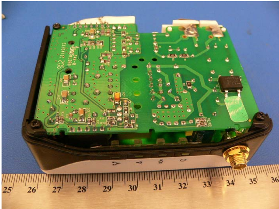
EUT-PCB Component View (1)
