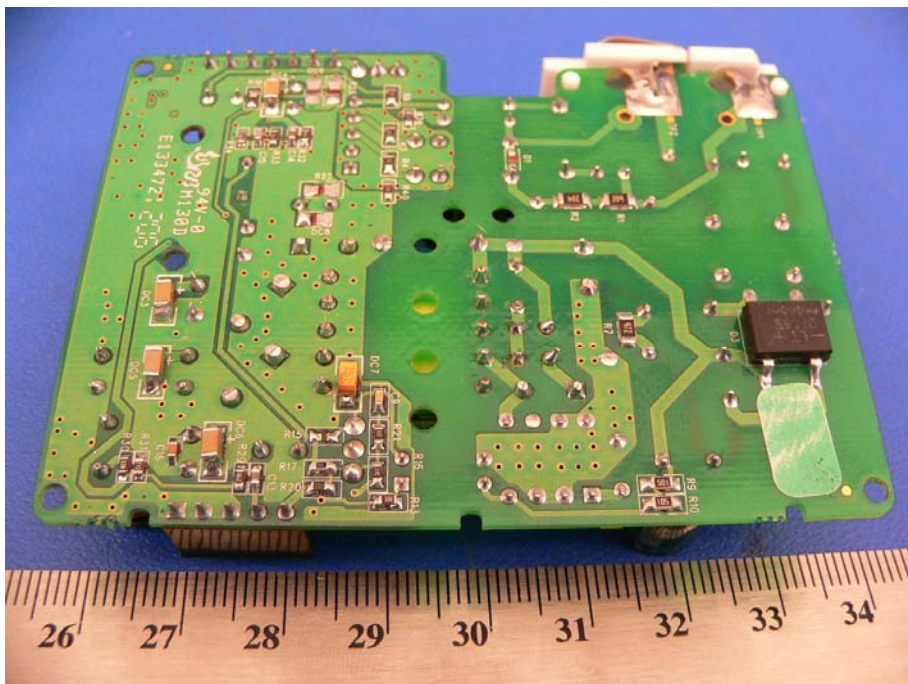
EUT-PCB Solder View (1)
