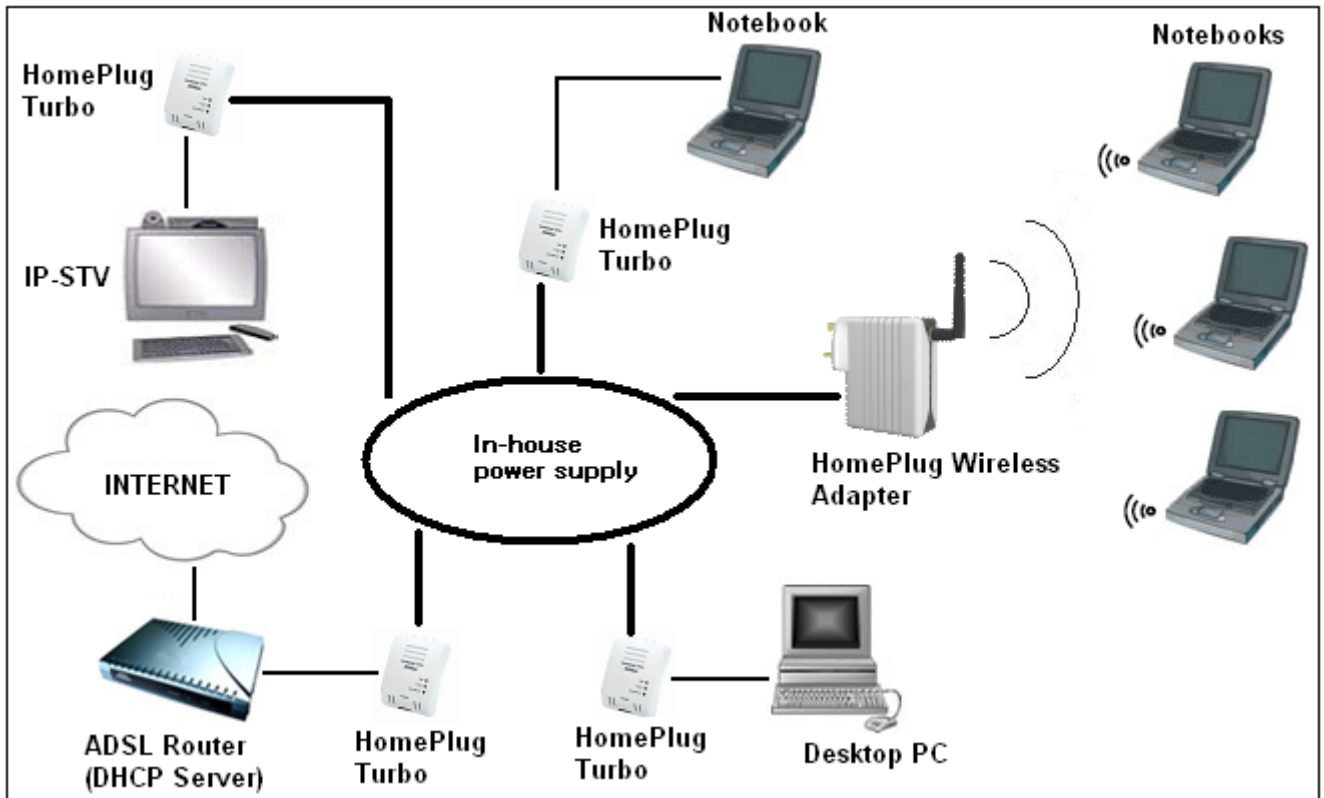
Figure 1 : User Connection Diagram
