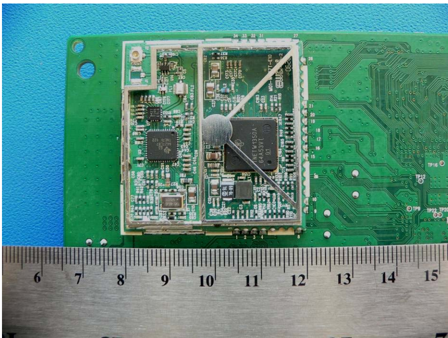
EUT - PCB Bottom View Close Up
