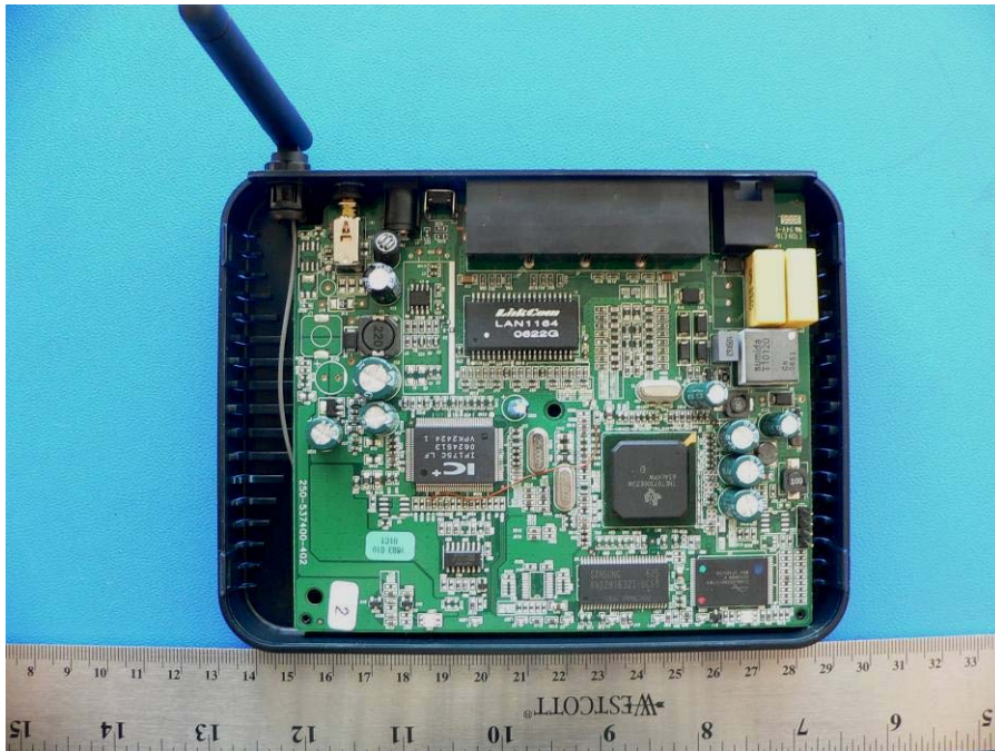
EUT- Cover off Front
