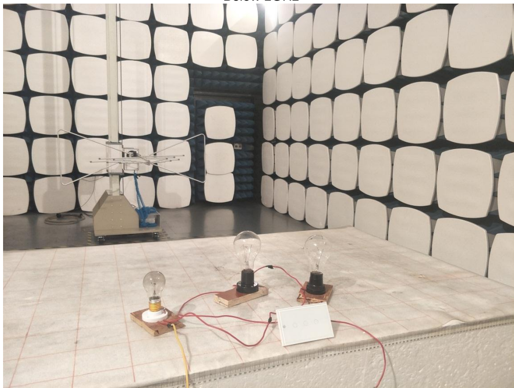
KSW5-223-ZB Radiated Emission Below 1GHz
