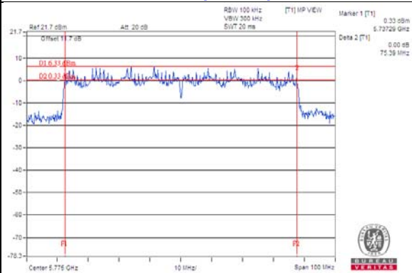
802.11ac (80MHz)_CH155
