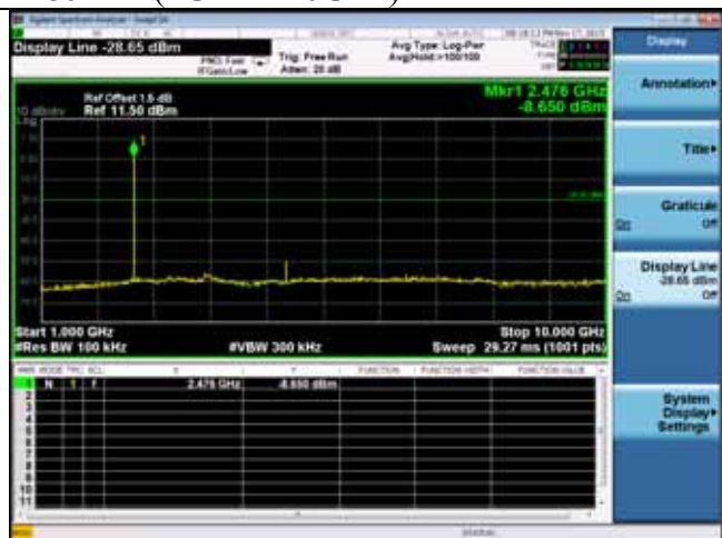
2480MHz(1GHz – 10GHz)
