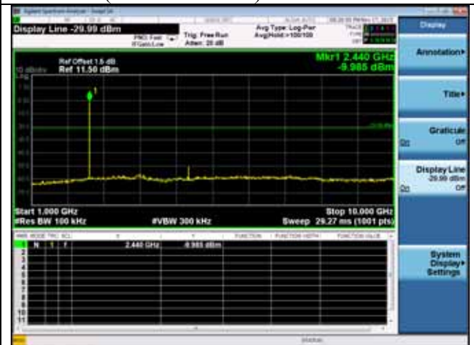
2441MHz(1GHz – 10GHz)
