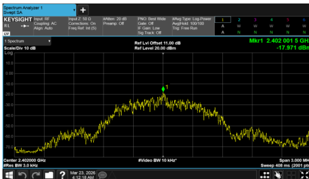
Modulation Type: GFSK(1Mbps), CH00
