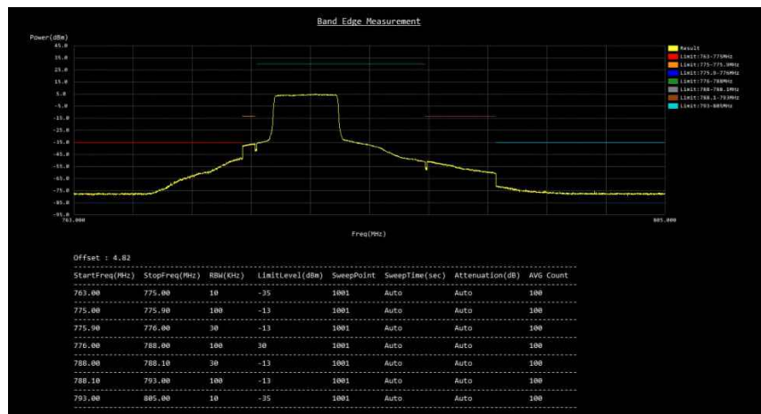
# FCC / Band : B13 / Channel : 23205 ( 779.5MHz ) Band Edge Measurement
