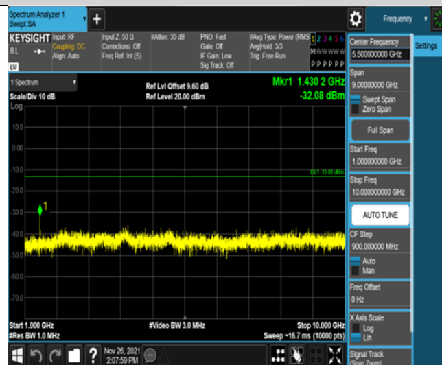
Band12-3MHz-QPSK-23165-15RB#0-Range2:1000~10000MHz
