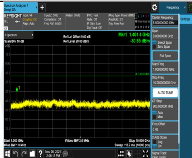
Band12-3MHz-QPSK-23025-15RB#0-Range2:1000~10000MHz
