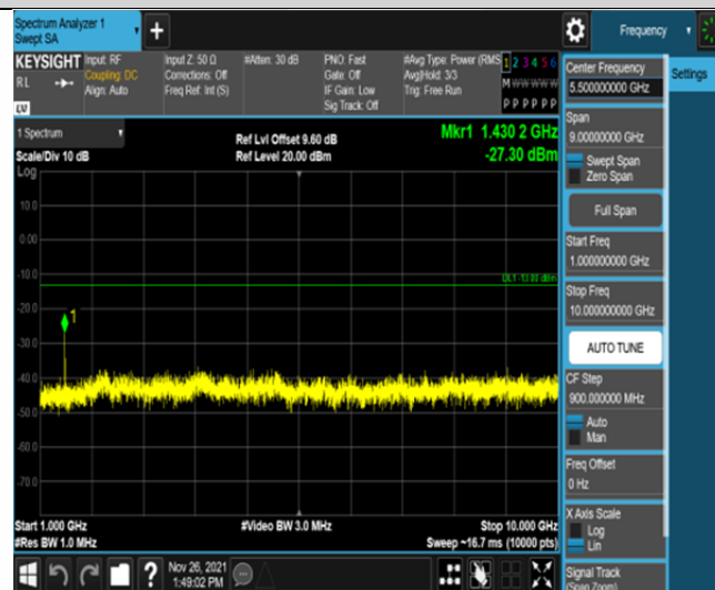
Band12-1.4MHz-16QAM-23173-6RB#0-Range2:1000~10000MHz
