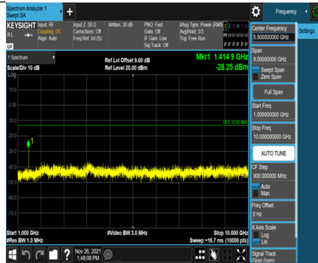
Band12-1.4MHz-16QAM-23095-6RB#0-Range2:1000~10000MHz
