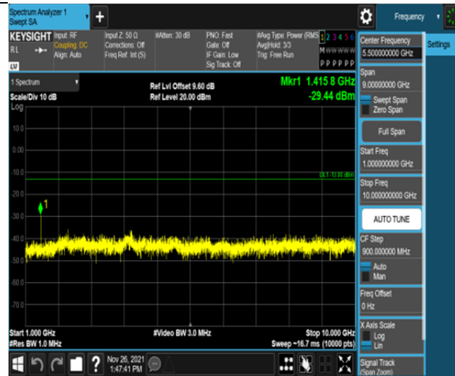
Band12-1.4MHz-QPSK-23095-6RB#0-Range2:1000~10000MHz
