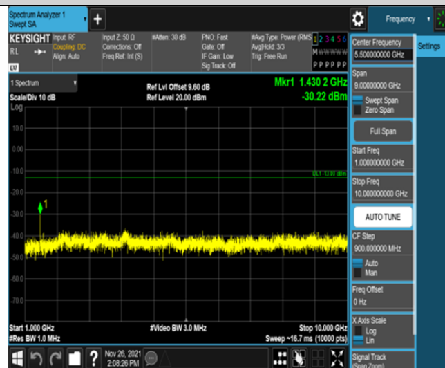
Band12-3MHz-16QAM-23165-15RB#0-Range2:1000~10000MHz
