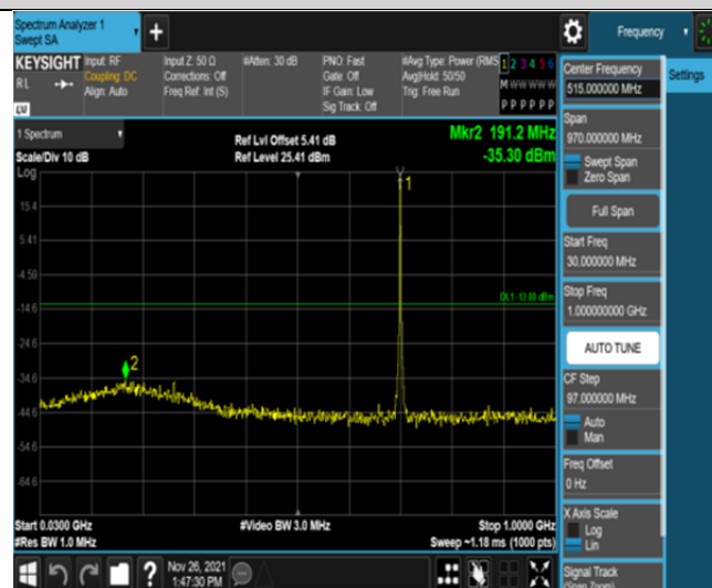
Band12-1.4MHz-QPSK-23095-6RB#0-Range1:30~1000MHz
