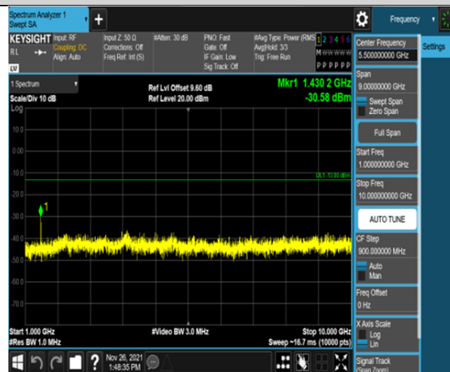
Band12-1.4MHz-QPSK-23173-6RB#0-Range2:1000~10000MHz
