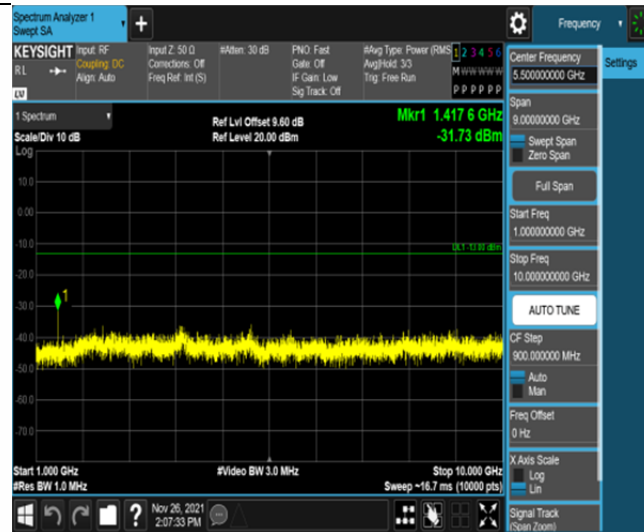
Band12-3MHz-16QAM-23095-15RB#0-Range2:1000~10000MHz
