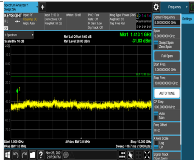
Band12-3MHz-QPSK-23095-15RB#0-Range2:1000~10000MHz
