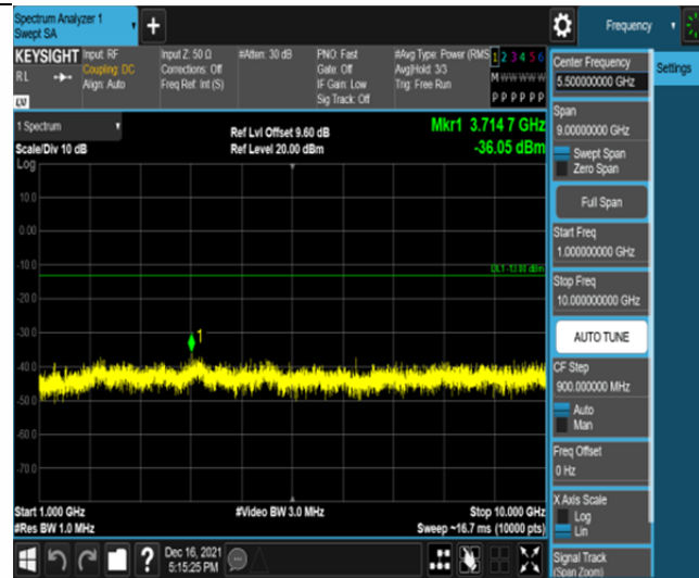
Band13-5MHz-16QAM-23205-25RB#0-Range2:1000~10000MHz
