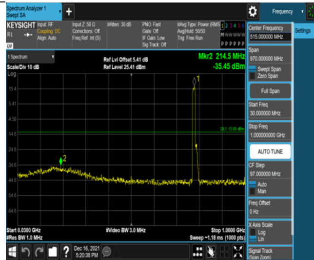
Band13-5MHz-16QAM-23205-25RB#0-Range1:30~1000MHz
