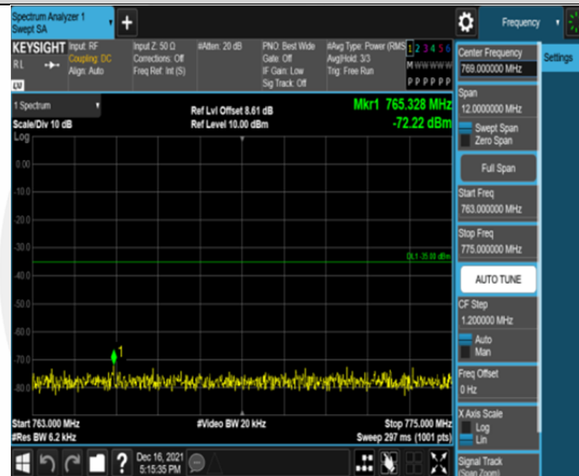
Band13-5MHz-16QAM-23205-25RB#0-Range3:763~775MHz
