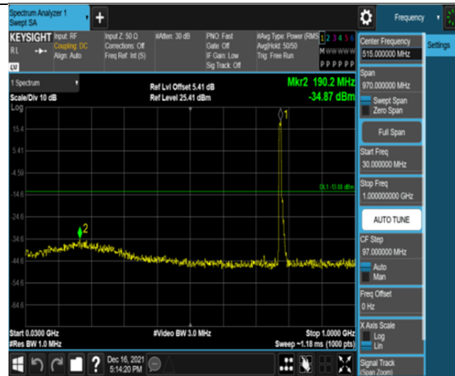
Band13-5MHz-QPSK-23205-25RB#0-Range1:30~1000MHz
