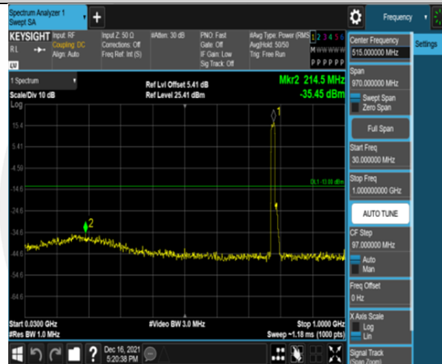
Band13-5MHz-QPSK-23255-25RB#0-Range1:30~1000MHz
