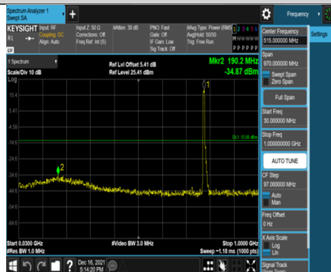
Band13-5MHz-16QAM-23230-25RB#0-Range1:30~1000MHz
