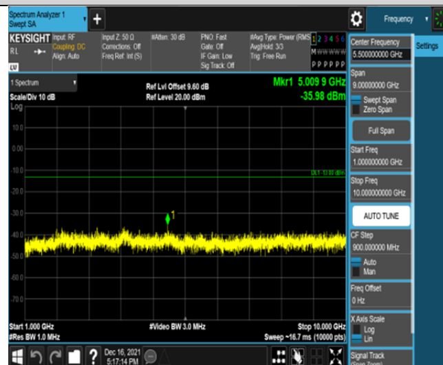
Band13-5MHz-16QAM-23230-25RB#0-Range2:1000~10000MHz
