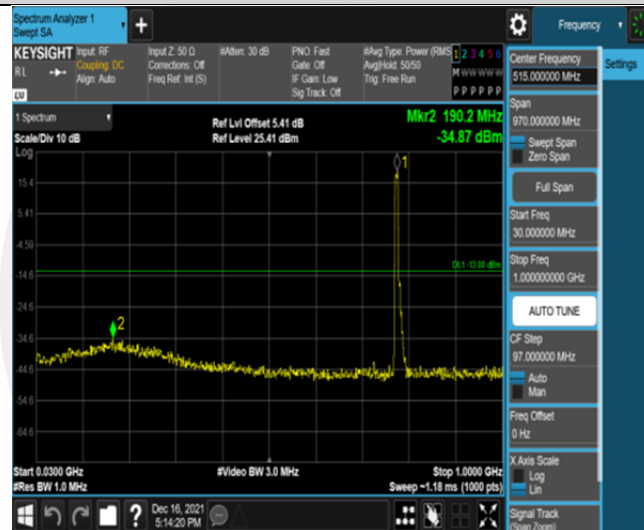
Band13-5MHz-16QAM-23255-25RB#0-Range1:30~1000MHz
