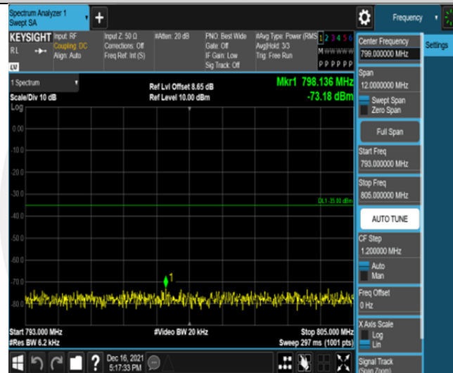
Band13-5MHz-16QAM-23230-25RB#0-Range4:793~805MHz
