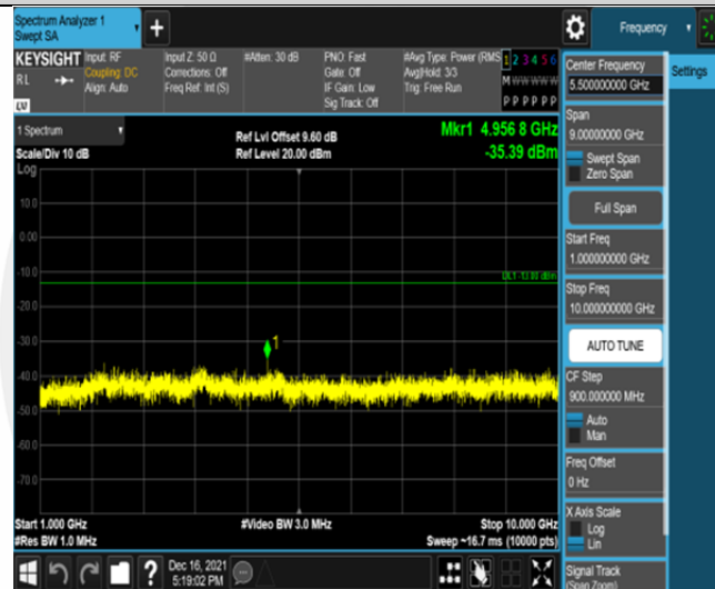
Band13-5MHz-16QAM-23255-25RB#0-Range2:1000~10000MHz
