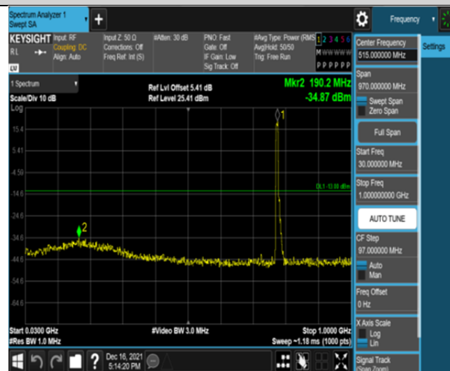
Band13-10MHz-16QAM-23230-50RB#0-Range1:30~1000MHz
