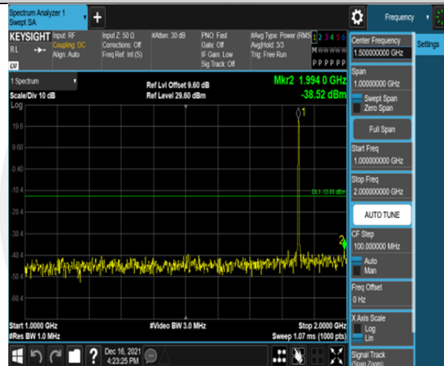
Band2-1.4MHz-16QAM-18607-6RB#0-Range2:1000~2000MHz
