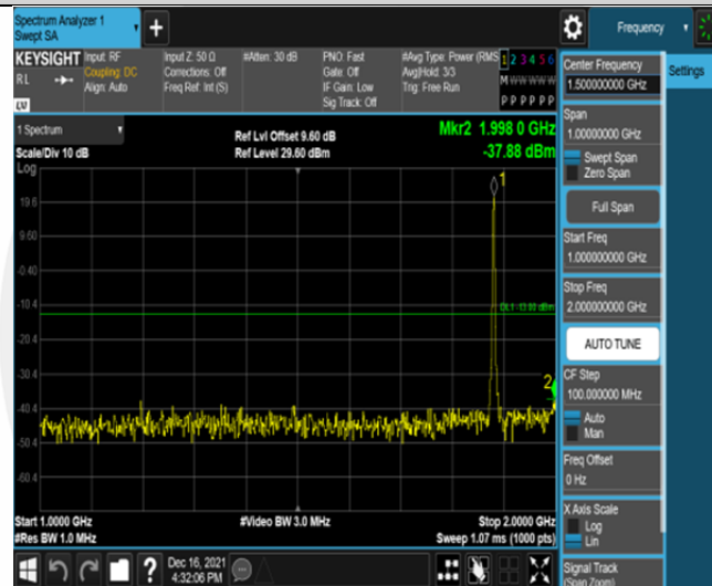
Band2-3MHz-16QAM-18900-15RB#0-Range2:1000~2000MHz
