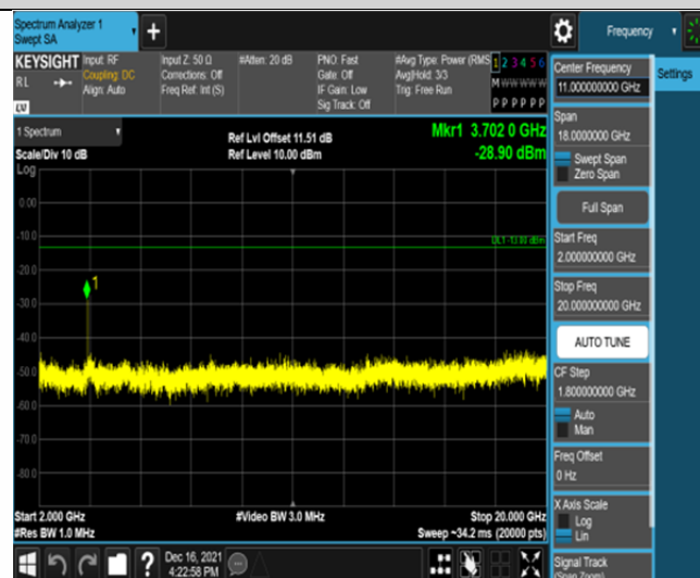
Band2-1.4MHz-QPSK-18607-6RB#0-Range3:2000~20000MHz
