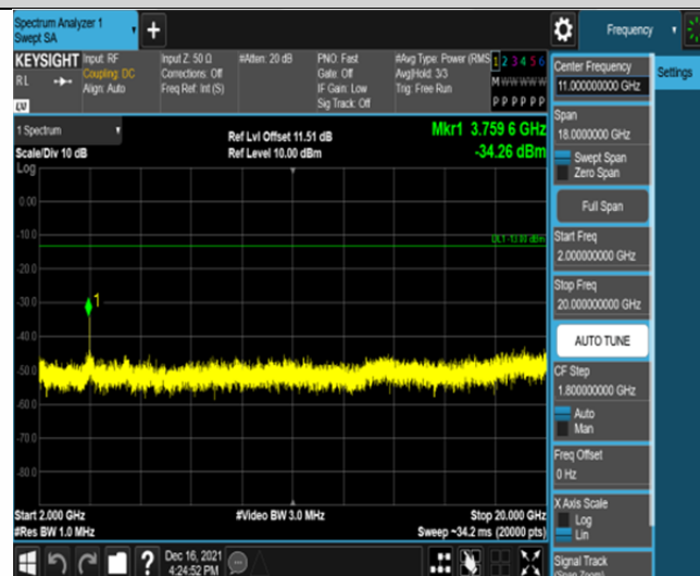
Band2-1.4MHz-16QAM-18900-6RB#0-Range3:2000~20000MHz
