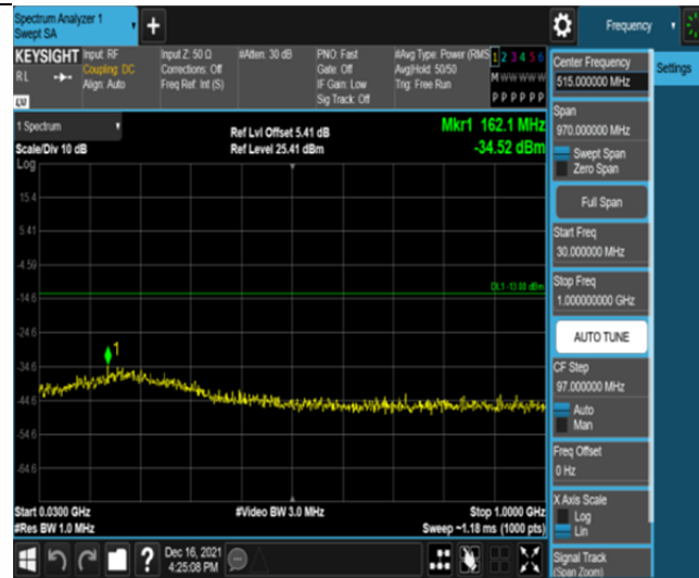
Band2-1.4MHz-QPSK-19193-6RB#0-Range1:30~1000MHz
