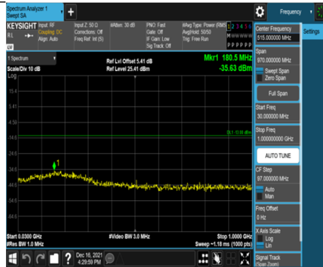
Band2-3MHz-QPSK-18615-15RB#0-Range1:30~1000MHz
