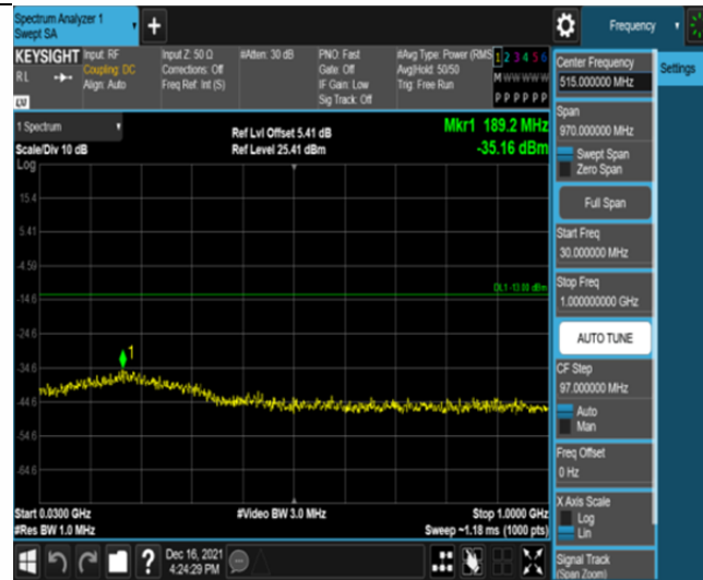
Band2-1.4MHz-16QAM-18900-6RB#0-Range1:30~1000MHz
