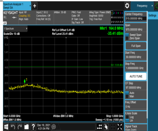
Band2-3MHz-16QAM-18900-15RB#0-Range1:30~1000MHz
