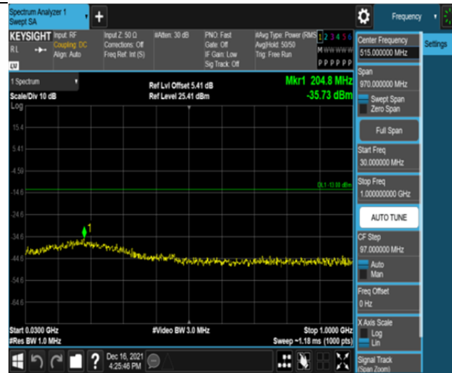
Band2-1.4MHz-16QAM-19193-6RB#0-Range1:30~1000MHz
