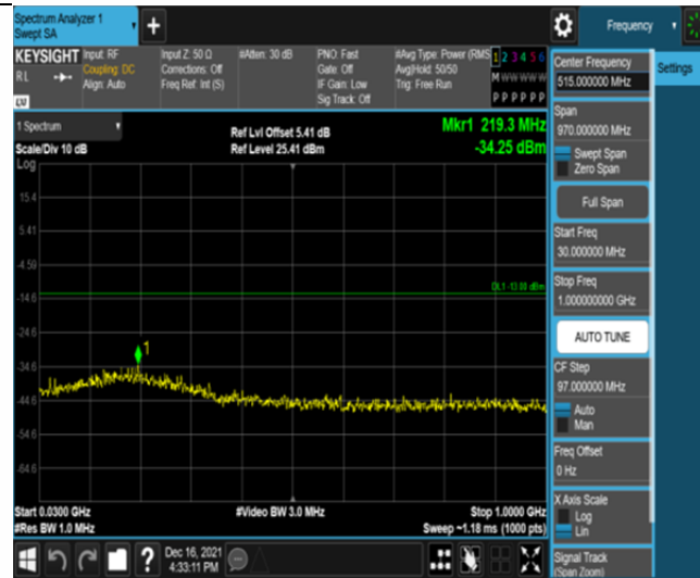
Band2-3MHz-16QAM-19185-15RB#0-Range1:30~1000MHz
