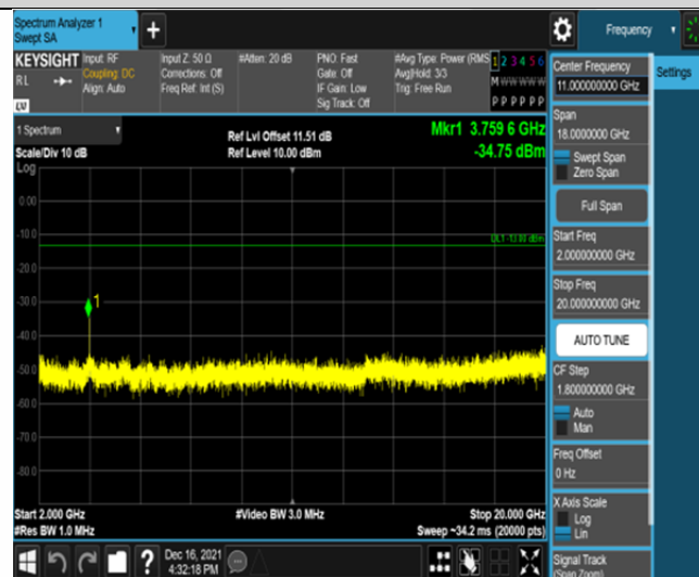
Band2-3MHz-16QAM-18900-15RB#0-Range3:2000~20000MHz
