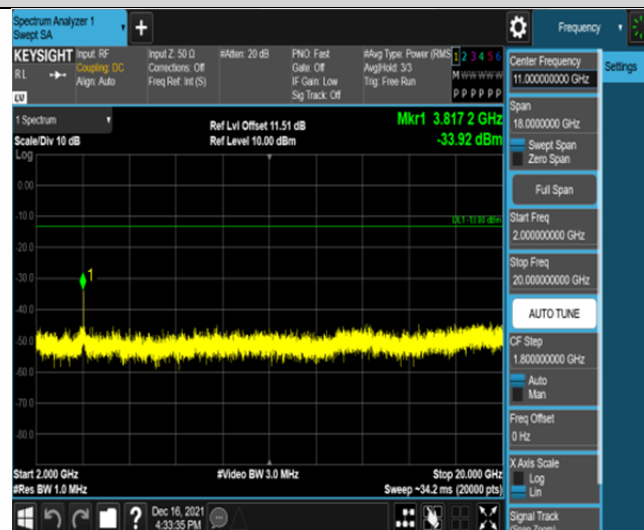
Band2-3MHz-16QAM-19185-15RB#0-Range3:2000~20000MHz
