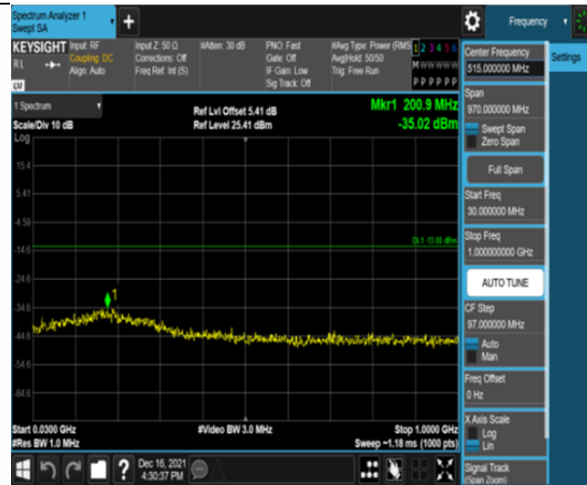
Band2-3MHz-16QAM-18615-15RB#0-Range1:30~1000MHz
