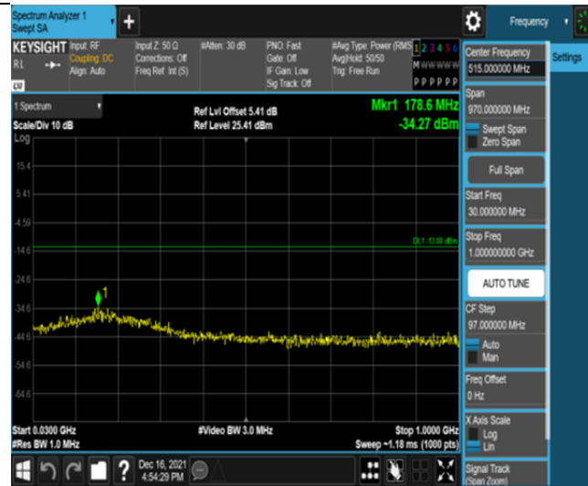
Band2-15MHz-QPSK-18900-75RB#0-Range1:30~1000MHz
