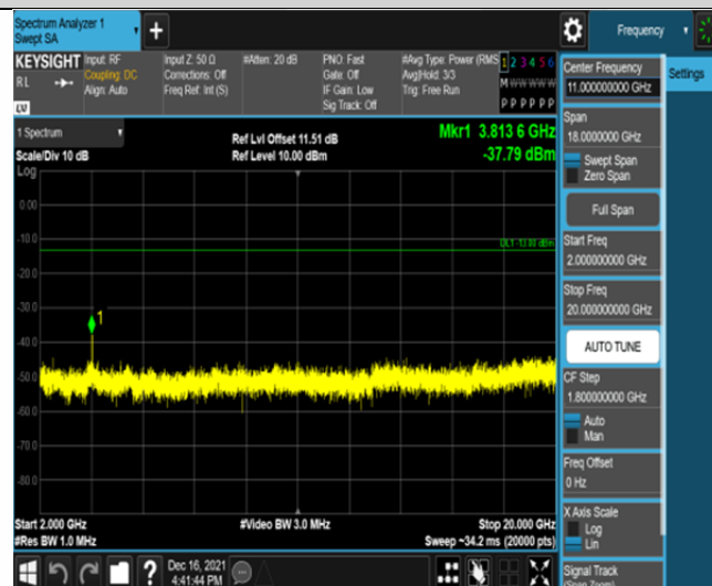
Band2-5MHz-16QAM-19175-25RB#0-Range3:2000~20000MHz
