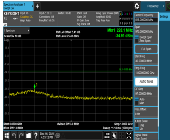
Band2-15MHz-QPSK-18675-75RB#0-Range1:30~1000MHz
