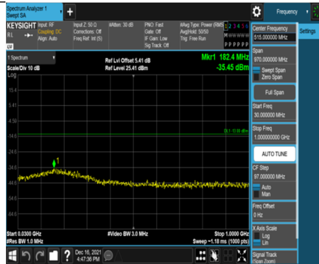
Band2-10MHz-16QAM-18900-50RB#0-Range1:30~1000MHz
