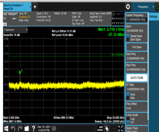
Band2-10MHz-QPSK-18650-50RB#0-Range3:2000~20000MHz
