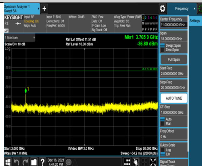
Band2-10MHz-QPSK-18900-50RB#0-Range3:2000~20000MHz
