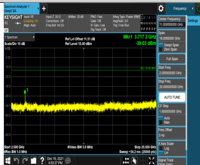
Band2-15MHz-QPSK-18675-75RB#0-Range3:2000~20000MHz
