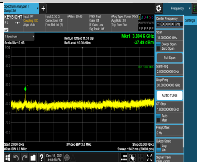
Band2-10MHz-QPSK-19150-50RB#0-Range3:2000~20000MHz
