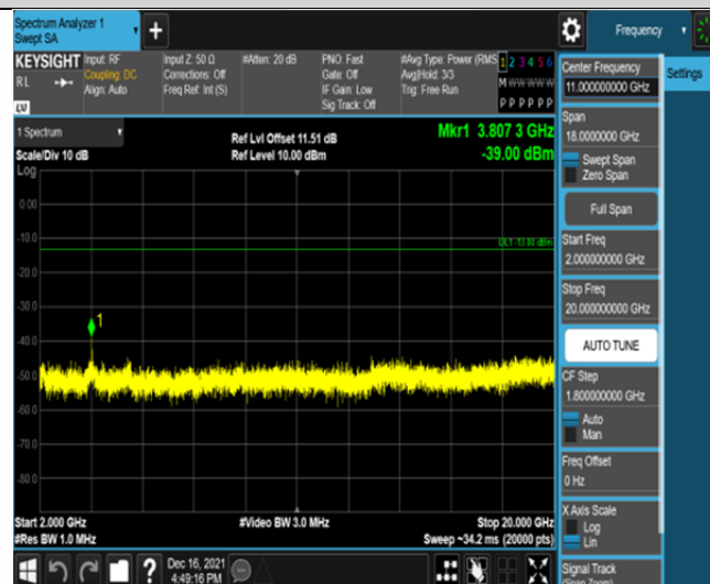
Band2-10MHz-16QAM-19150-50RB#0-Range3:2000~20000MHz
