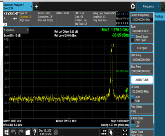
Band2-10MHz-16QAM-18650-50RB#0-Range2:1000~2000MHz
