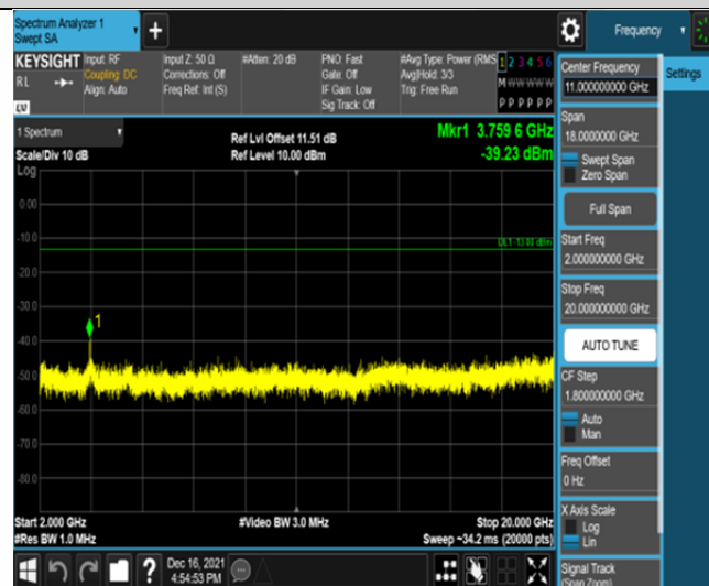
Band2-15MHz-QPSK-18900-75RB#0-Range3:2000~20000MHz
