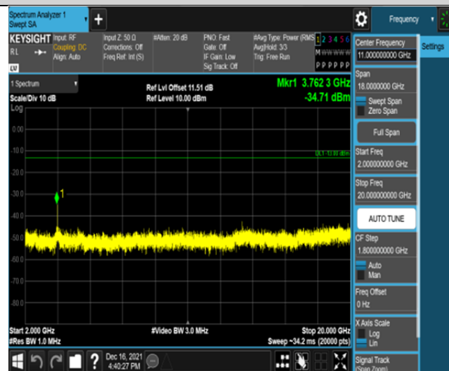
Band2-5MHz-16QAM-18900-25RB#0-Range3:2000~20000MHz
