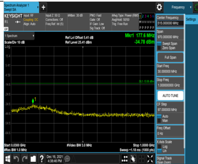
Band2-5MHz-16QAM-18625-25RB#0-Range1:30~1000MHz
