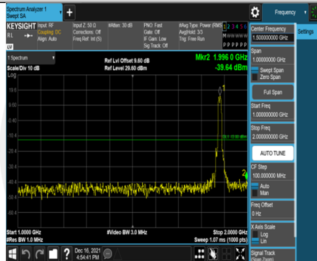
Band2-15MHz-QPSK-18900-75RB#0-Range2:1000~2000MHz
