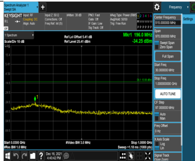
Band2-5MHz-QPSK-19175-25RB#0-Range1:30~1000MHz
