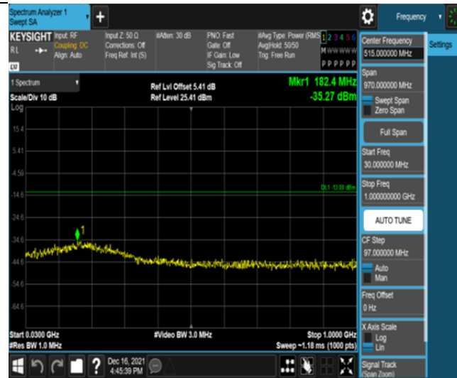
Band2-10MHz-QPSK-18650-50RB#0-Range1:30~1000MHz
