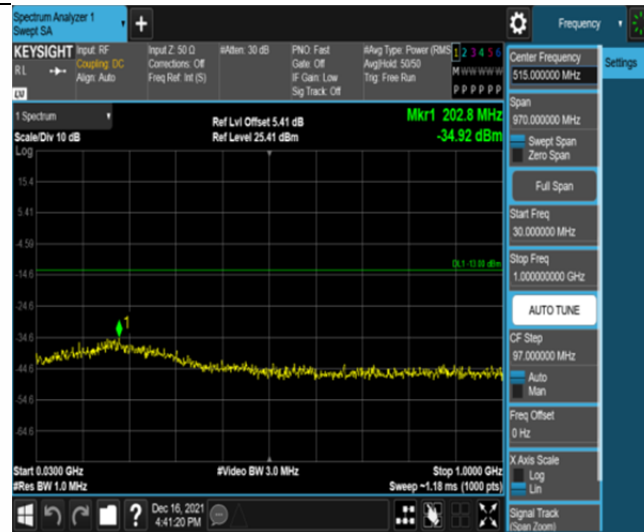
Band2-5MHz-16QAM-19175-25RB#0-Range1:30~1000MHz
