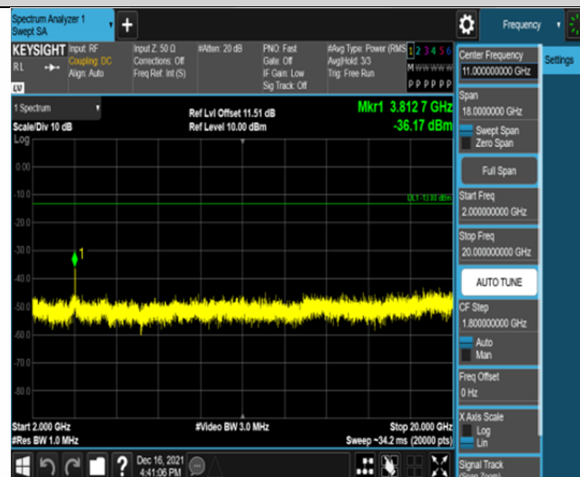
Band2-5MHz-QPSK-19175-25RB#0-Range3:2000~20000MHz
