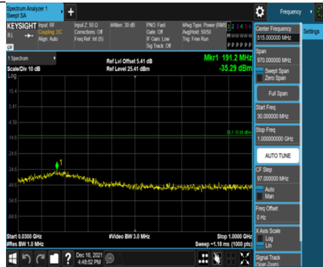
Band2-10MHz-16QAM-19150-50RB#0-Range1:30~1000MHz
