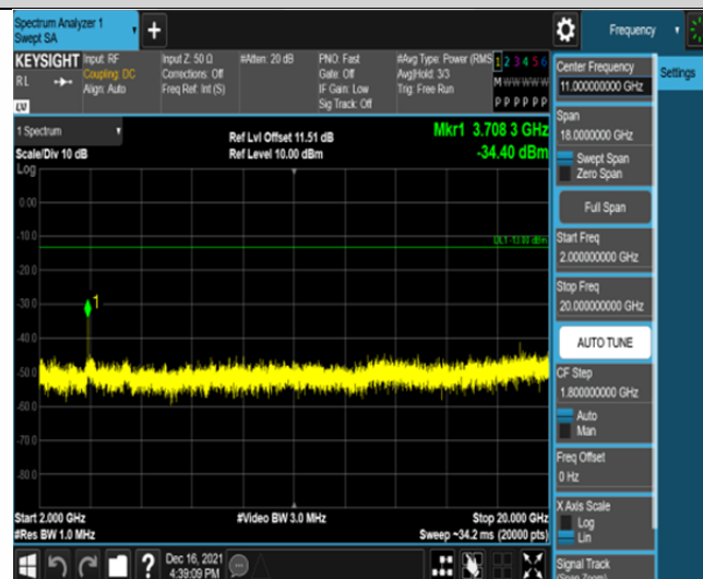
Band2-5MHz-16QAM-18625-25RB#0-Range3:2000~20000MHz
