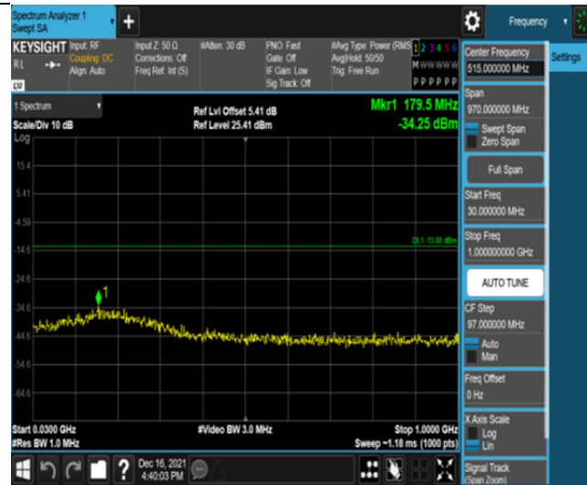
Band2-5MHz-16QAM-18900-25RB#0-Range1:30~1000MHz
