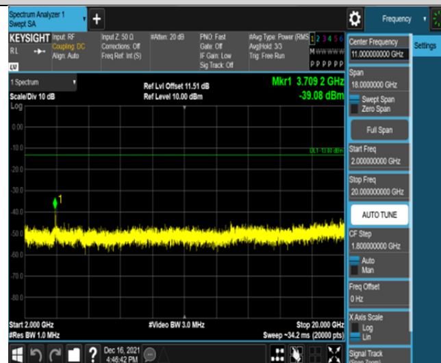
Band2-10MHz-16QAM-18650-50RB#0-Range3:2000~20000MHz
