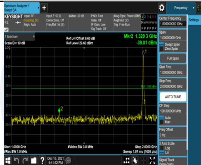
Band2-5MHz-16QAM-19175-25RB#0-Range2:1000~2000MHz
