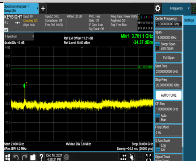
Band2-5MHz-QPSK-18625-25RB#0-Range3:2000~20000MHz
