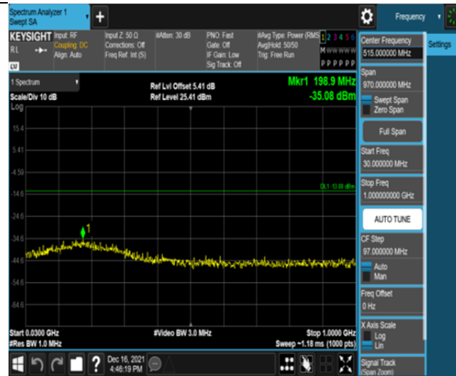
Band2-10MHz-16QAM-18650-50RB#0-Range1:30~1000MHz
