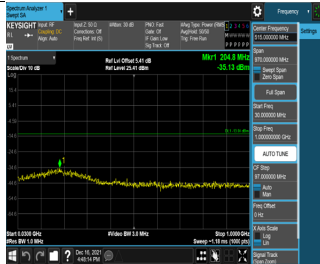
Band2-10MHz-QPSK-19150-50RB#0-Range1:30~1000MHz
