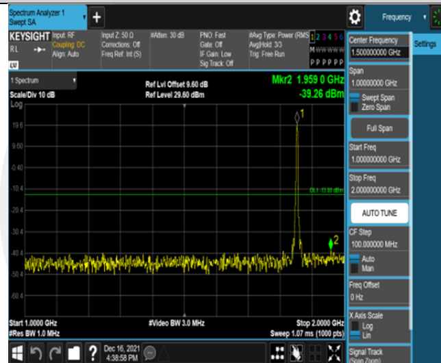
Band2-5MHz-16QAM-18625-25RB#0-Range2:1000~2000MHz
