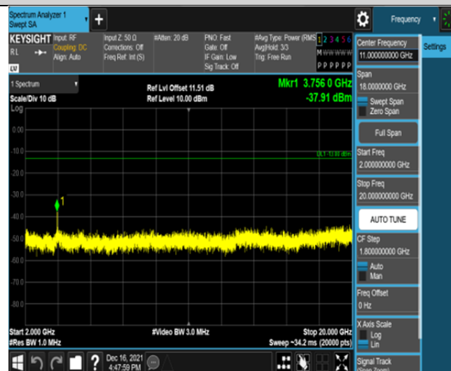
Band2-10MHz-16QAM-18900-50RB#0-Range3:2000~20000MHz
