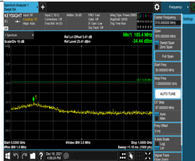
Band2-15MHz-16QAM-19125-75RB#0-Range1:30~1000MHz
