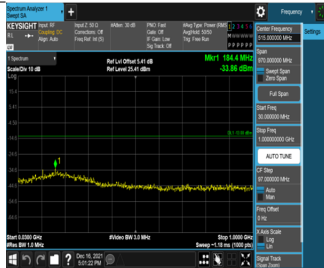
Band2-20MHz-16QAM-18700-100RB#0-Range1:30~1000MHz
