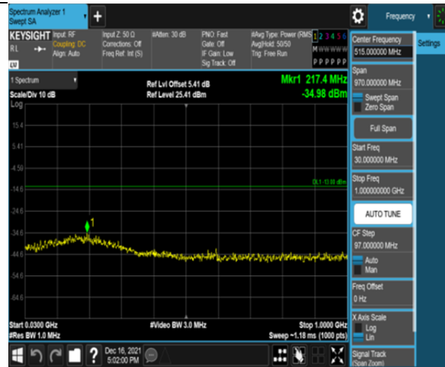
Band2-20MHz-QPSK-18900-100RB#0-Range1:30~1000MHz
