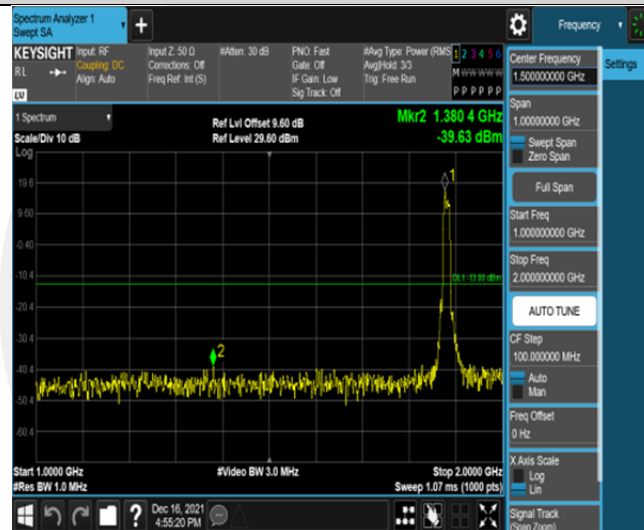
Band2-15MHz-16QAM-18900-75RB#0-Range2:1000~2000MHz
