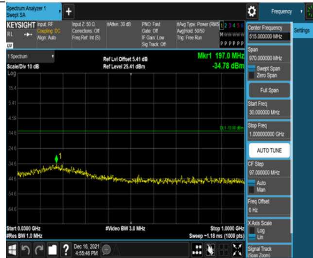
Band2-15MHz-QPSK-19125-75RB#0-Range1:30~1000MHz
