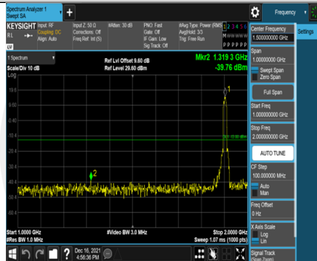
Band2-15MHz-16QAM-19125-75RB#0-Range2:1000~2000MHz
