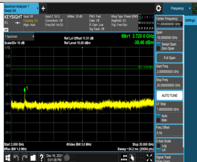
Band2-20MHz-QPSK-18700-100RB#0-Range3:2000~20000MHz
