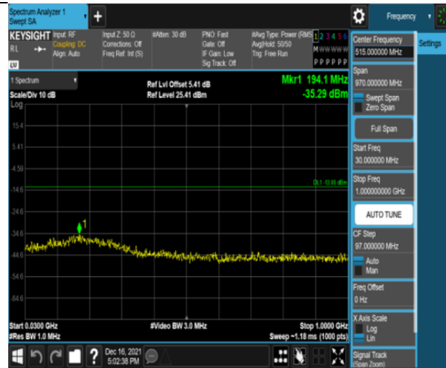
Band2-20MHz-16QAM-18900-100RB#0-Range1:30~1000MHz
