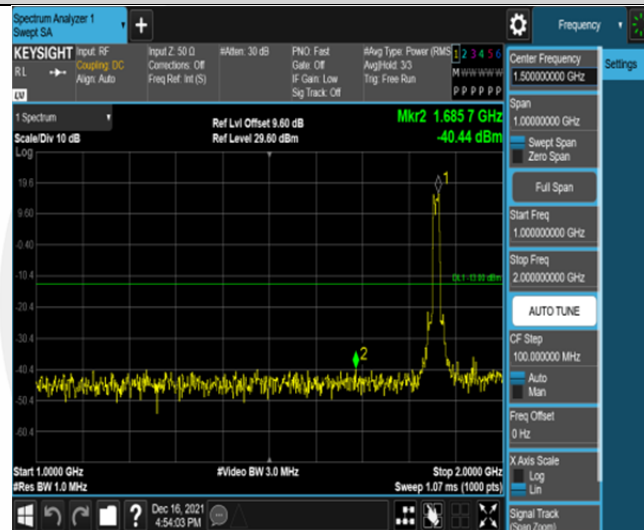
Band2-15MHz-16QAM-18675-75RB#0-Range2:1000~2000MHz
