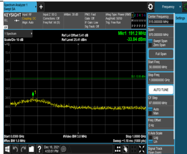
Band2-15MHz-16QAM-18675-75RB#0-Range1:30~1000MHz
