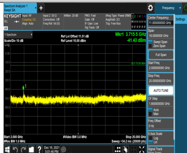
Band2-20MHz-16QAM-18700-100RB#0-Range3:2000~20000MHz
