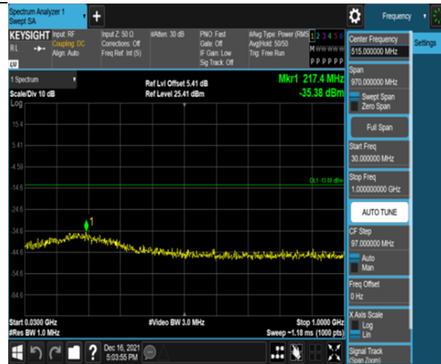
Band2-20MHz-16QAM-19100-100RB#0-Range1:30~1000MHz
