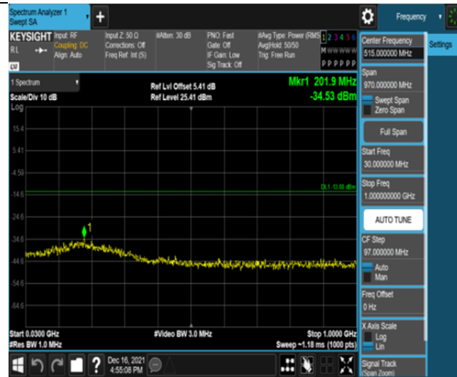
Band2-15MHz-16QAM-18900-75RB#0-Range1:30~1000MHz
