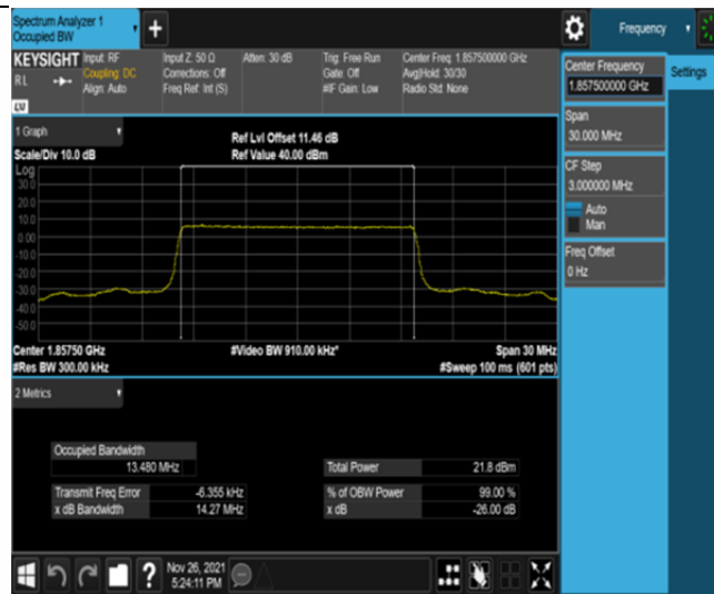
Band25-15MHz-16QAM-26115-75RB#0
