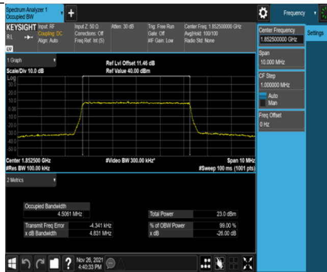
Band25-5MHz-16QAM-26065-25RB#0
