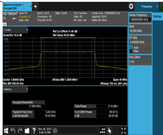
Band25-20MHz-16QAM-26140-100RB#0
