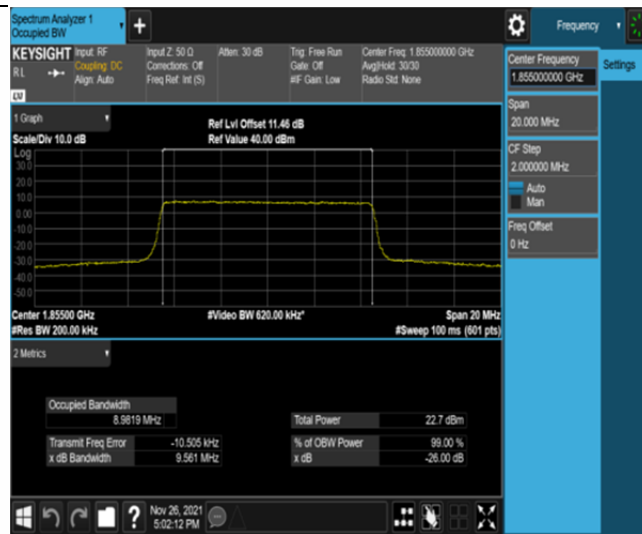
Band25-10MHz-QPSK-26090-50RB#0
