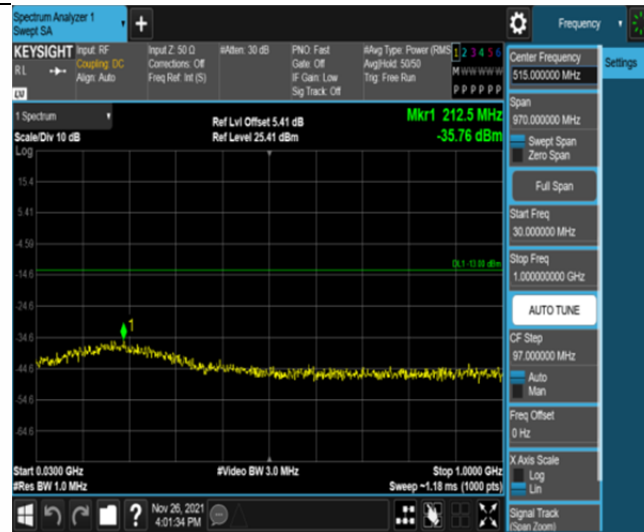
Band25-1.4MHz-16QAM-26047-6RB#0-Range1:30~1000MHz
