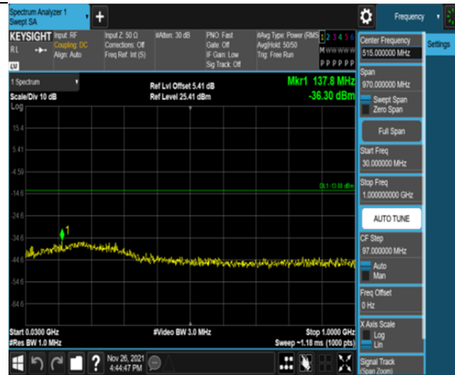
Band25-5MHz-QPSK-26365-25RB#0-Range1:30~1000MHz
