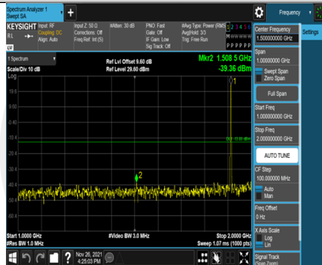
Band25-3MHz-16QAM-26675-1RB#0-Range2:1000~2000MHz
