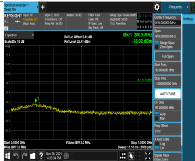
Band25-3MHz-16QAM-26365-1RB#0-Range1:30~1000MHz
