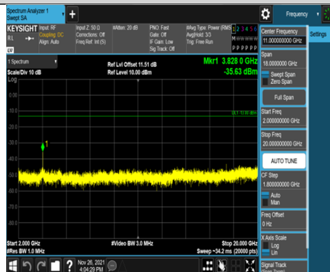
Band25-1.4MHz-16QAM-26683-6RB#0-Range3:2000~20000MHz
