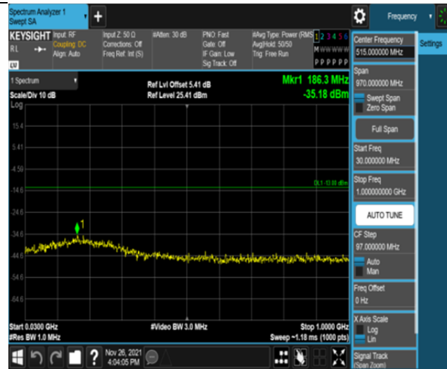
Band25-1.4MHz-16QAM-26683-6RB#0-Range1:30~1000MHz
