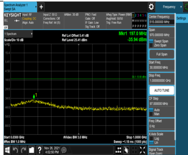
Band25-1.4MHz-16QAM-26365-6RB#0-Range1:30~1000MHz
