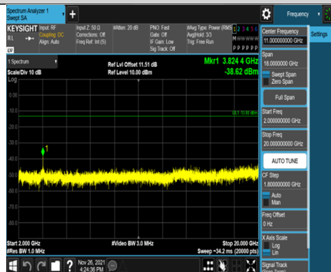
Band25-3MHz-QPSK-26675-1RB#0-Range3:2000~20000MHz
