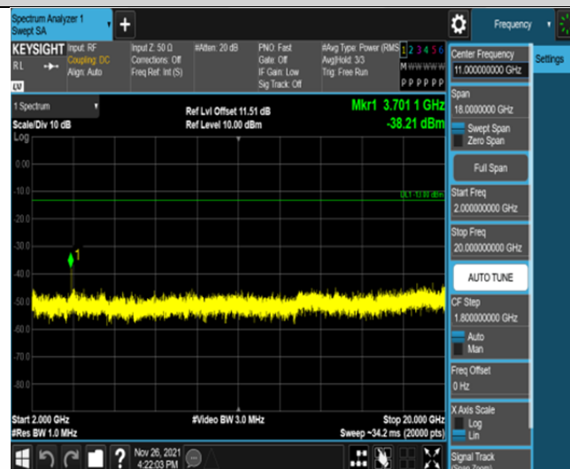
Band25-3MHz-QPSK-26055-1RB#0-Range3:2000~20000MHz
