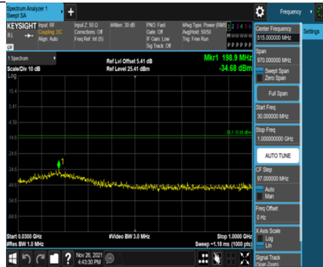
Band25-5MHz-QPSK-26065-25RB#0-Range1:30~1000MHz
