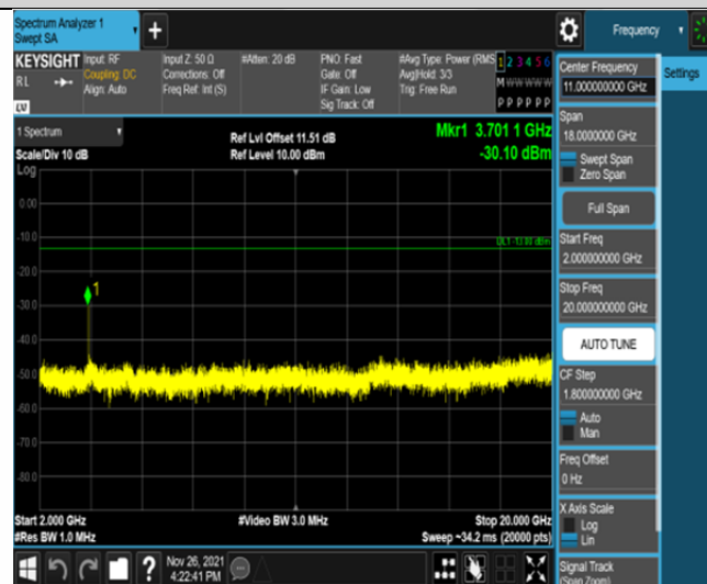
Band25-3MHz-16QAM-26055-1RB#0-Range3:2000~20000MHz
