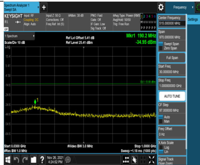
Band25-3MHz-16QAM-26675-1RB#0-Range1:30~1000MHz
