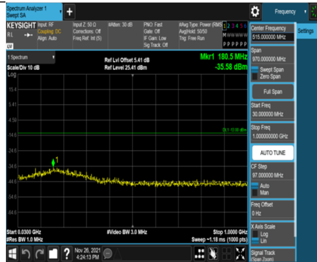
Band25-3MHz-QPSK-26675-1RB#0-Range1:30~1000MHz
