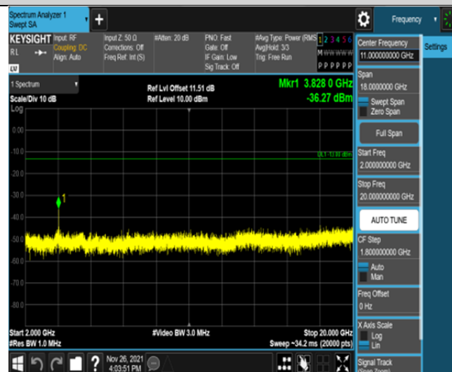
Band25-1.4MHz-QPSK-26683-6RB#0-Range3:2000~20000MHz
