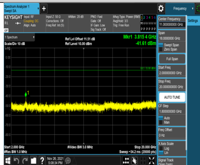
Band25-10MHz-16QAM-26640-50RB#0-Range3:2000~20000MHz
