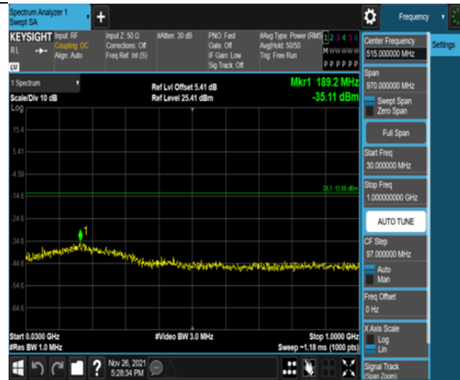
Band25-15MHz-16QAM-26365-75RB#0-Range1:30~1000MHz
