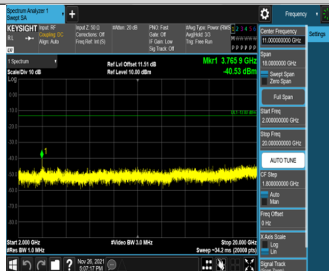
Band25-10MHz-16QAM-26365-50RB#0-Range3:2000~20000MHz
