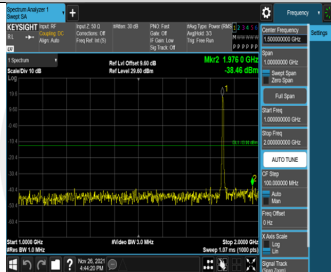
Band25-5MHz-16QAM-26065-25RB#0-Range2:1000~2000MHz
