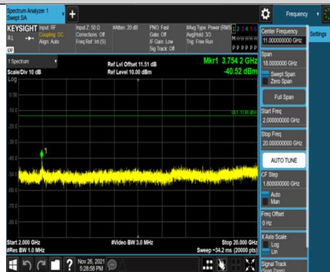
Band25-15MHz-16QAM-26365-75RB#0-Range3:2000~20000MHz
