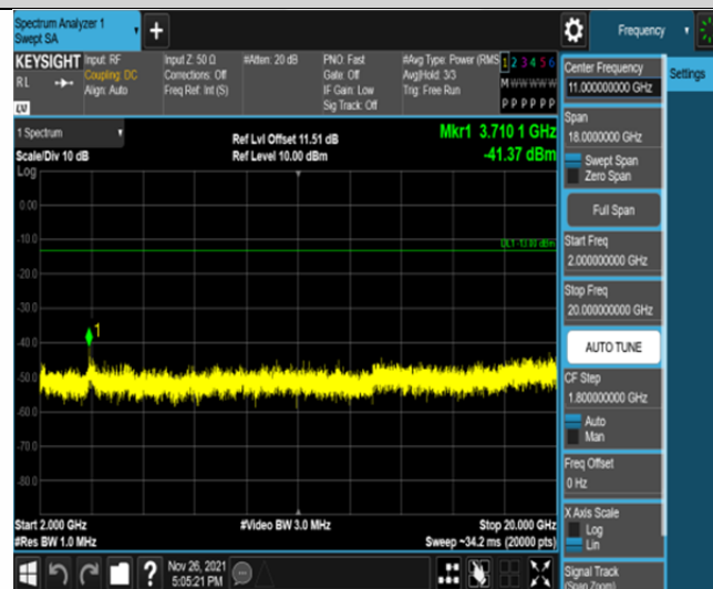
Band25-10MHz-QPSK-26090-50RB#0-Range3:2000~20000MHz
