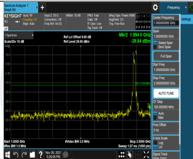
Band25-15MHz-QPSK-26365-75RB#0-Range2:1000~2000MHz
