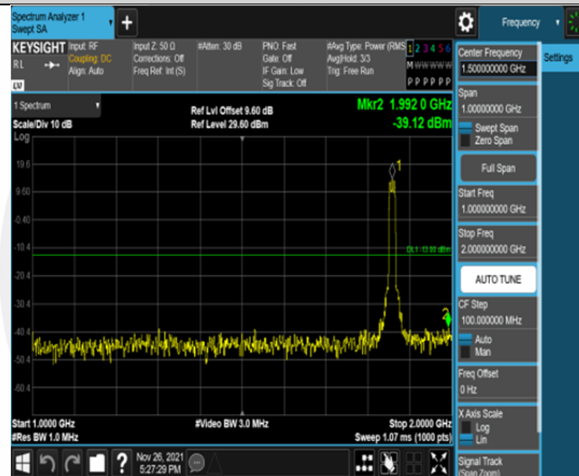
Band25-15MHz-16QAM-26115-75RB#0-Range2:1000~2000MHz
