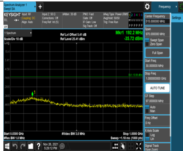
Band25-15MHz-QPSK-26615-75RB#0-Range1:30~1000MHz
