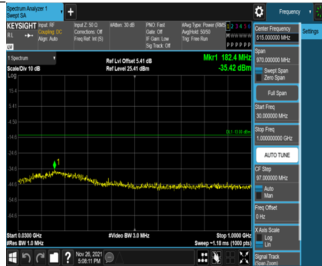
Band25-10MHz-16QAM-26640-50RB#0-Range1:30~1000MHz
