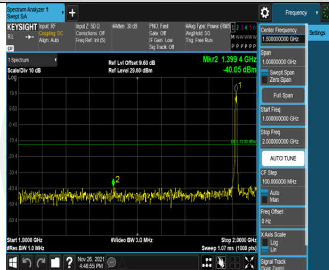
Band25-5MHz-16QAM-26665-25RB#0-Range2:1000~2000MHz
