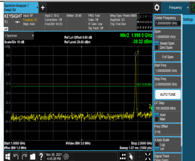
Band25-5MHz-16QAM-26365-25RB#0-Range2:1000~2000MHz
