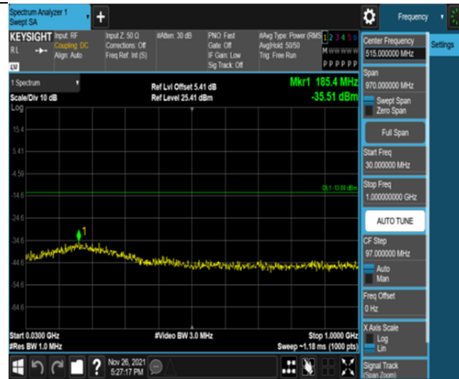
Band25-15MHz-16QAM-26115-75RB#0-Range1:30~1000MHz
