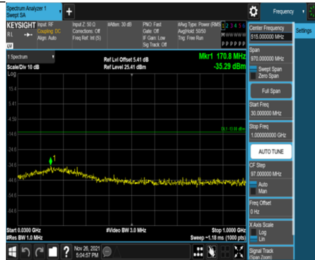
Band25-10MHz-QPSK-26090-50RB#0-Range1:30~1000MHz
