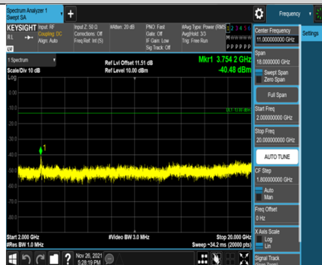
Band25-15MHz-QPSK-26365-75RB#0-Range3:2000~20000MHz
