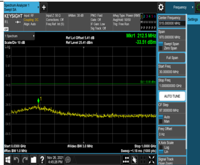
Band25-5MHz-16QAM-26365-25RB#0-Range1:30~1000MHz
