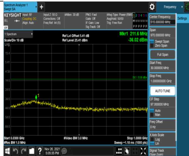
Band25-10MHz-16QAM-26090-50RB#0-Range1:30~1000MHz
