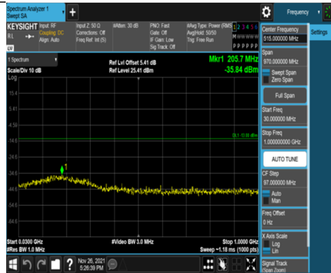
Band25-15MHz-QPSK-26115-75RB#0-Range1:30~1000MHz
