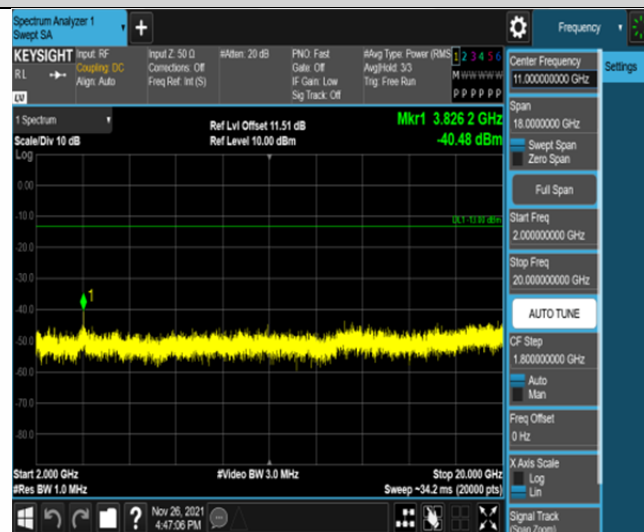
Band25-5MHz-16QAM-26665-25RB#0-Range3:2000~20000MHz
