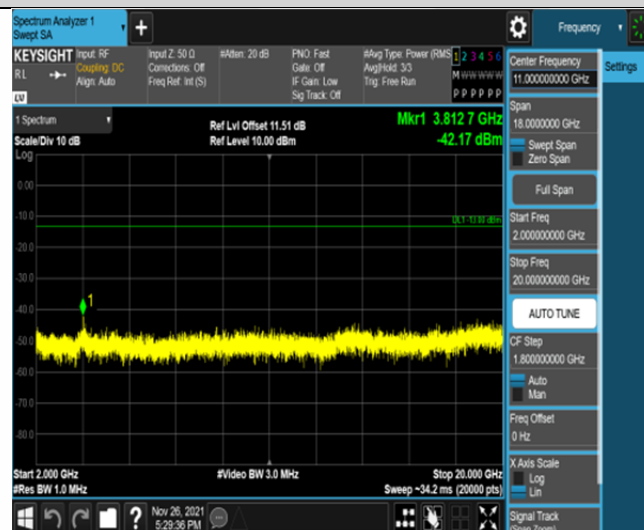
Band25-15MHz-QPSK-26615-75RB#0-Range3:2000~20000MHz
