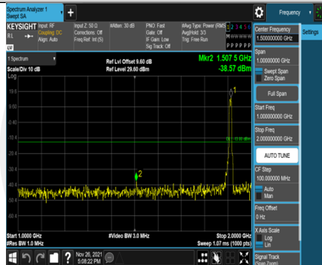
Band25-10MHz-16QAM-26640-50RB#0-Range2:1000~2000MHz
