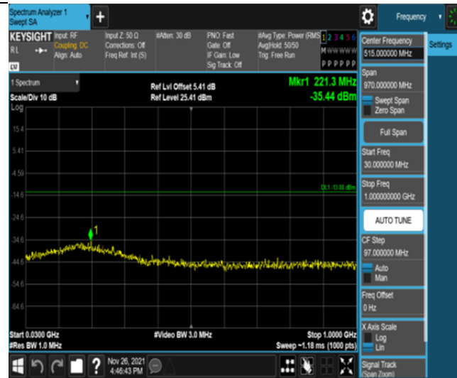
Band25-5MHz-16QAM-26665-25RB#0-Range1:30~1000MHz
