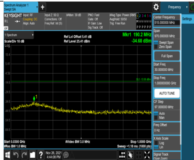
Band25-5MHz-16QAM-26065-25RB#0-Range1:30~1000MHz
