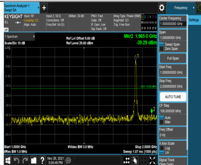
Band25-10MHz-16QAM-26090-50RB#0-Range2:1000~2000MHz
