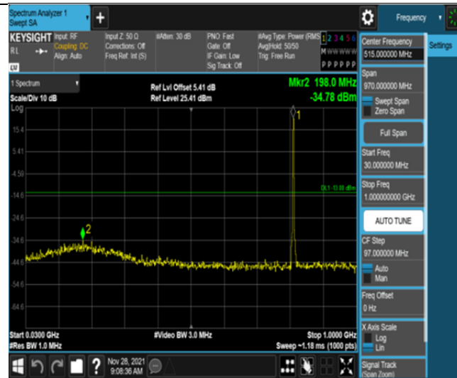
Band26-1.4MHz-QPSK-26697-6RB#0-Range1:30~1000MHz
