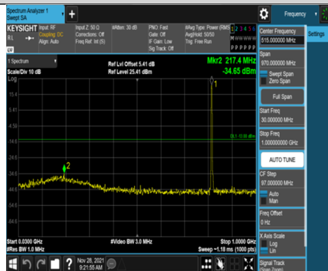
Band26-1.4MHz-16QAM-26740-6RB#0-Range1:30~1000MHz
