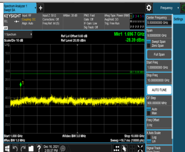
Band26-1.4MHz-16QAM-27033-6RB#0-Range2:1000~10000MHz
