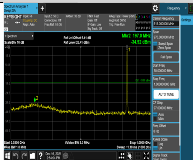
Band26-1.4MHz-QPSK-26915-6RB#0-Range1:30~1000MHz
