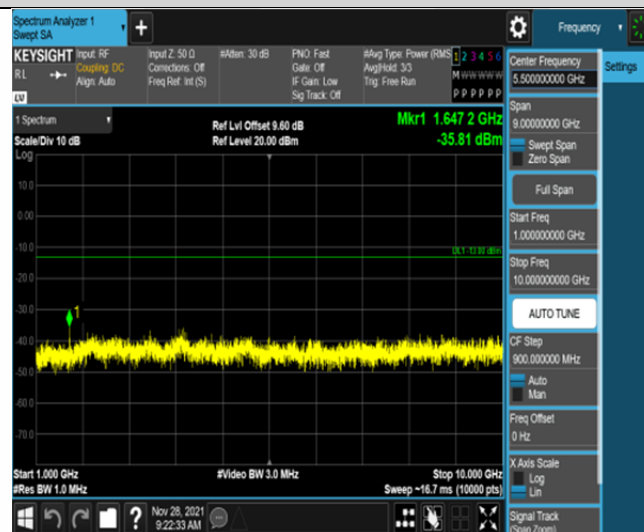
Band26-1.4MHz-QPSK-26783-6RB#0-Range2:1000~10000MHz
