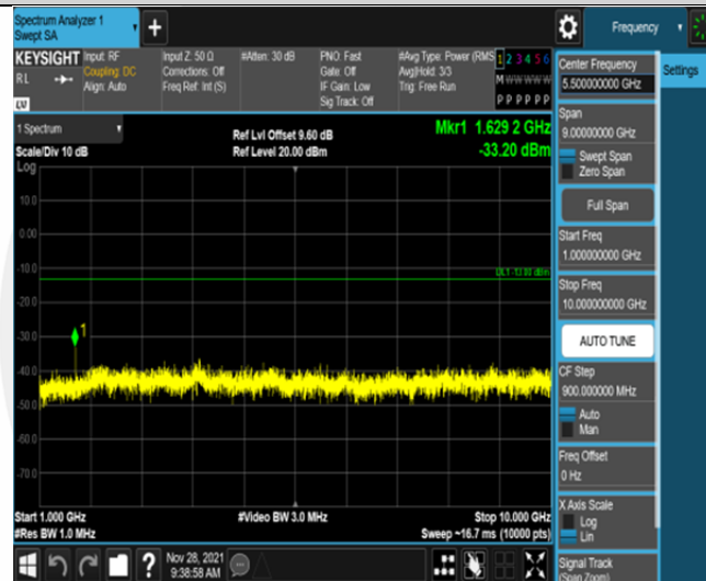
Band26-3MHz-16QAM-26705-1RB#0-Range2:1000~10000MHz
