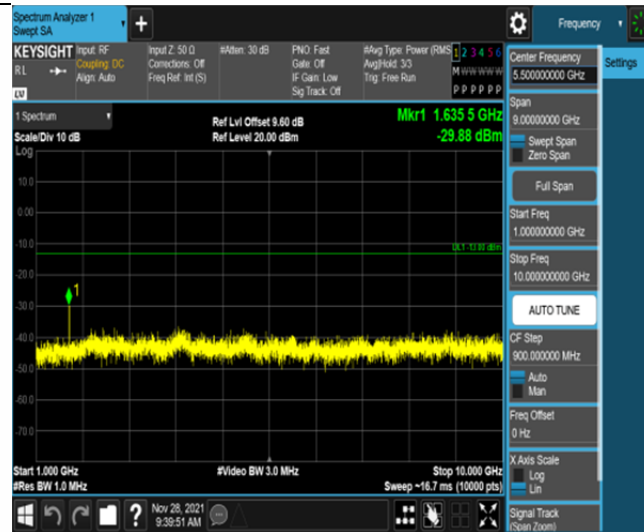
Band26-3MHz-16QAM-26740-1RB#0-Range2:1000~10000MHz
