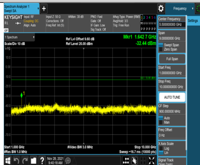
Band26-3MHz-QPSK-26775-1RB#0-Range2:1000~10000MHz
