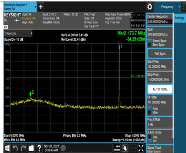
Band26-3MHz-16QAM-26705-1RB#0-Range1:30~1000MHz
