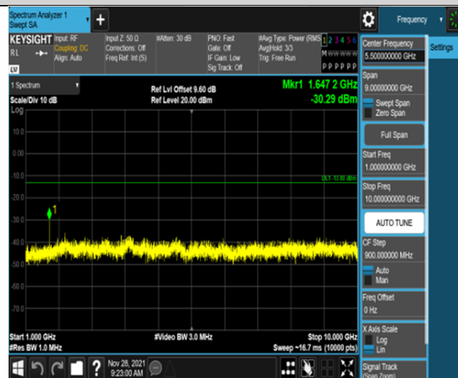
Band26-1.4MHz-16QAM-26783-6RB#0-Range2:1000~10000MHz
