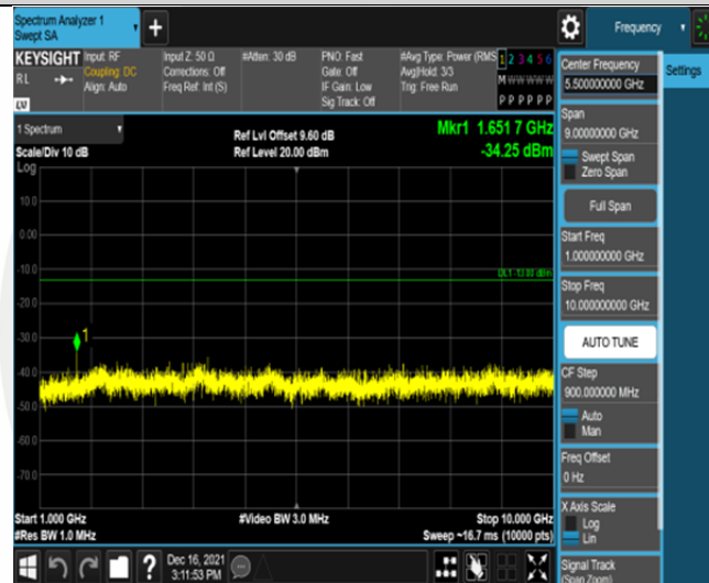
Band26-3MHz-QPSK-26805-15RB#0-Range2:1000~10000MHz
