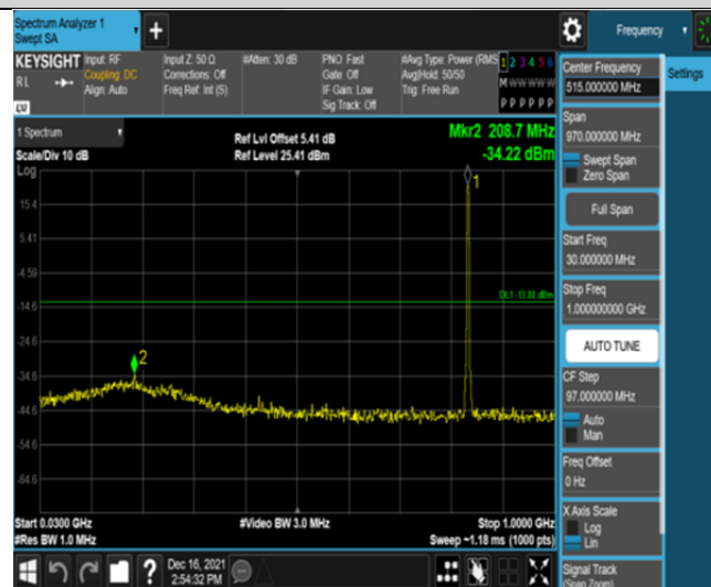
Band26-1.4MHz-16QAM-26915-6RB#0-Range1:30~1000MHz
