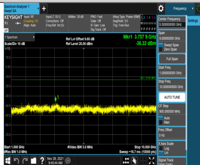
Band26-3MHz-16QAM-26775-1RB#0-Range2:1000~10000MHz
