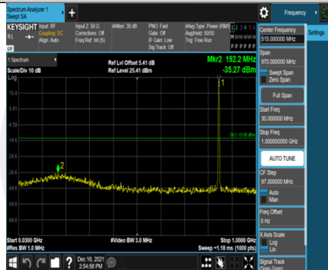
Band26-1.4MHz-QPSK-27033-6RB#0-Range1:30~1000MHz
