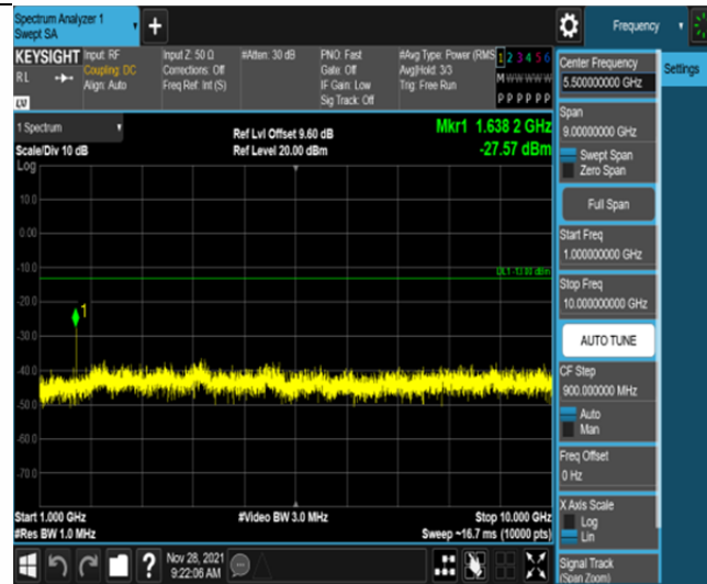
Band26-1.4MHz-16QAM-26740-6RB#0-Range2:1000~10000MHz
