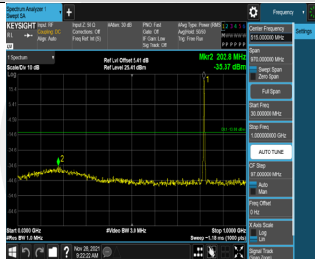
Band26-1.4MHz-QPSK-26783-6RB#0-Range1:30~1000MHz
