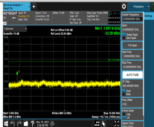
Band26-1.4MHz-QPSK-27033-6RB#0-Range2:1000~10000MHz
