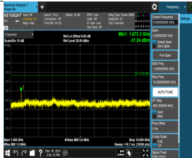
Band26-1.4MHz-QPSK-26915-6RB#0-Range2:1000~10000MHz
