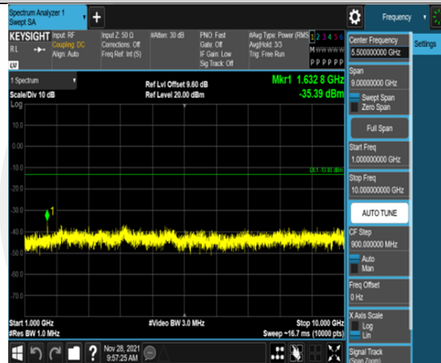
Band26-5MHz-QPSK-26715-25RB#0-Range2:1000~10000MHz
