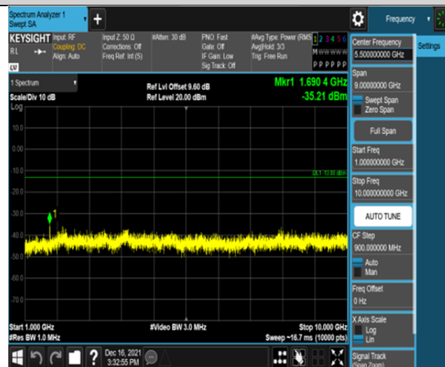
Band26-5MHz-QPSK-27015-25RB#0-Range2:1000~10000MHz
