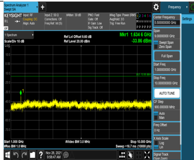
Band26-5MHz-16QAM-26740-25RB#0-Range2:1000~10000MHz
