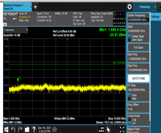
Band26-5MHz-16QAM-27015-25RB#0-Range2:1000~10000MHz
