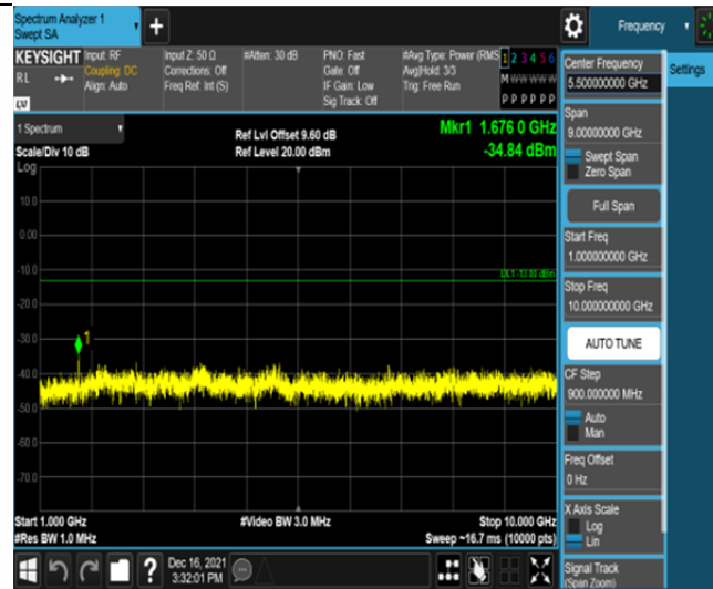
Band26-5MHz-QPSK-26915-25RB#0-Range2:1000~10000MHz
