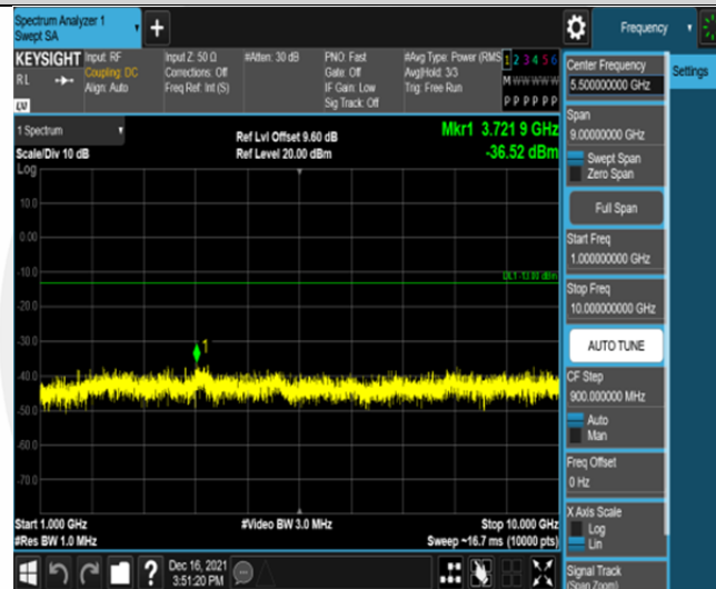
Band26-10MHz-16QAM-26915-50RB#0-Range2:1000~10000MHz
