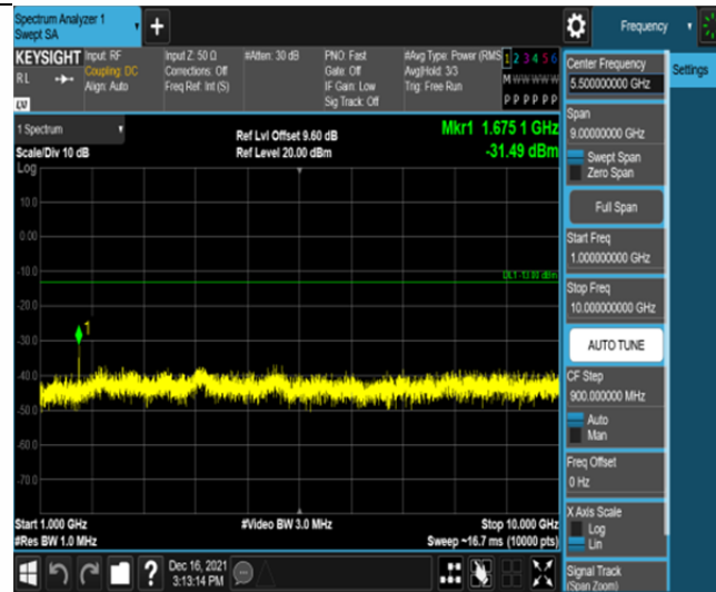
Band26-3MHz-16QAM-26915-15RB#0-Range2:1000~10000MHz
