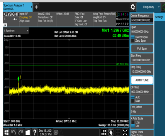
Band26-3MHz-16QAM-27025-15RB#0-Range2:1000~10000MHz
