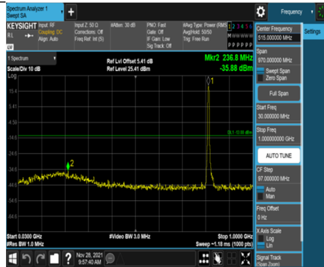
Band26-5MHz-16QAM-26715-25RB#0-Range1:30~1000MHz
