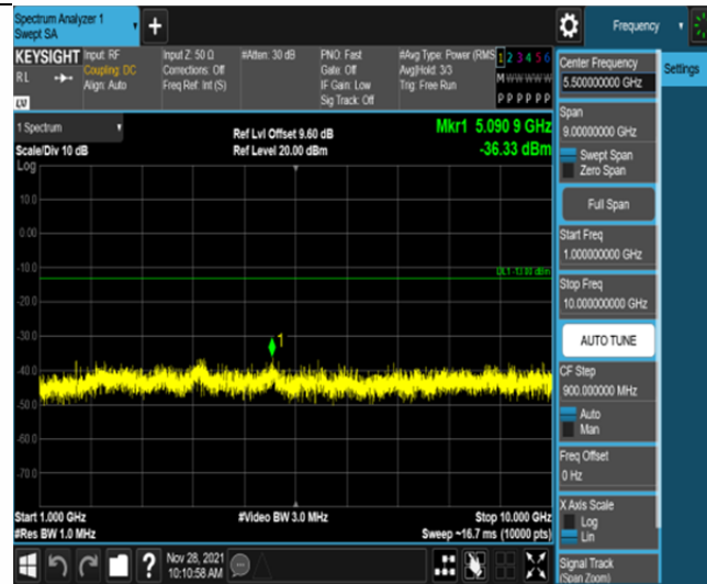
Band26-10MHz-16QAM-26740-50RB#0-Range2:1000~10000MHz
