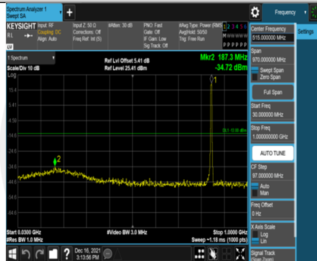
Band26-3MHz-16QAM-27025-15RB#0-Range1:30~1000MHz
