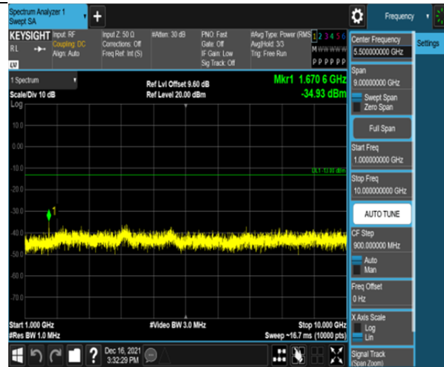
Band26-5MHz-16QAM-26915-25RB#0-Range2:1000~10000MHz
