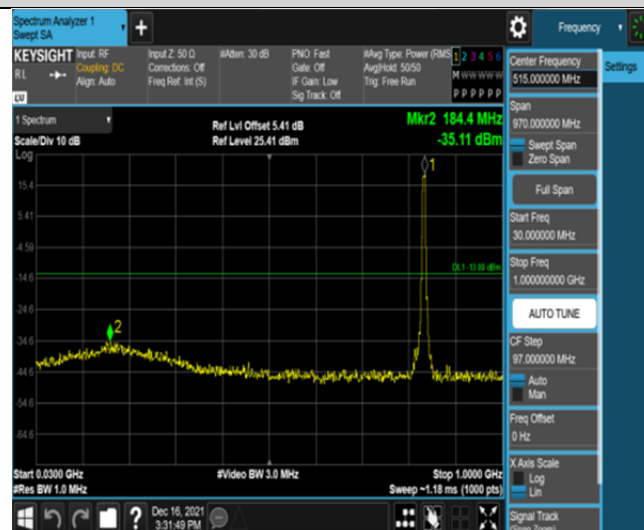
Band26-5MHz-QPSK-26915-25RB#0-Range1:30~1000MHz
