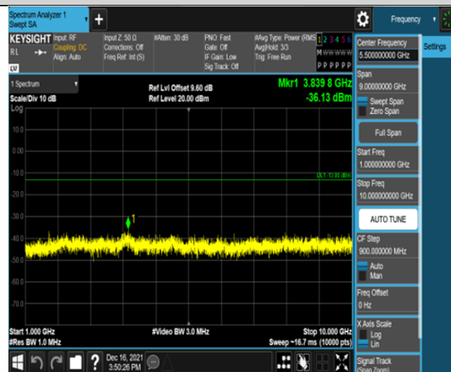
Band26-10MHz-16QAM-26840-50RB#0-Range2:1000~10000MHz
