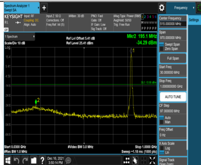
Band26-10MHz-16QAM-26840-50RB#0-Range1:30~1000MHz
