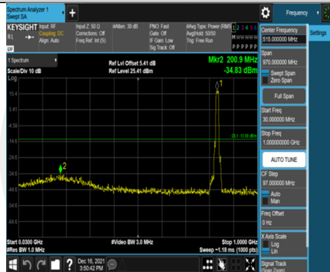
Band26-10MHz-QPSK-26915-50RB#0-Range1:30~1000MHz
