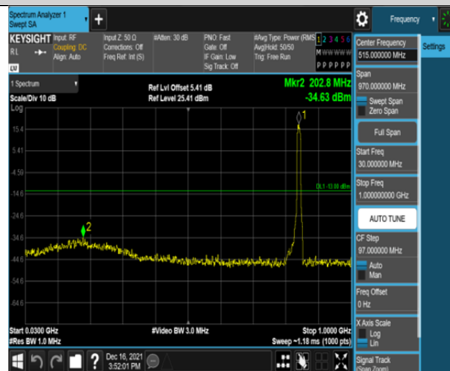
Band26-10MHz-16QAM-26990-50RB#0-Range1:30~1000MHz
