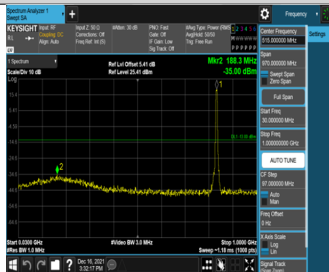
Band26-5MHz-16QAM-26915-25RB#0-Range1:30~1000MHz
