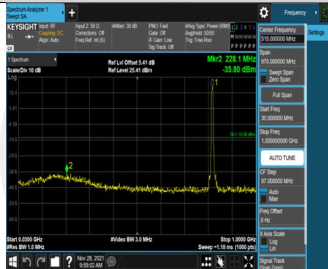
Band26-5MHz-QPSK-26765-25RB#0-Range1:30~1000MHz
