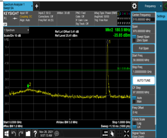
Band26-5MHz-QPSK-26715-25RB#0-Range1:30~1000MHz
