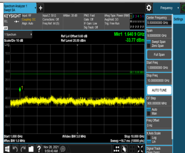
Band26-5MHz-16QAM-26765-25RB#0-Range2:1000~10000MHz
