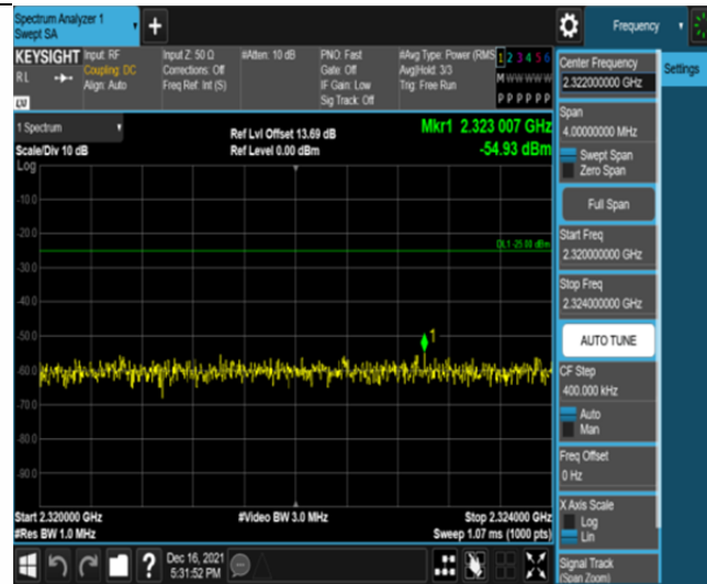
Band30-5MHz-QPSK-27685-25RB#0-Range7:2320~2324MHz
