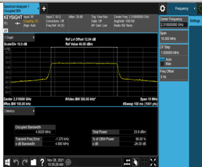
Band30-5MHz-QPSK-27710-25RB#0
