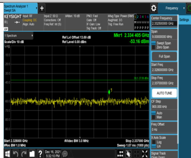
Band30-5MHz-QPSK-27685-25RB#0-Range9:2328~2337MHz
