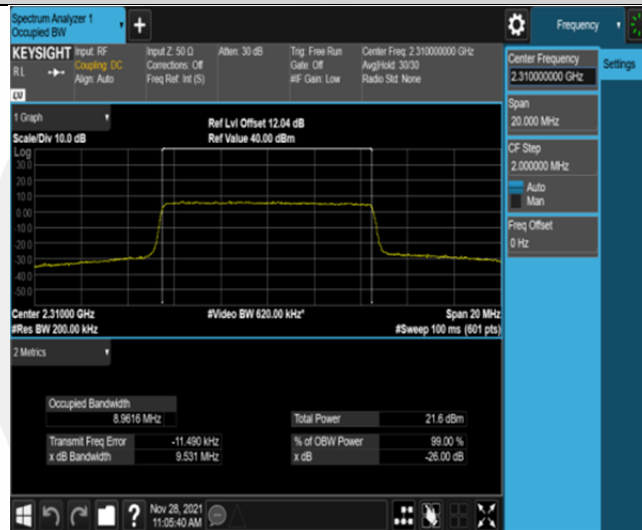
Band30-10MHz-16QAM-27710-50RB#0
