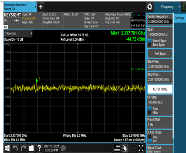
Band30-5MHz-QPSK-27685-25RB#0-Range10:2337~2341MHz
