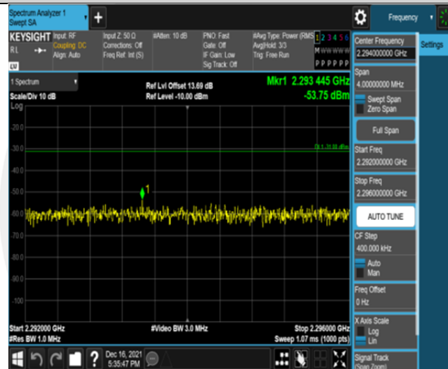
Band30-5MHz-QPSK-27710-25RB#0-Range4:2292~2296MHz
