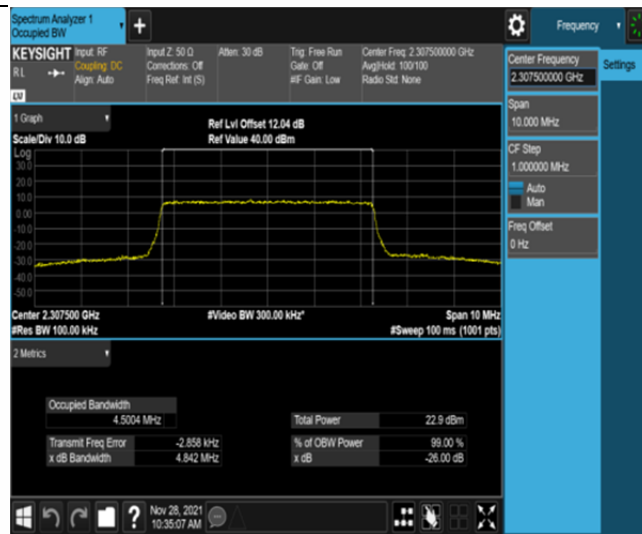
Band30-5MHz-16QAM-27685-25RB#0
