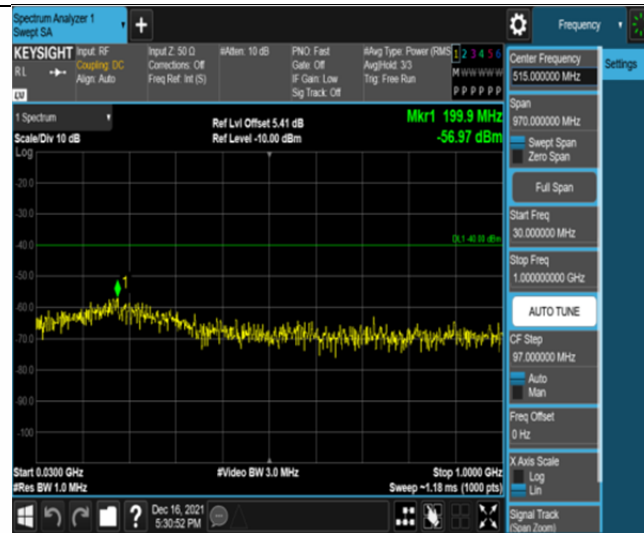
Band30-5MHz-QPSK-27685-25RB#0-Range1:30~1000MHz
