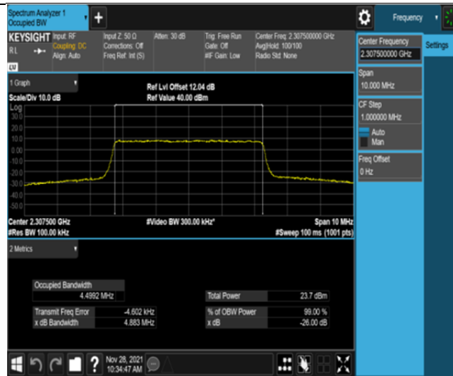
Band30-5MHz-QPSK-27685-25RB#0
