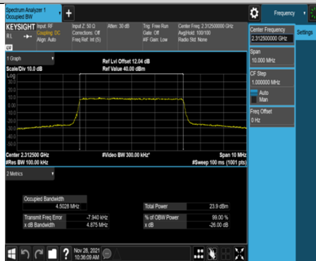
Band30-5MHz-QPSK-27735-25RB#0
