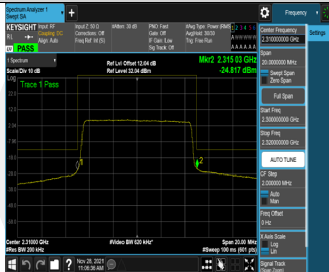
Band30-10MHz-QPSK-27710-50RB#0
