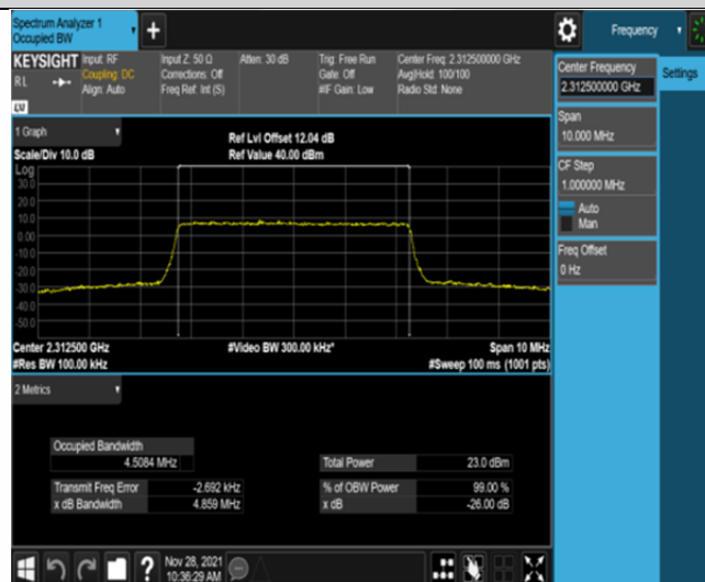
Band30-5MHz-16QAM-27735-25RB#0
