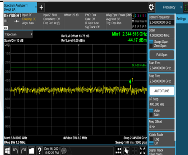
Band30-5MHz-QPSK-27685-25RB#0-Range11:2341~2345MHz
