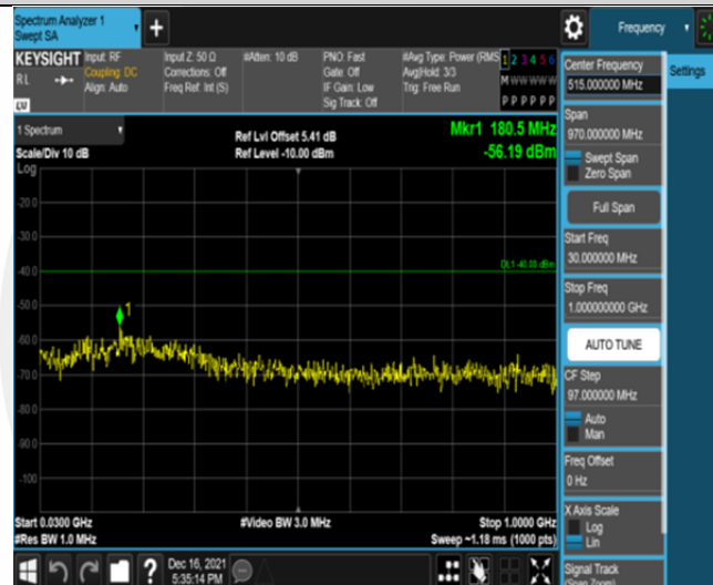
Band30-5MHz-QPSK-27710-25RB#0-Range1:30~1000MHz
