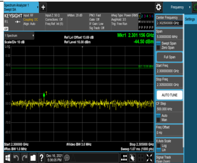
Band30-5MHz-QPSK-27710-25RB#0-Range6:2300~2305MHz
