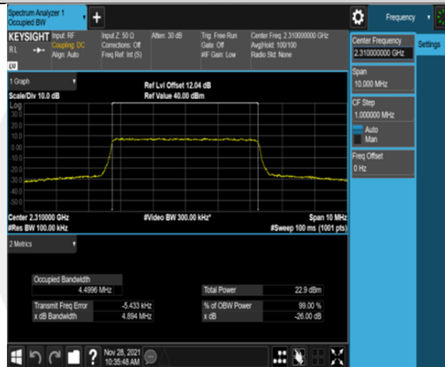
Band30-5MHz-16QAM-27710-25RB#0
