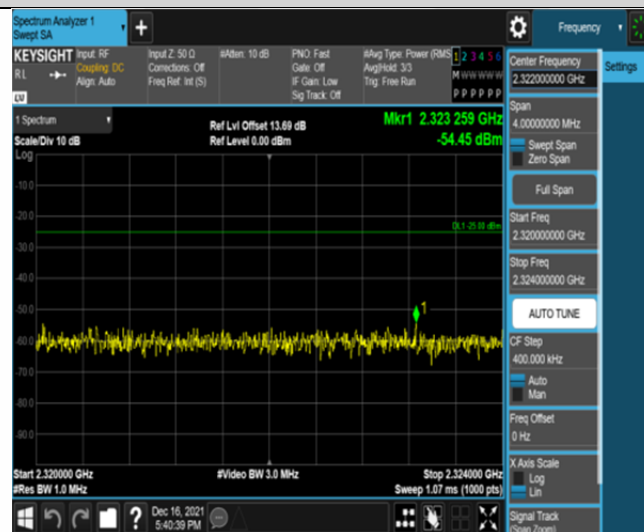
Band30-5MHz-QPSK-27735-25RB#0-Range7:2320~2324MHz
