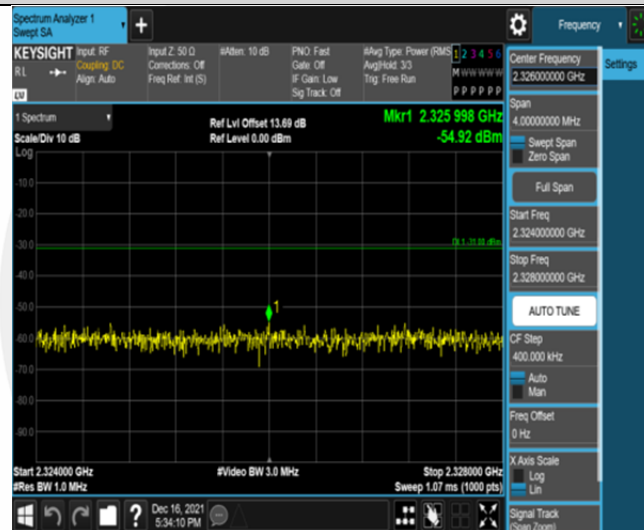
Band30-5MHz-16QAM-27685-25RB#0-Range8:2324~2328MHz
