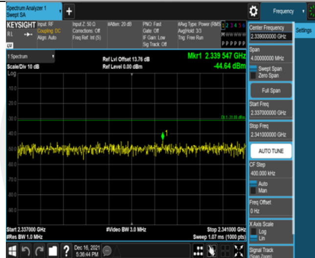
Band30-5MHz-QPSK-27710-25RB#0-Range10:2337~2341MHz
