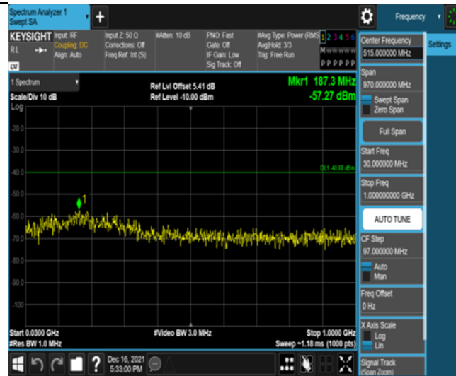
Band30-5MHz-16QAM-27685-25RB#0-Range1:30~1000MHz
