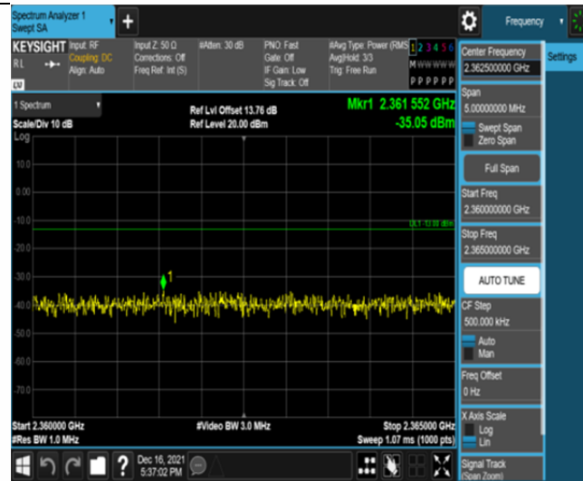
Band30-5MHz-QPSK-27710-25RB#0-Range12:2360~2365MHz
