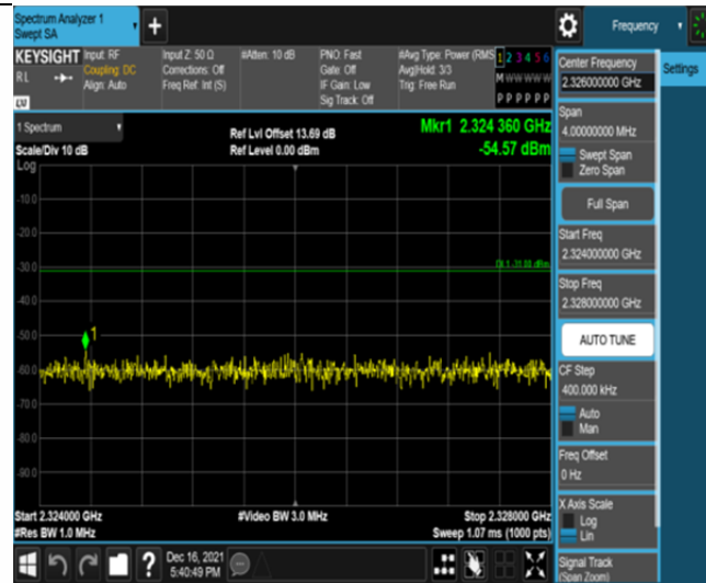
Band30-5MHz-QPSK-27735-25RB#0-Range8:2324~2328MHz
