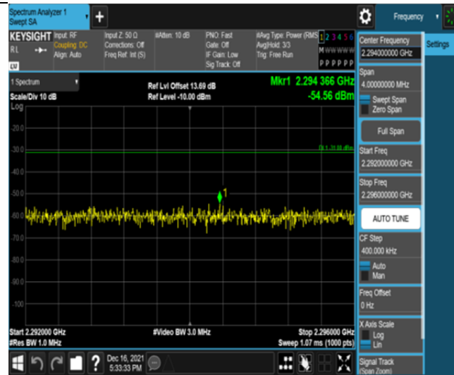
Band30-5MHz-16QAM-27685-25RB#0-Range4:2292~2296MHz
