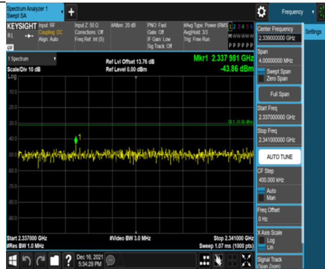
Band30-5MHz-16QAM-27685-25RB#0-Range10:2337~2341MHz
