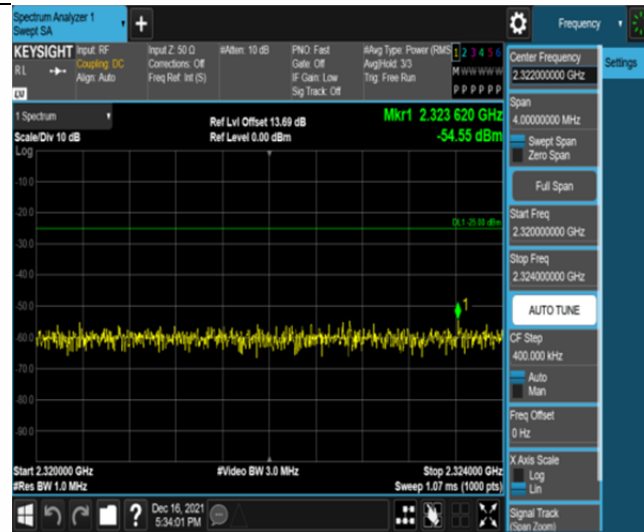
Band30-5MHz-16QAM-27685-25RB#0-Range7:2320~2324MHz
