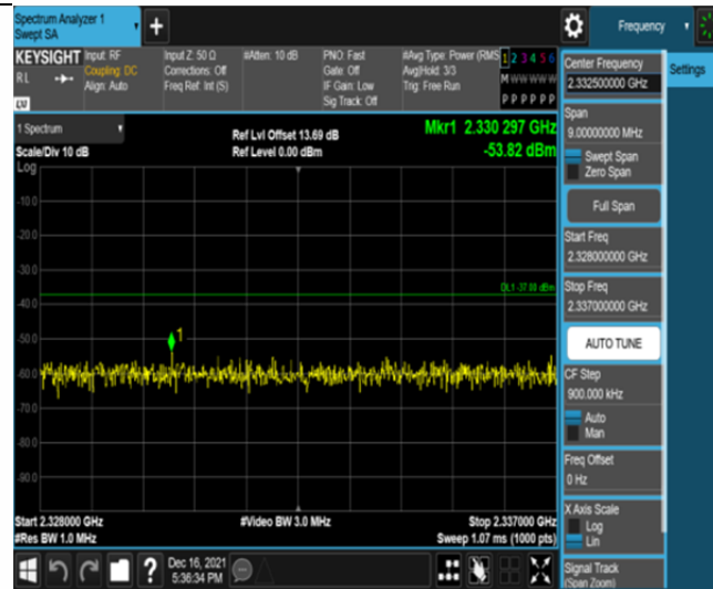
Band30-5MHz-QPSK-27710-25RB#0-Range9:2328~2337MHz
