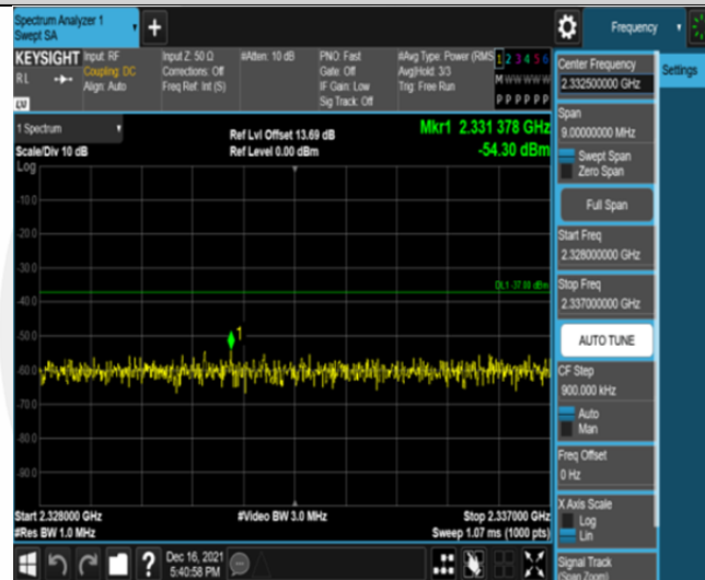
Band30-5MHz-QPSK-27735-25RB#0-Range9:2328~2337MHz
