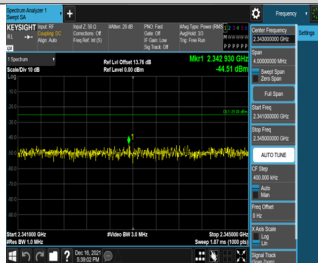
Band30-5MHz-16QAM-27710-25RB#0-Range11:2341~2345MHz
