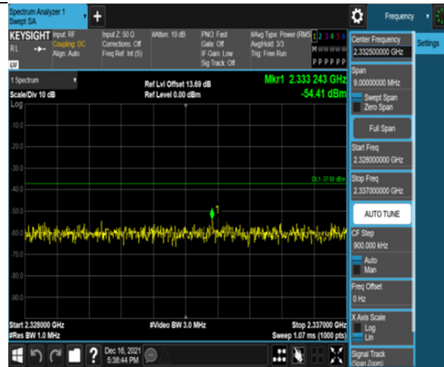
Band30-5MHz-16QAM-27710-25RB#0-Range9:2328~2337MHz
