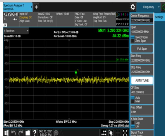
Band30-5MHz-16QAM-27685-25RB#0-Range3:2288~2292MHz
