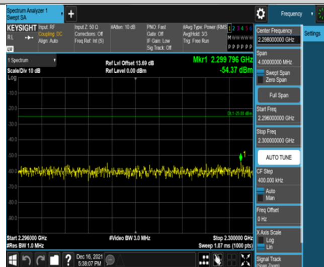
Band30-5MHz-16QAM-27710-25RB#0-Range5:2296~2300MHz
