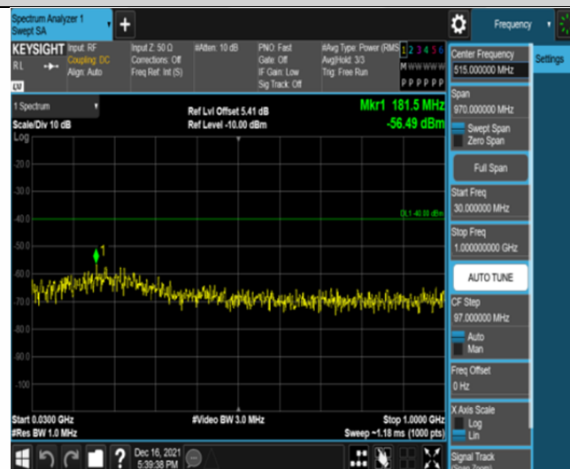
Band30-5MHz-QPSK-27735-25RB#0-Range1:30~1000MHz
