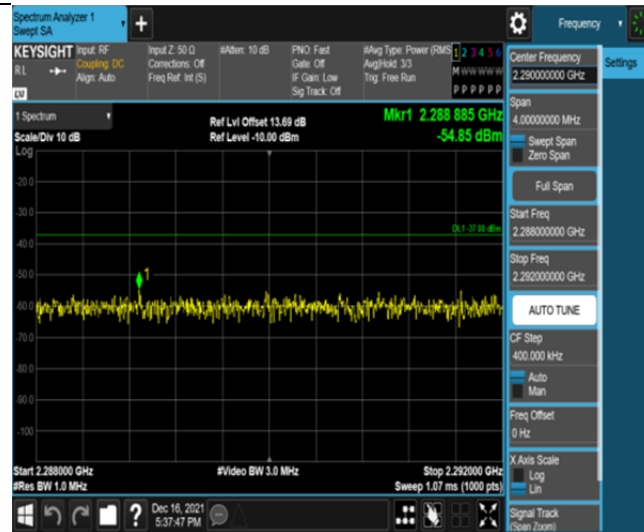
Band30-5MHz-16QAM-27710-25RB#0-Range3:2288~2292MHz
