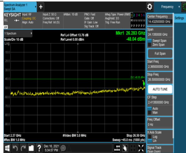
Band30-5MHz-16QAM-27685-25RB#0-Range13:2365~26500MHz
