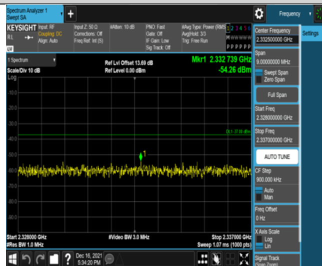
Band30-5MHz-16QAM-27685-25RB#0-Range9:2328~2337MHz
