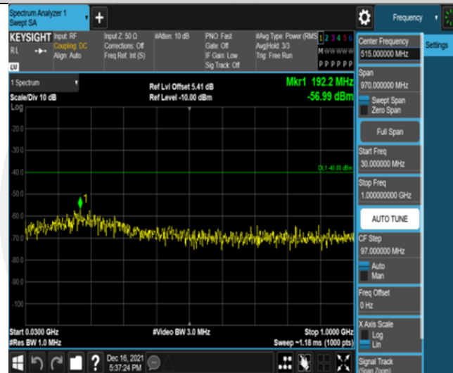
Band30-5MHz-16QAM-27710-25RB#0-Range1:30~1000MHz
