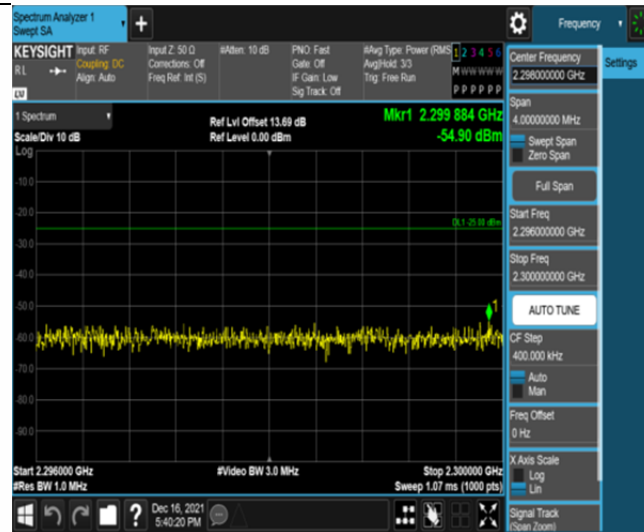
Band30-5MHz-QPSK-27735-25RB#0-Range5:2296~2300MHz
