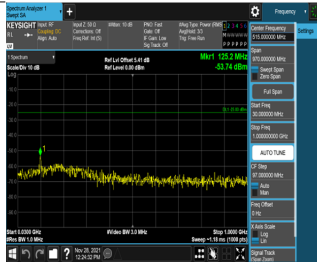
Band41-5MHz-16QAM-41565-25RB#0-Range1:30~1000MHz
