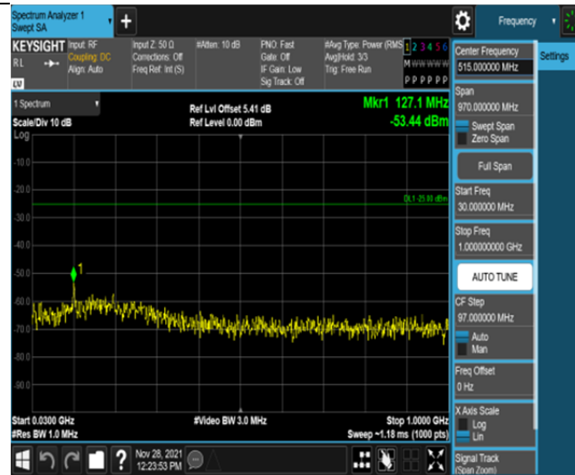
Band41-5MHz-QPSK-41565-25RB#0-Range1:30~1000MHz
