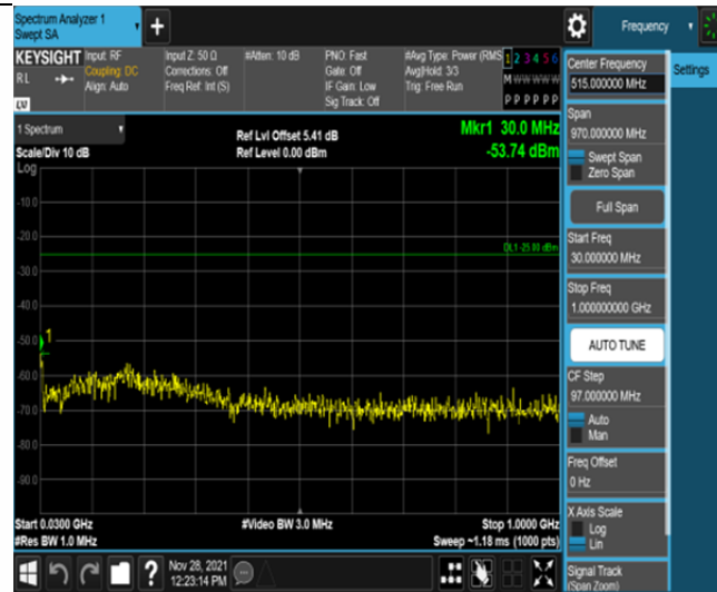
Band41-5MHz-16QAM-40620-25RB#0-Range1:30~1000MHz
