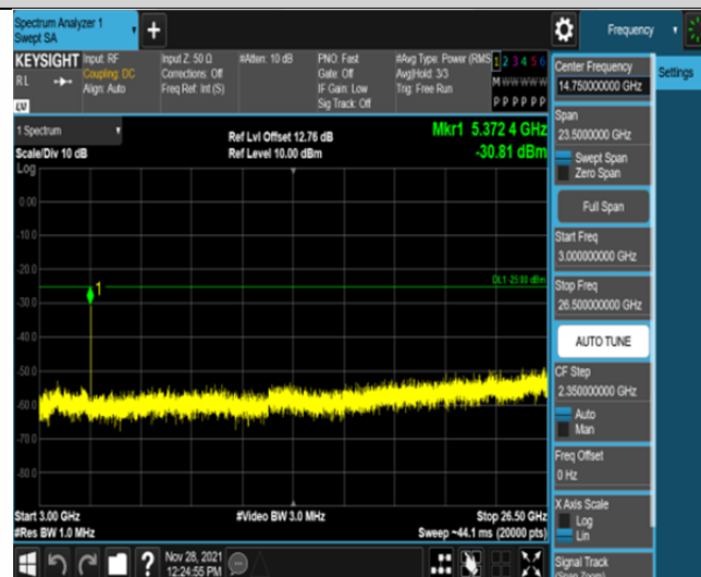
Band41-5MHz-16QAM-41565-25RB#0-Range3:3000~26500MHz
