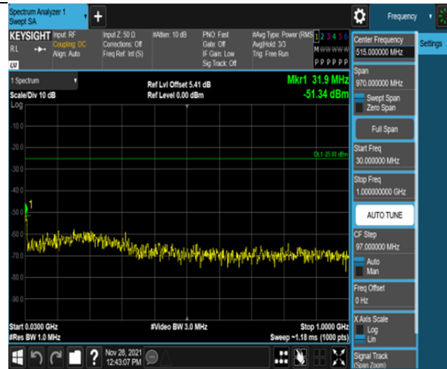
Band41-10MHz-QPSK-40620-50RB#0-Range1:30~1000MHz
