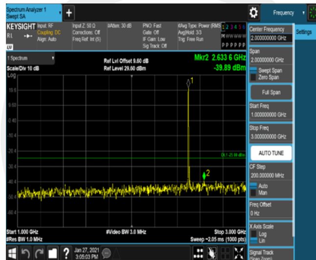
Band41-5MHz-16QAM-39675-25RB#0-Range2:1000~3000MHz
