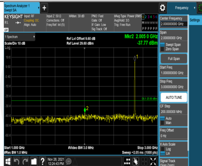
Band41-5MHz-16QAM-41565-25RB#0-Range2:1000~3000MHz
