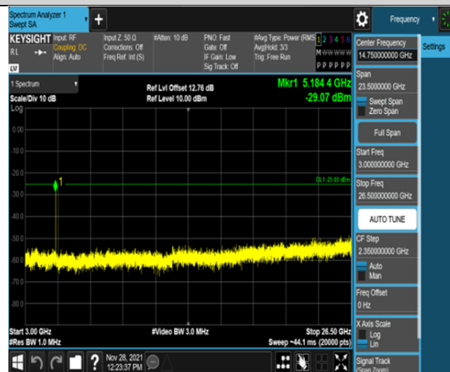
Band41-5MHz-16QAM-40620-25RB#0-Range3:3000~26500MHz
