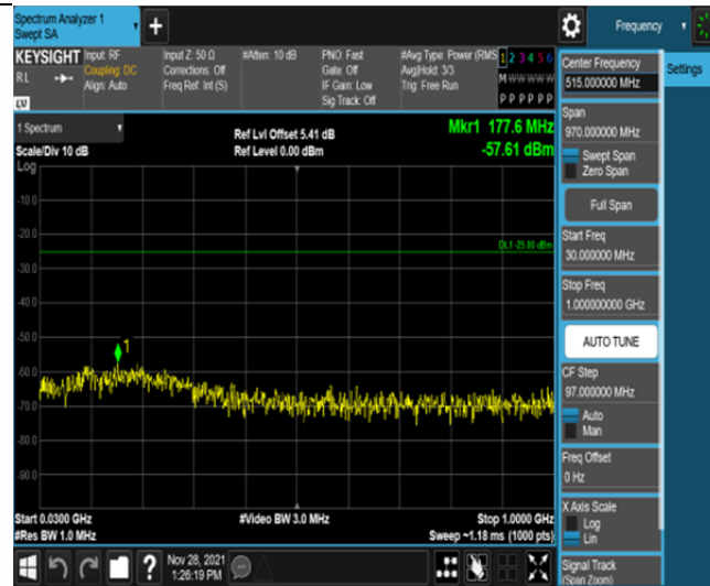
Band41-20MHz-QPSK-41490-100RB#0-Range1:30~1000MHz
