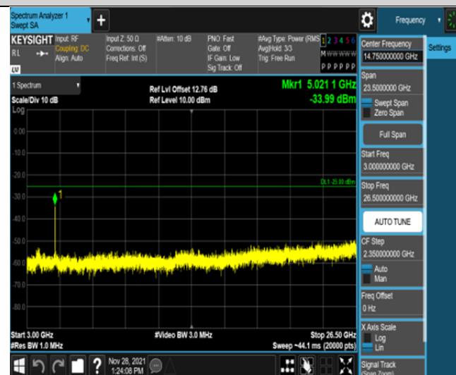
Band41-20MHz-QPSK-39750-100RB#0-Range3:3000~26500MHz
