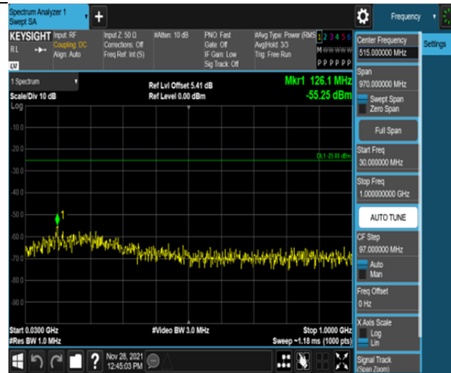
Band41-10MHz-16QAM-41540-50RB#0-Range1:30~1000MHz
