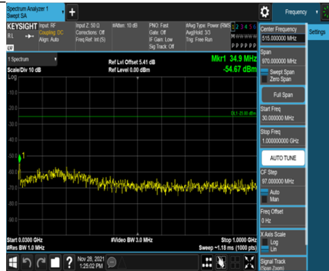
Band41-20MHz-QPSK-40620-100RB#0-Range1:30~1000MHz
