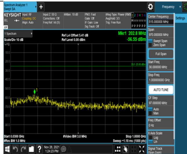
Band41-20MHz-16QAM-39750-100RB#0-Range1:30~1000MHz
