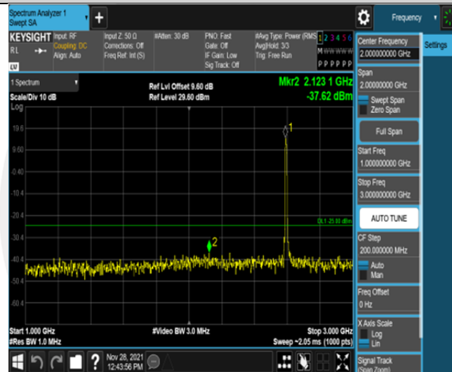
Band41-10MHz-16QAM-40620-50RB#0-Range2:1000~3000MHz
