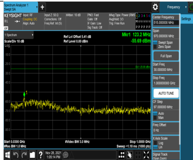
Band41-15MHz-QPSK-41515-75RB#0-Range1:30~1000MHz
