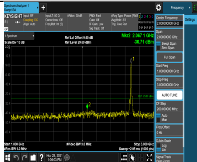
Band41-15MHz-16QAM-41515-75RB#0-Range2:1000~3000MHz
