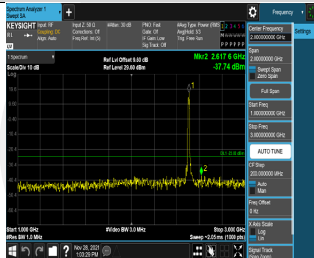
Band41-15MHz-16QAM-39725-75RB#0-Range2:1000~3000MHz
