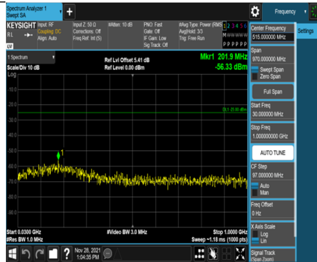
Band41-15MHz-16QAM-40620-75RB#0-Range1:30~1000MHz
