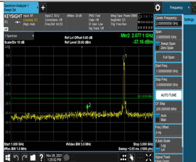
Band41-20MHz-16QAM-40620-100RB#0-Range2:1000~3000MHz
