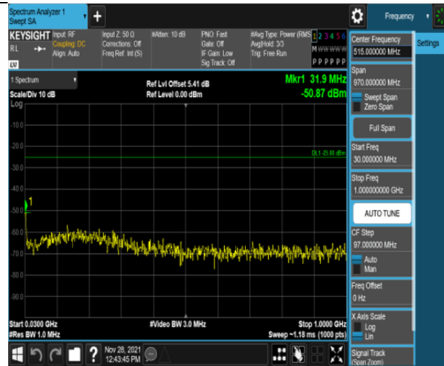
Band41-10MHz-16QAM-40620-50RB#0-Range1:30~1000MHz
