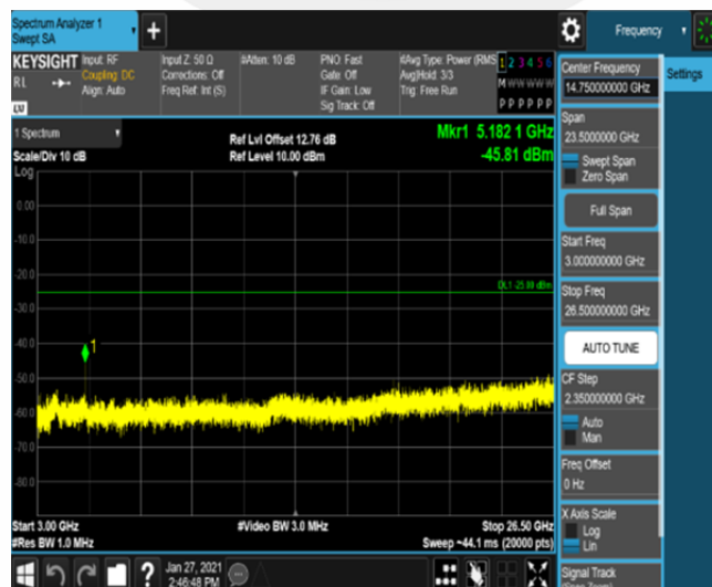
Band41-20MHz-16QAM-39750-100RB#0-Range3:3000~26500MHz
