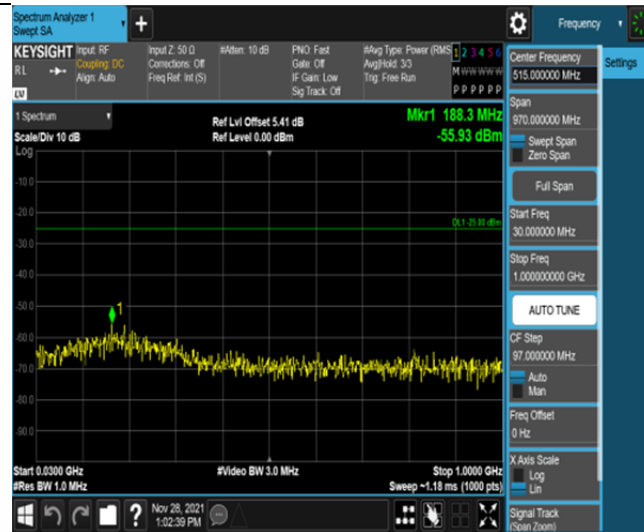
Band41-15MHz-QPSK-39725-75RB#0-Range1:30~1000MHz
