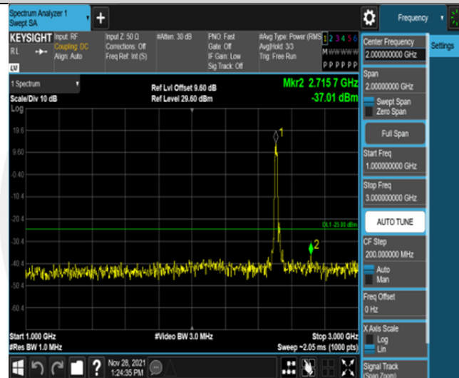
Band41-20MHz-16QAM-39750-100RB#0-Range2:1000~3000MHz
