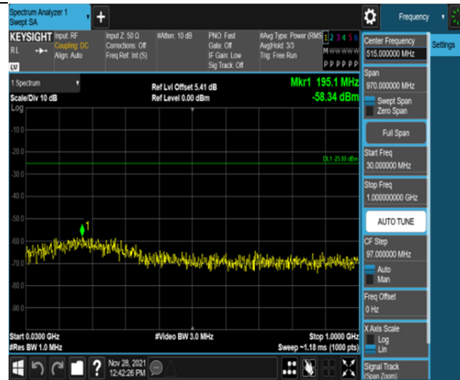
Band41-10MHz-16QAM-39700-50RB#0-Range1:30~1000MHz
