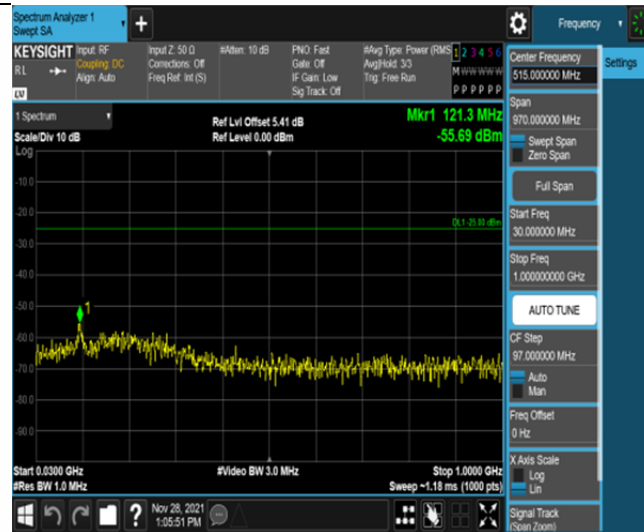
Band41-15MHz-16QAM-41515-75RB#0-Range1:30~1000MHz
