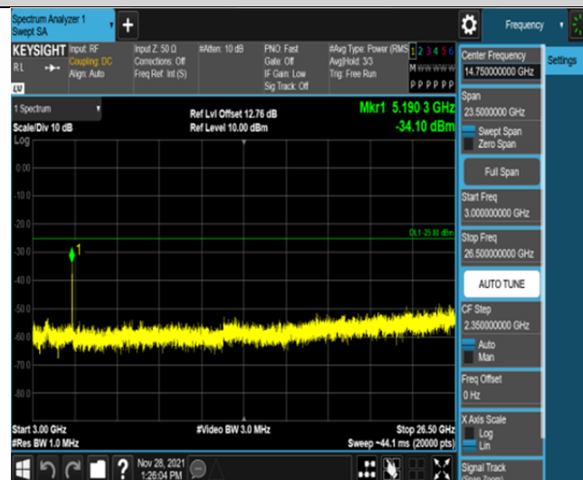
Band41-20MHz-16QAM-40620-100RB#0-Range3:3000~26500MHz
