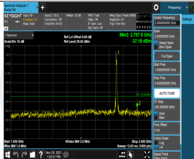
Band41-15MHz-QPSK-39725-75RB#0-Range2:1000~3000MHz
