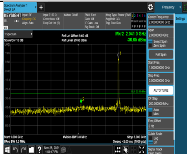
Band41-15MHz-16QAM-40620-75RB#0-Range2:1000~3000MHz
