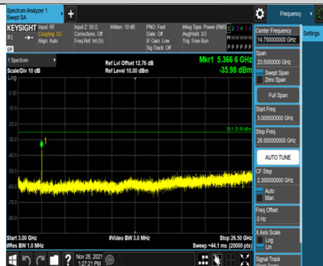
Band41-20MHz-16QAM-41490-100RB#0-Range3:3000~26500MHz
