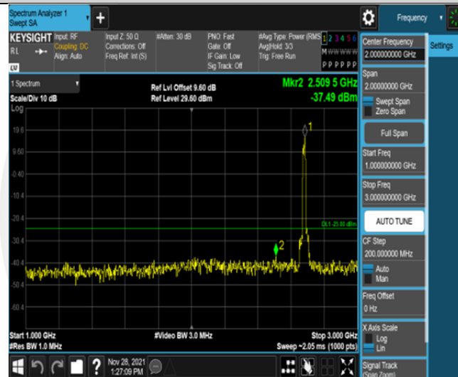
Band41-20MHz-16QAM-41490-100RB#0-Range2:1000~3000MHz
