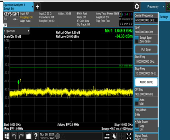
Band5-1.4MHz-16QAM-20407-6RB#0-Range2:1000~10000MHz
