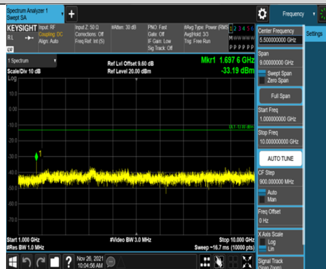
Band5-1.4MHz-16QAM-20643-6RB#0-Range2:1000~10000MHz
