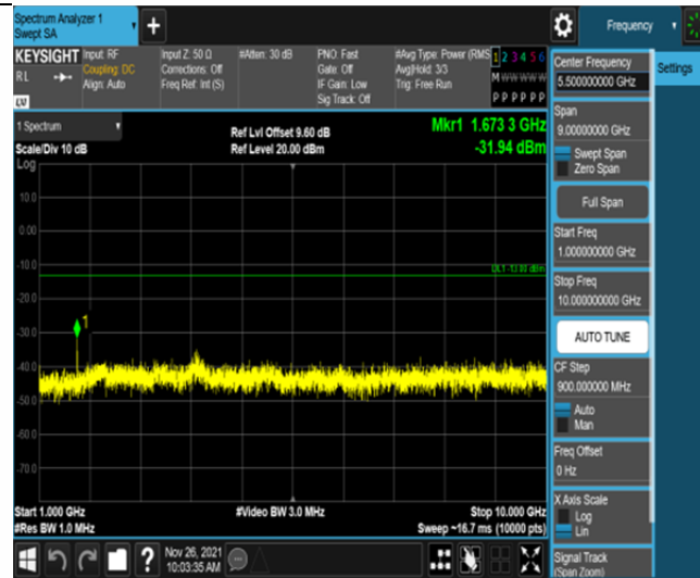
Band5-1.4MHz-QPSK-20525-6RB#0-Range2:1000~10000MHz
