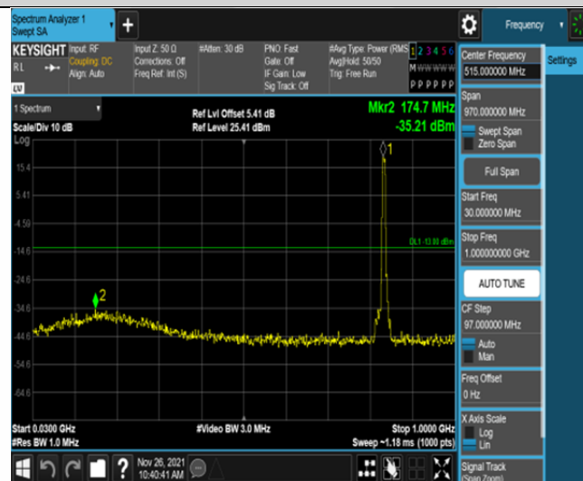
Band5-5MHz-QPSK-20525-25RB#0-Range1:30~1000MHz
