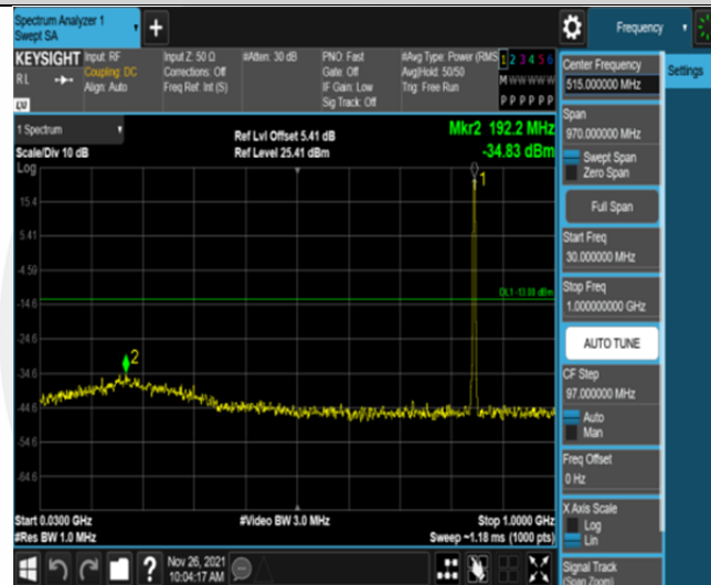
Band5-1.4MHz-QPSK-20643-6RB#0-Range1:30~1000MHz
