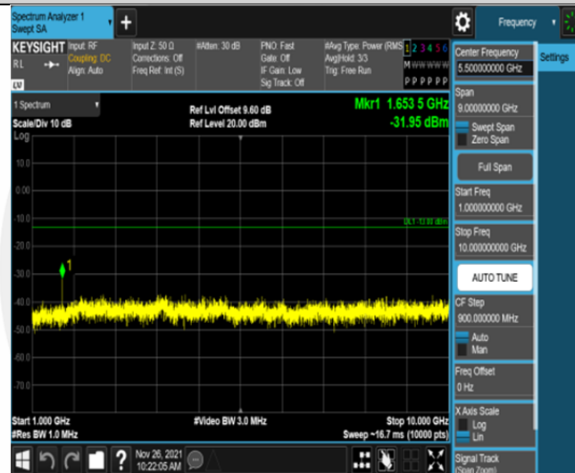
Band5-3MHz-16QAM-20415-15RB#0-Range2:1000~10000MHz
