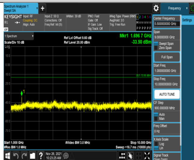
Band5-3MHz-QPSK-20635-15RB#0-Range2:1000~10000MHz
