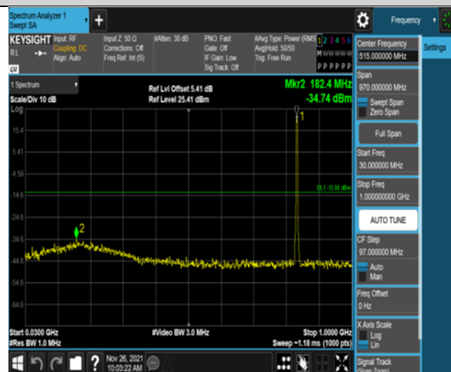
Band5-1.4MHz-QPSK-20525-6RB#0-Range1:30~1000MHz
