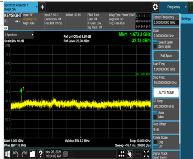
Band5-1.4MHz-16QAM-20525-6RB#0-Range2:1000~10000MHz
