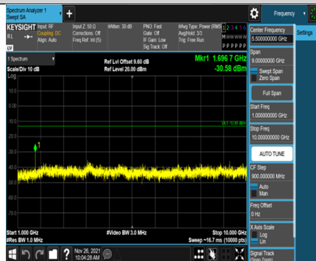
Band5-1.4MHz-QPSK-20643-6RB#0-Range2:1000~10000MHz
