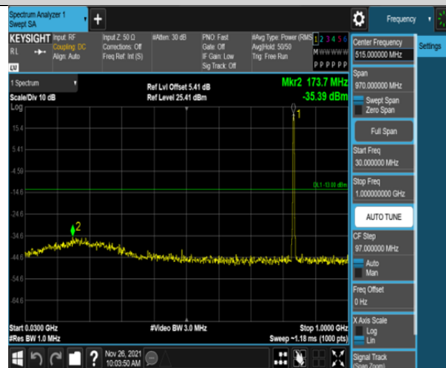
Band5-1.4MHz-16QAM-20525-6RB#0-Range1:30~1000MHz
