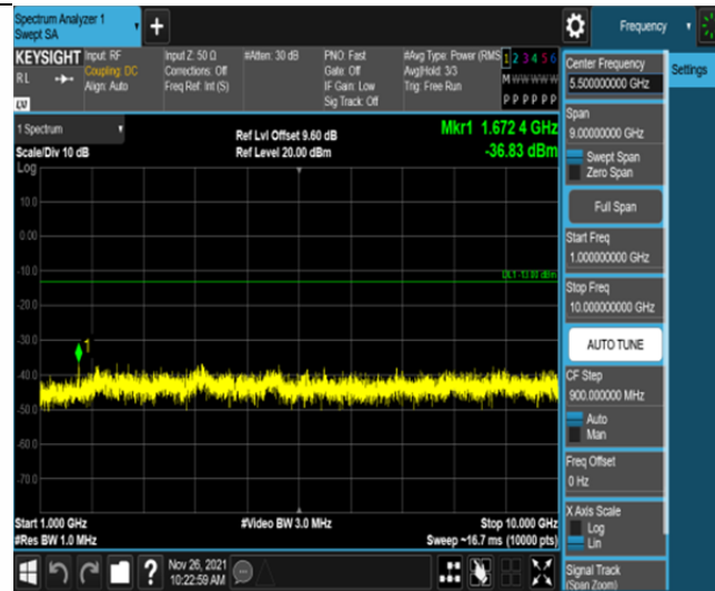
Band5-3MHz-16QAM-20525-15RB#0-Range2:1000~10000MHz
