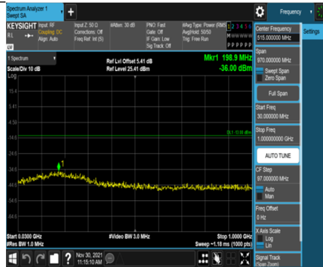
Band66-3MHz-16QAM-131987-15RB#0-Range1:30~1000MHz
