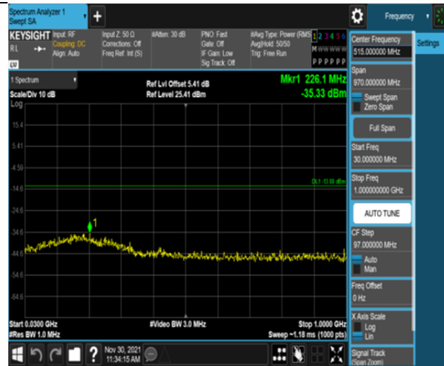
Band66-5MHz-QPSK-131997-25RB#0-Range1:30~1000MHz
