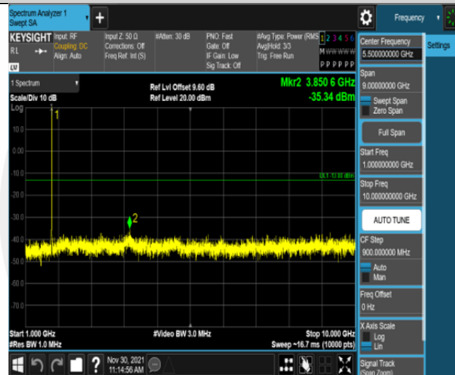
Band66-3MHz-QPSK-131987-15RB#0-Range2:1000~10000MHz
