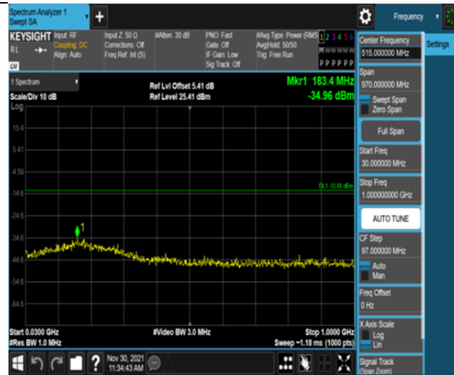
Band66-5MHz-16QAM-131997-25RB#0-Range1:30~1000MHz
