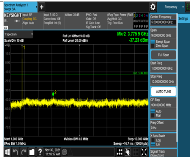
Band66-3MHz-16QAM-132322-15RB#0-Range2:1000~10000MHz
