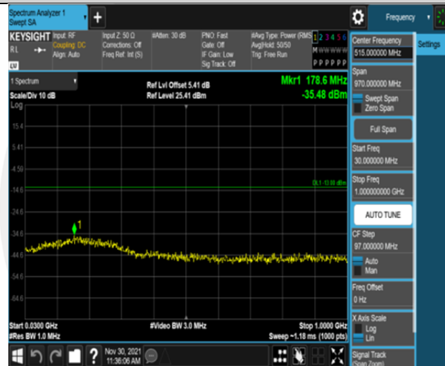
Band66-5MHz-QPSK-132647-25RB#0-Range1:30~1000MHz
