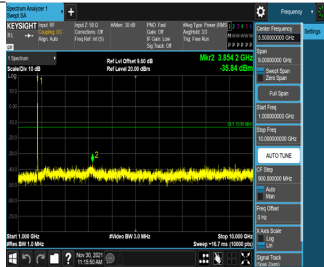
Band66-3MHz-QPSK-132322-15RB#0-Range2:1000~10000MHz
