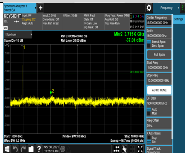
Band66-5MHz-QPSK-132647-25RB#0-Range2:1000~10000MHz
