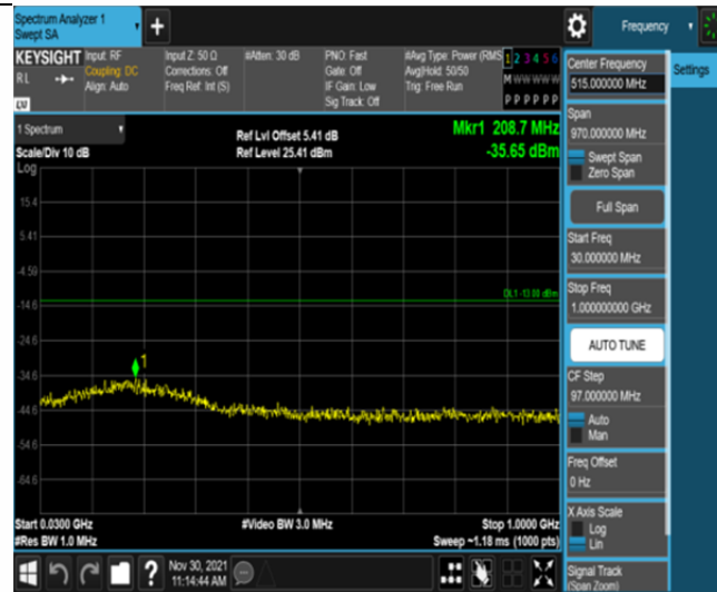
Band66-3MHz-QPSK-131987-15RB#0-Range1:30~1000MHz
