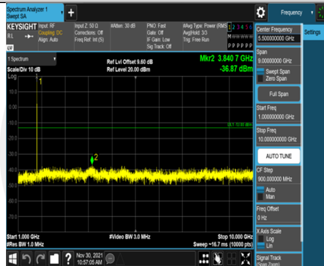
Band66-1.4MHz-16QAM-131979-6RB#0-Range2:1000~10000MHz
