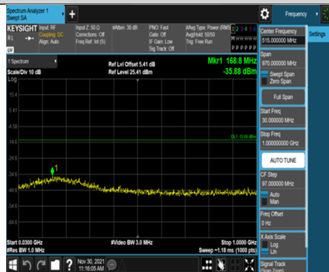
Band66-3MHz-16QAM-132322-15RB#0-Range1:30~1000MHz
