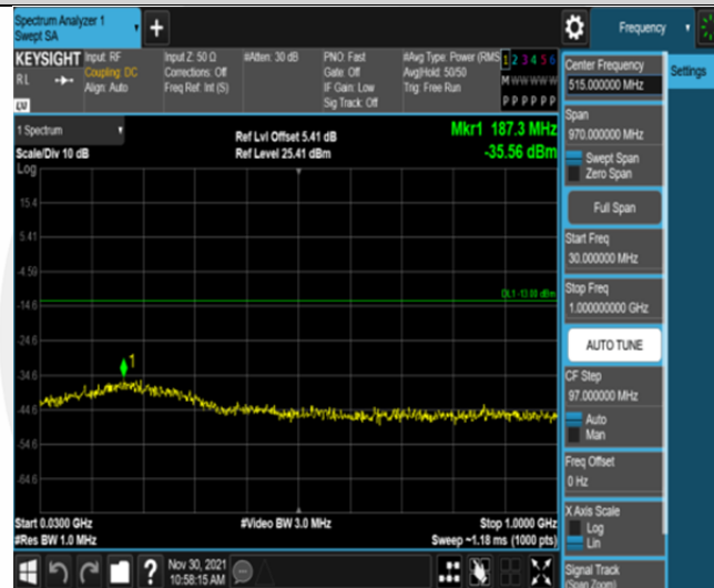
Band66-1.4MHz-QPSK-132665-6RB#0-Range1:30~1000MHz
