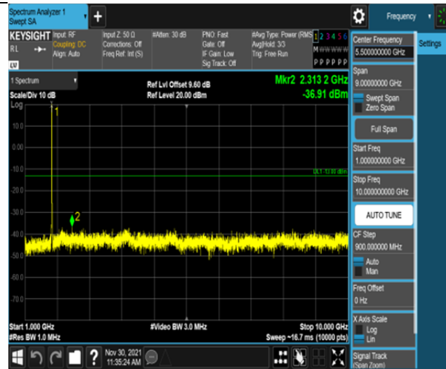
Band66-5MHz-QPSK-132322-25RB#0-Range2:1000~10000MHz
