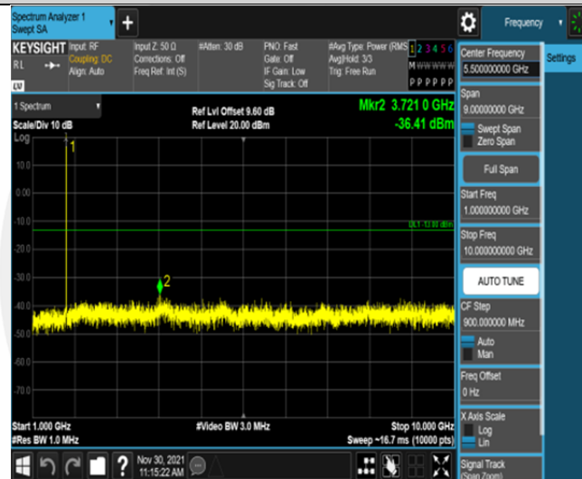
Band66-3MHz-16QAM-131987-15RB#0-Range2:1000~10000MHz
