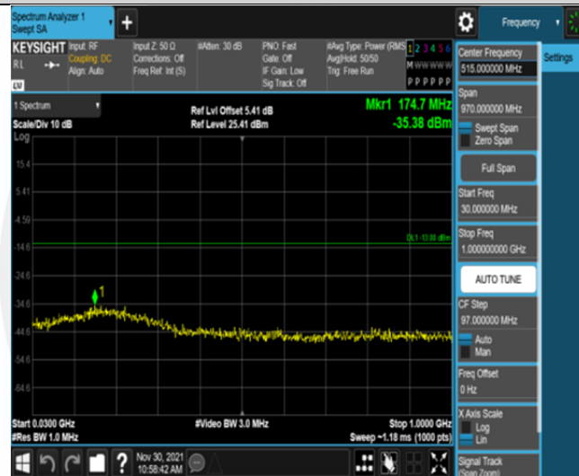
Band66-1.4MHz-16QAM-132665-6RB#0-Range1:30~1000MHz
