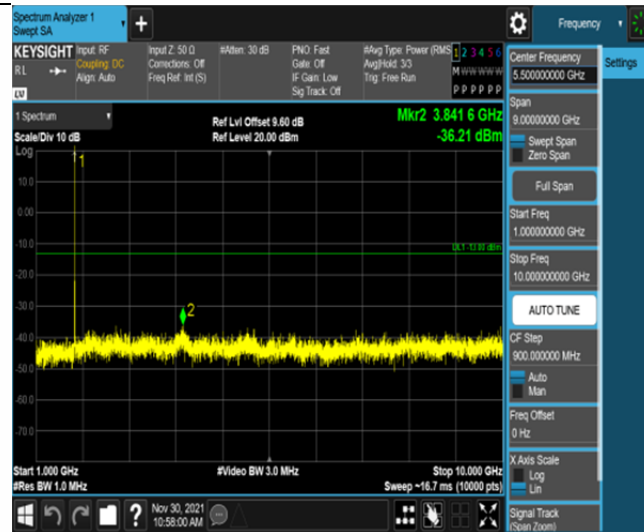
Band66-1.4MHz-16QAM-132322-6RB#0-Range2:1000~10000MHz
