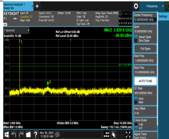
Band66-5MHz-16QAM-132322-25RB#0-Range2:1000~10000MHz
