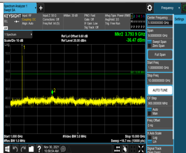
Band66-1.4MHz-16QAM-132665-6RB#0-Range2:1000~10000MHz
