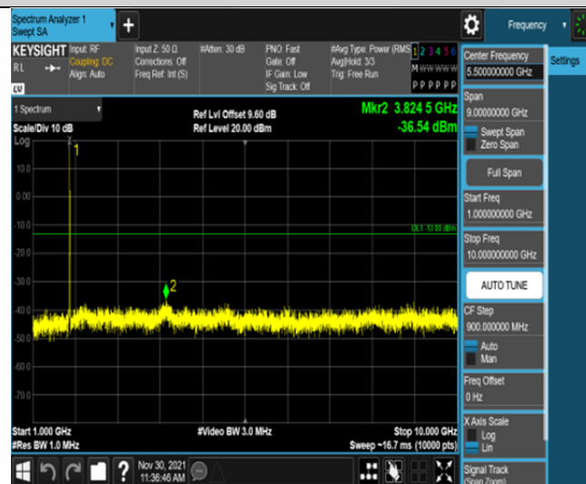
Band66-5MHz-16QAM-132647-25RB#0-Range2:1000~10000MHz
