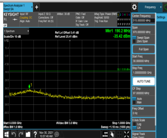
Band66-1.4MHz-16QAM-132322-6RB#0-Range1:30~1000MHz
