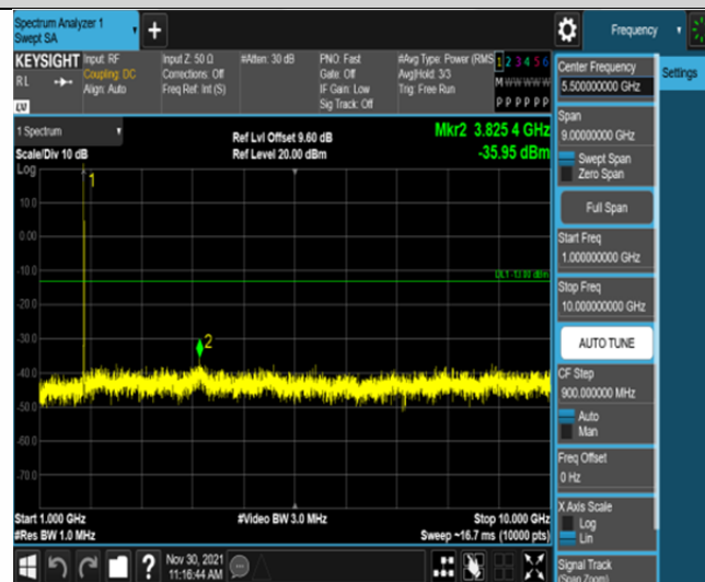
Band66-3MHz-QPSK-132657-15RB#0-Range2:1000~10000MHz
