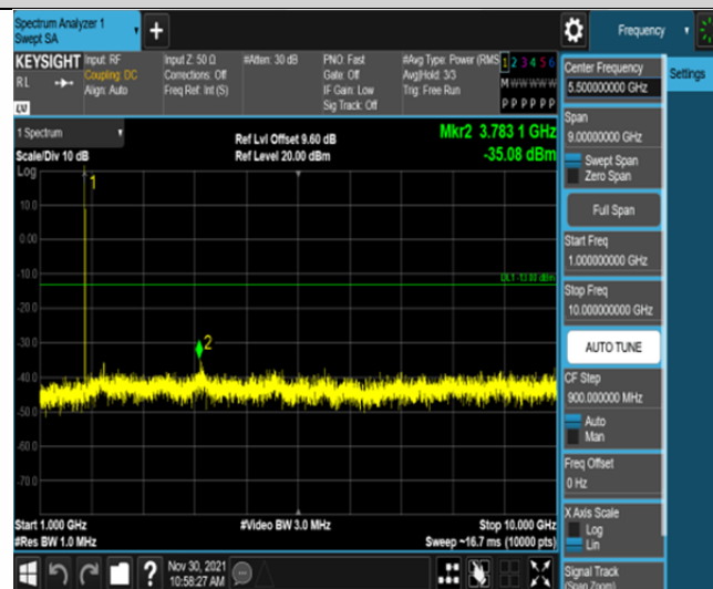
Band66-1.4MHz-QPSK-132665-6RB#0-Range2:1000~10000MHz
