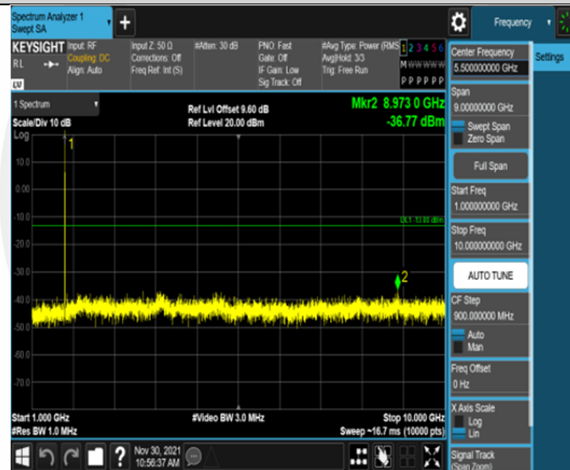
Band66-1.4MHz-QPSK-131979-6RB#0-Range2:1000~10000MHz
