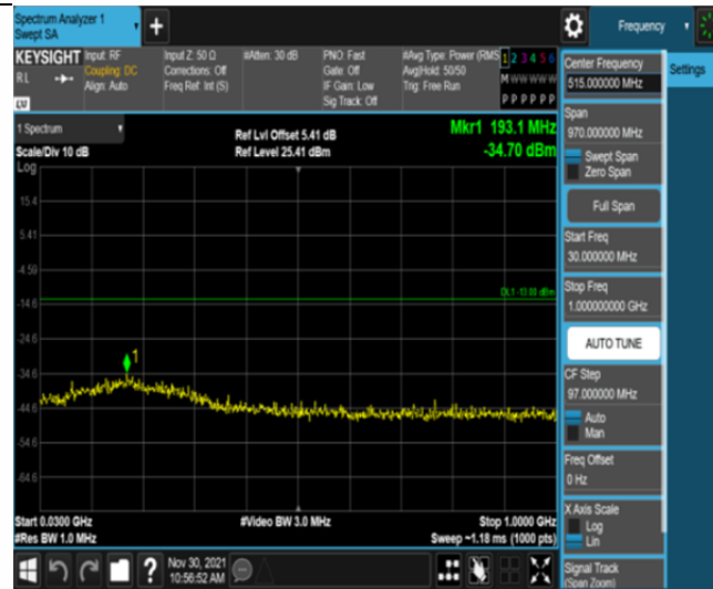
Band66-1.4MHz-16QAM-131979-6RB#0-Range1:30~1000MHz
