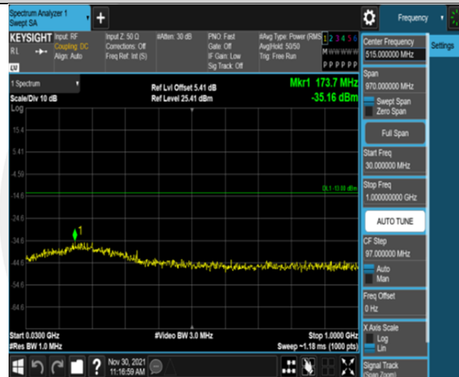
Band66-3MHz-16QAM-132657-15RB#0-Range1:30~1000MHz
