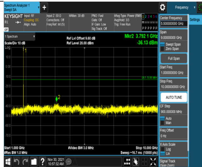
Band66-1.4MHz-QPSK-132322-6RB#0-Range2:1000~10000MHz
