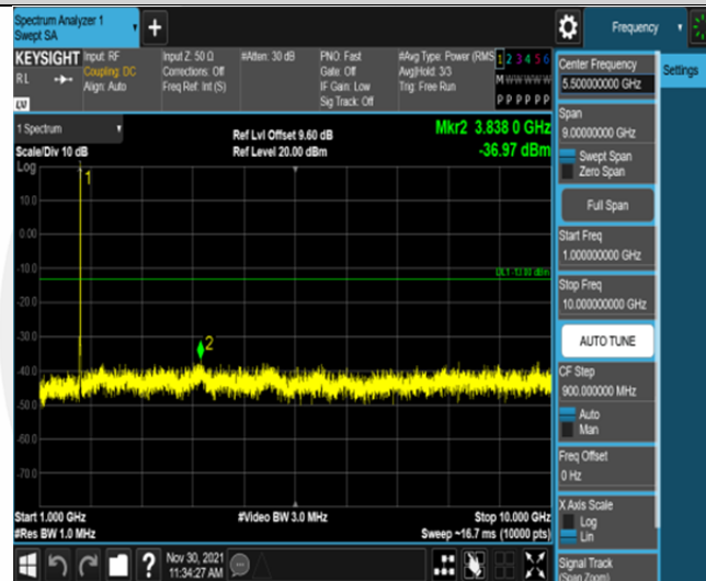
Band66-5MHz-QPSK-131997-25RB#0-Range2:1000~10000MHz
