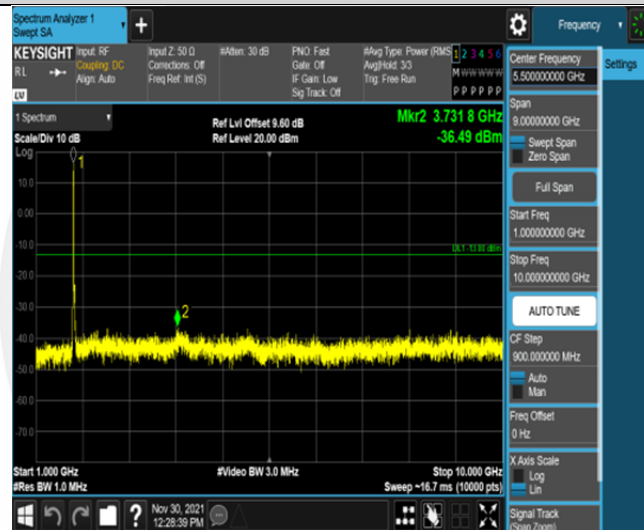
Band66-20MHz-16QAM-132072-100RB#0-Range2:1000~10000MHz
