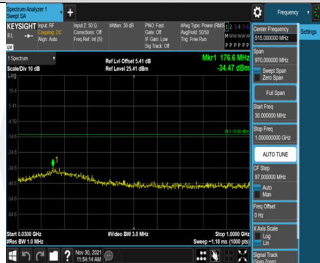
Band66-10MHz-16QAM-132622-50RB#0-Range1:30~1000MHz
