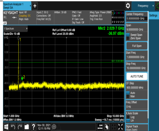
Band66-15MHz-16QAM-132322-75RB#0-Range2:1000~10000MHz
