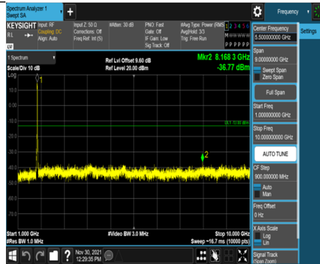
Band66-20MHz-16QAM-132322-100RB#0-Range2:1000~10000MHz
