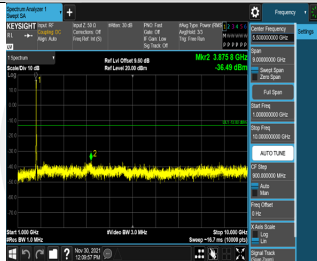
Band66-15MHz-QPSK-132047-75RB#0-Range2:1000~10000MHz
