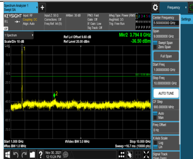
Band66-15MHz-16QAM-132047-75RB#0-Range2:1000~10000MHz
