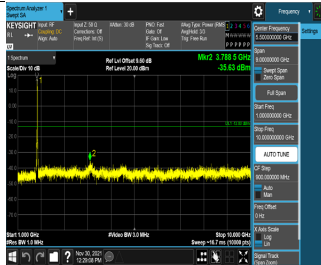
Band66-20MHz-QPSK-132322-100RB#0-Range2:1000~10000MHz
