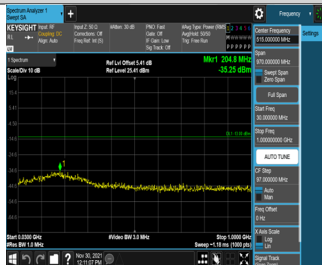
Band66-15MHz-16QAM-132322-75RB#0-Range1:30~1000MHz
