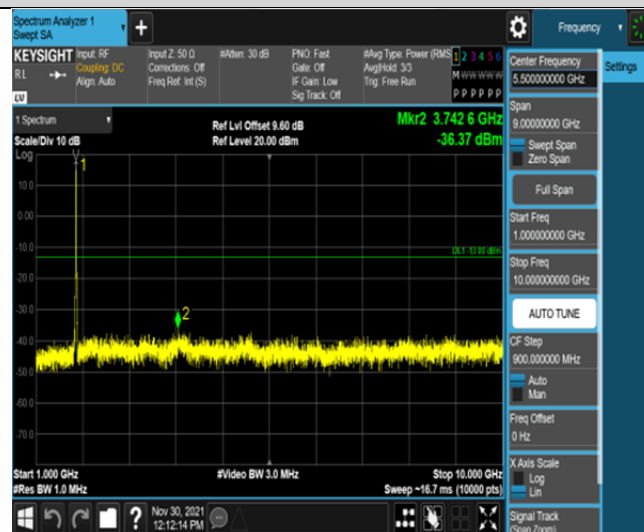
Band66-15MHz-16QAM-132597-75RB#0-Range2:1000~10000MHz
