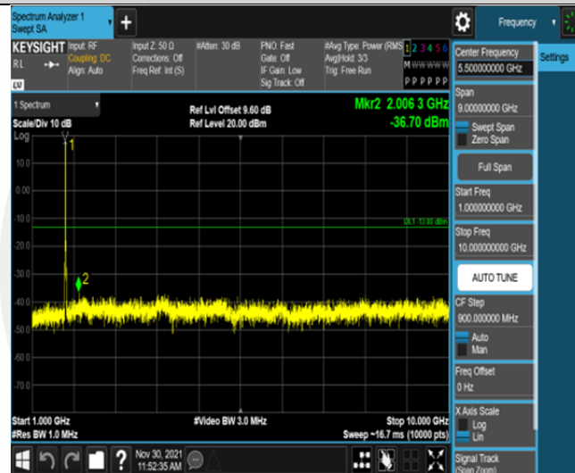
Band66-10MHz-16QAM-132022-50RB#0-Range2:1000~10000MHz
