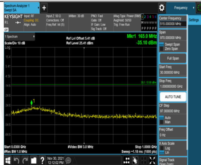
Band66-15MHz-16QAM-132597-75RB#0-Range1:30~1000MHz
