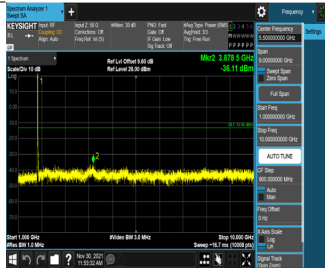
Band66-10MHz-16QAM-132322-50RB#0-Range2:1000~10000MHz
