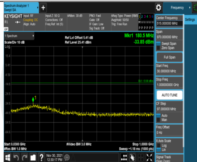
Band66-20MHz-16QAM-132572-100RB#0-Range1:30~1000MHz
