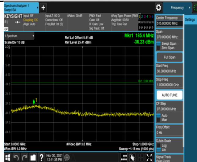
Band66-15MHz-QPSK-132597-75RB#0-Range1:30~1000MHz
