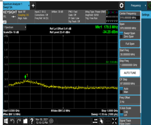
Band66-15MHz-16QAM-132047-75RB#0-Range1:30~1000MHz
