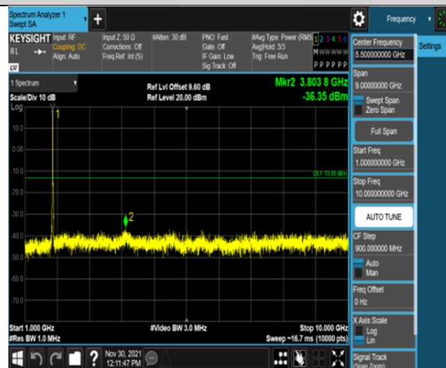
Band66-15MHz-QPSK-132597-75RB#0-Range2:1000~10000MHz
