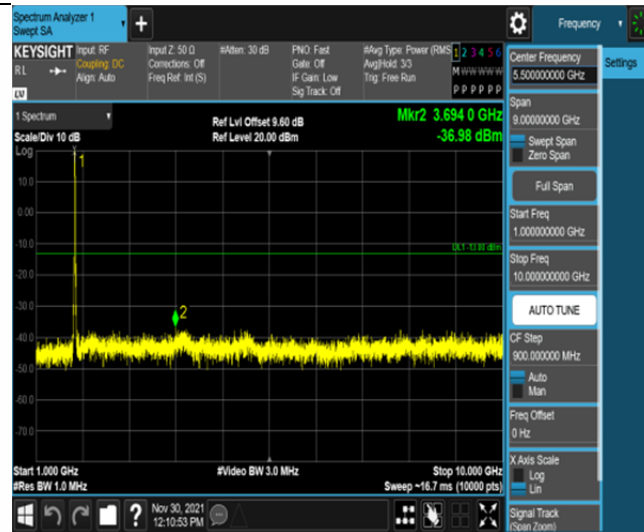
Band66-15MHz-QPSK-132322-75RB#0-Range2:1000~10000MHz
