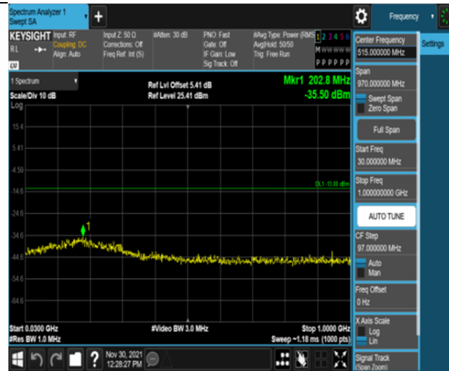
Band66-20MHz-16QAM-132072-100RB#0-Range1:30~1000MHz
