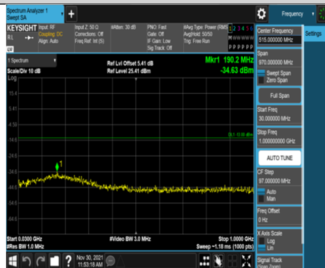
Band66-10MHz-16QAM-132322-50RB#0-Range1:30~1000MHz
