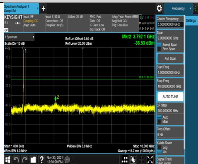
Band66-20MHz-16QAM-132572-100RB#0-Range2:1000~10000MHz
