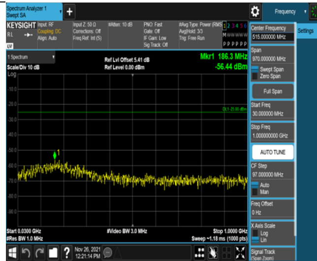
Band7-5MHz-QPSK-21425-25RB#0-Range1:30~1000MHz
