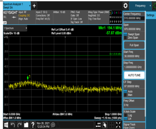
Band7-5MHz-16QAM-21100-25RB#0-Range1:30~1000MHz
