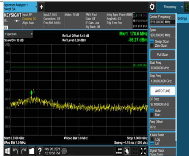
Band7-5MHz-QPSK-21100-25RB#0-Range1:30~1000MHz
