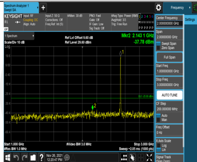
Band7-5MHz-16QAM-21100-25RB#0-Range2:1000~3000MHz
