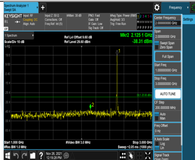
Band7-5MHz-16QAM-20775-25RB#0-Range2:1000~3000MHz
