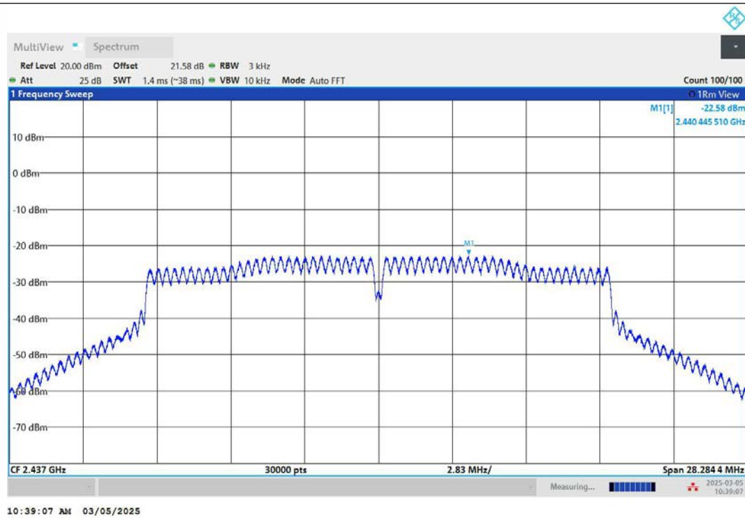
11N20MIMO-Ant2-2437-PASS
