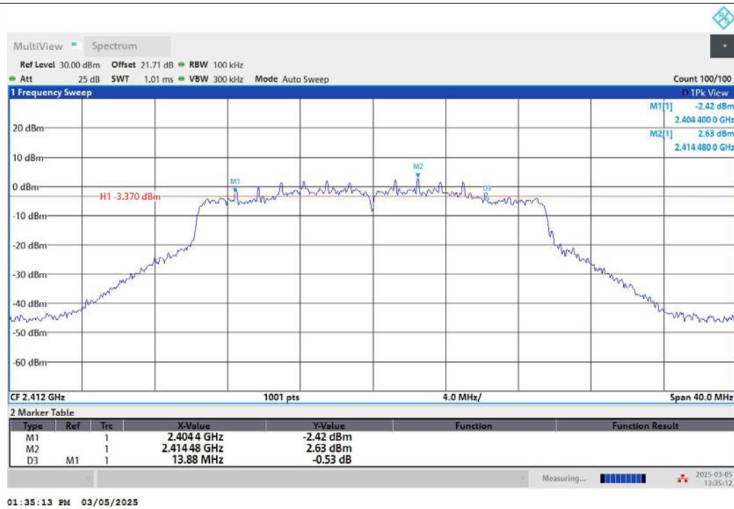
11AX20MIMO-Ant2-2412-PASS
