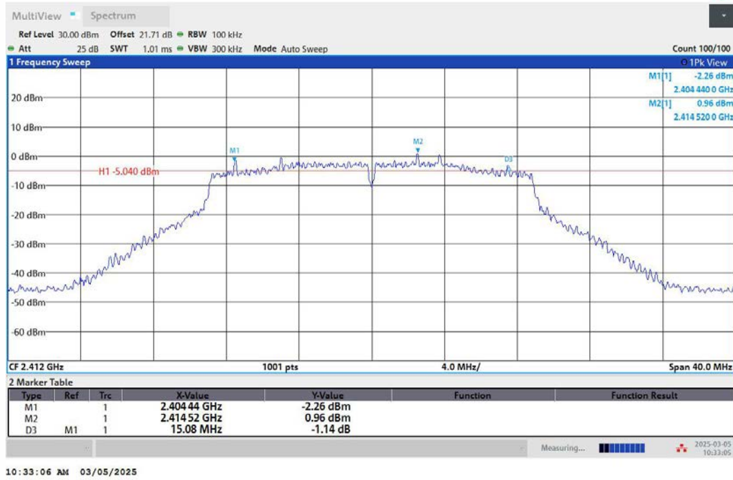
11N20MIMO-Ant2-2412-PASS
