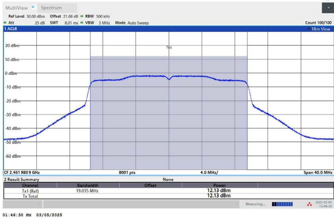
11AX20MIMO-Ant2-2462-PASS
