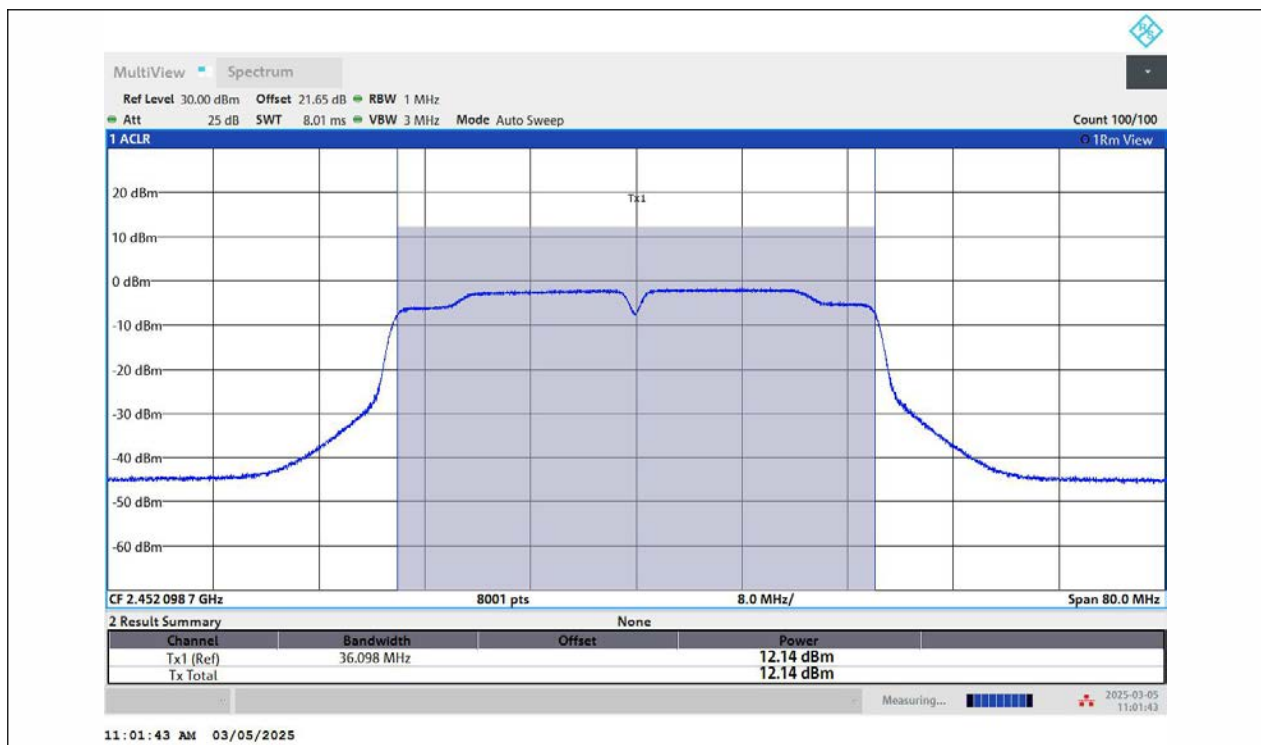
11N40MIMO-Ant2-2452-PASS
