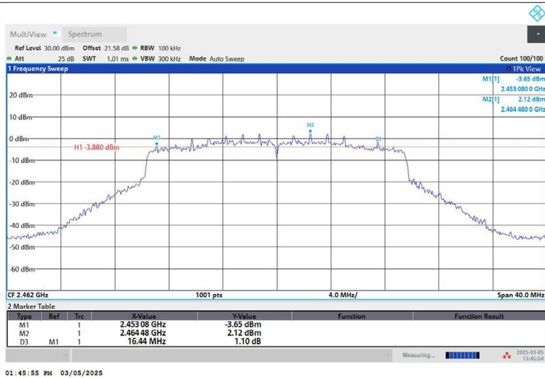
11AX20MIMO-Ant2-2462-PASS
