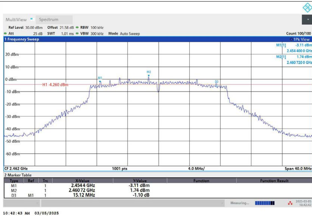
11N20MIMO-Ant2-2462-PASS
