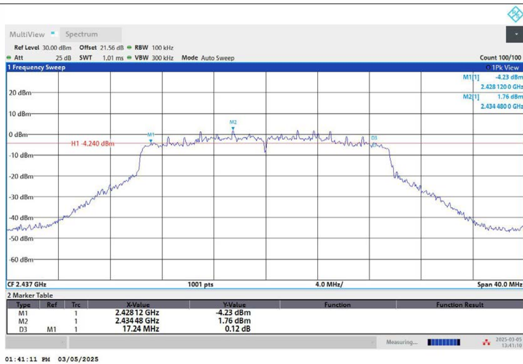
11AX20MIMO-Ant2-2437-PASS
