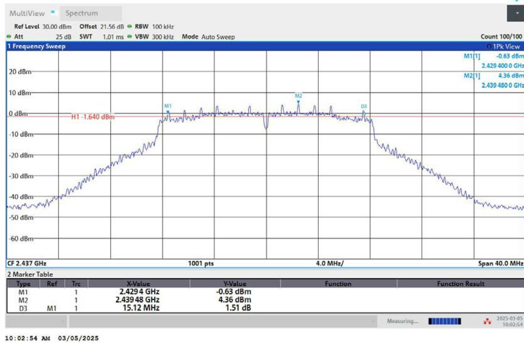
11G-Ant2-2437-PASS
