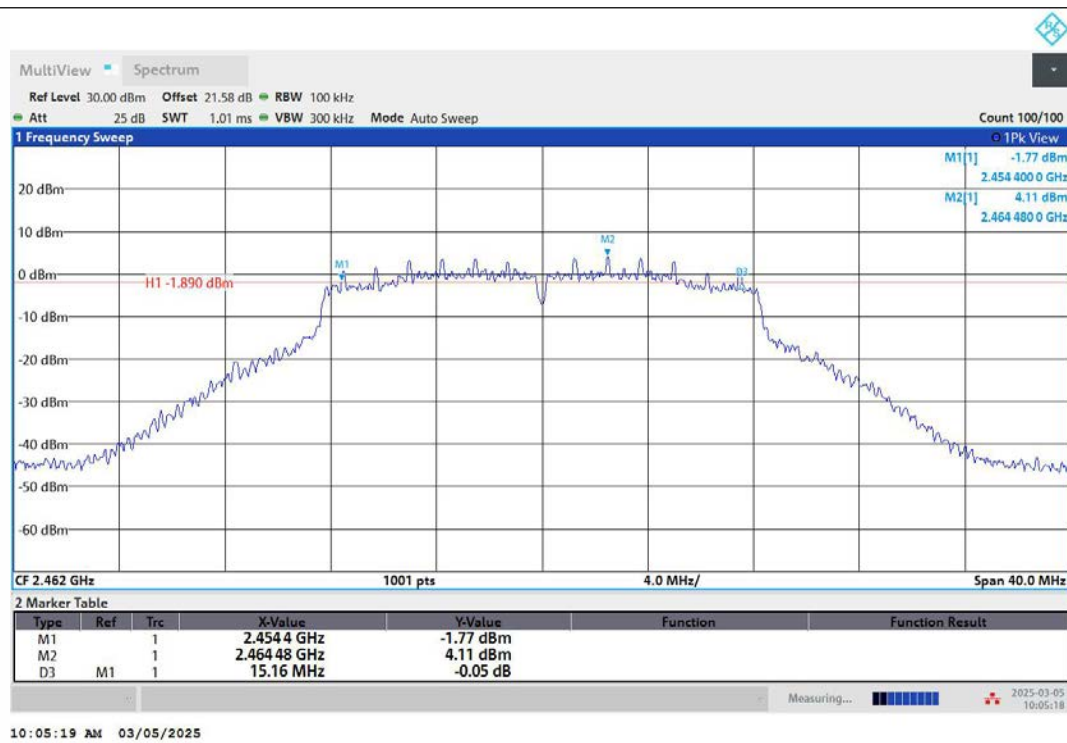
11G-Ant2-2462-PASS
