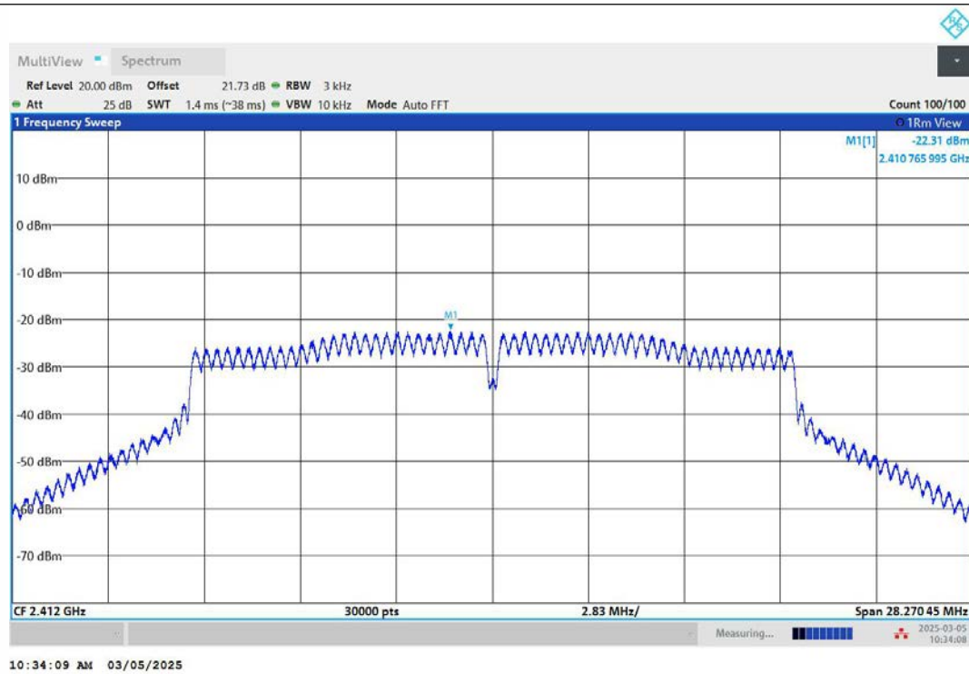
11N20MIMO-Ant2-2412-PASS
