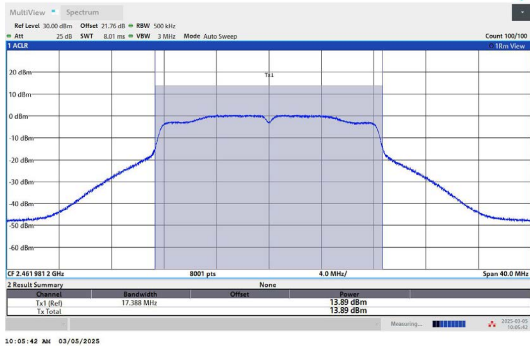
11G-Ant2-2462-PASS
