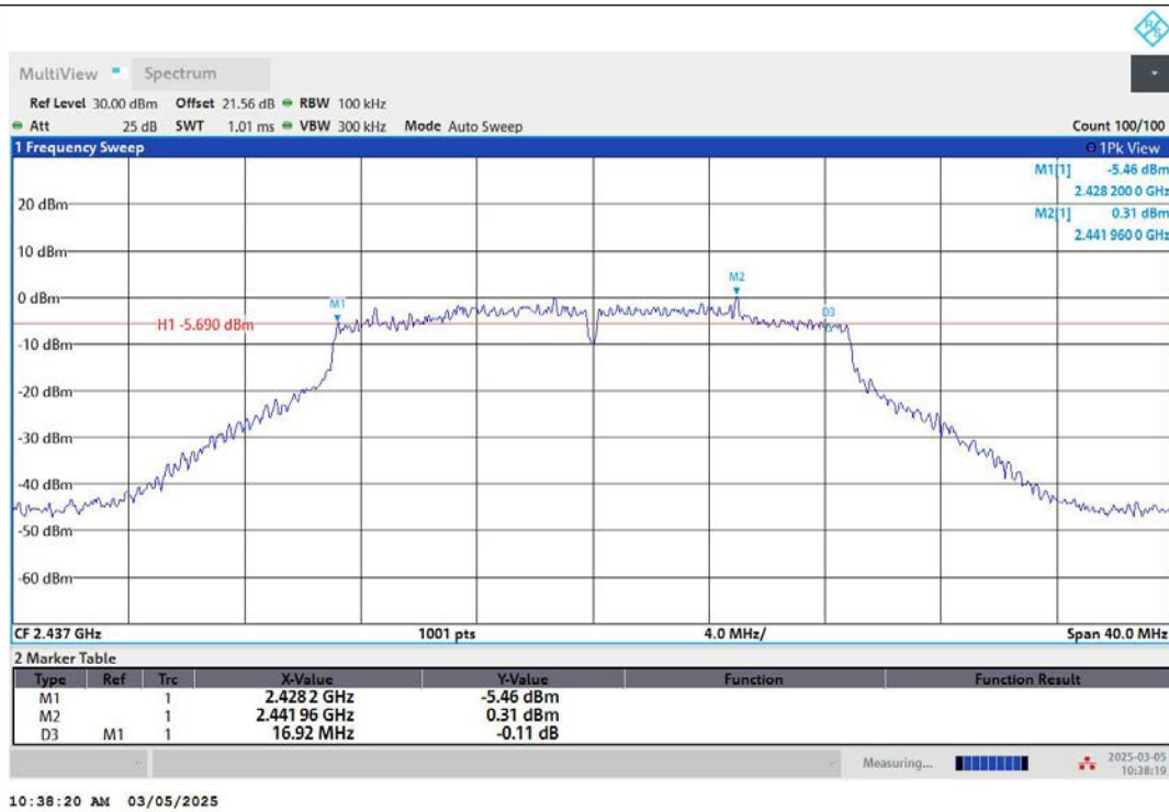
11N20MIMO-Ant2-2437-PASS
