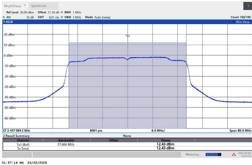
11AX40MIMO-Ant2-2437-PASS
