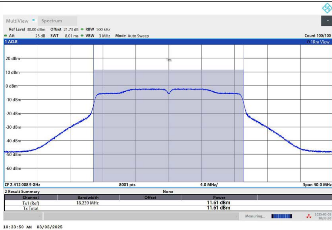
11N20MIMO-Ant2-2412-PASS
