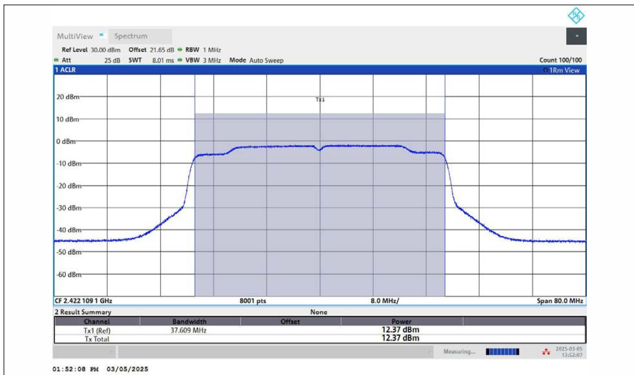
11AX40MIMO-Ant2-2422-PASS
