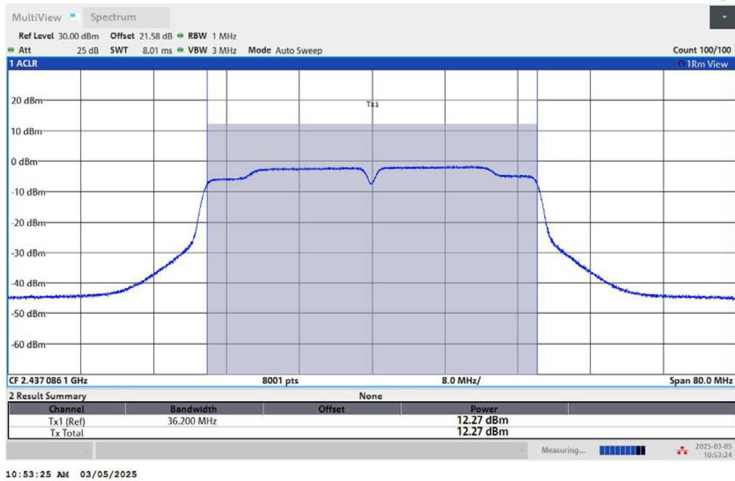
11N40MIMO-Ant2-2437-PASS
