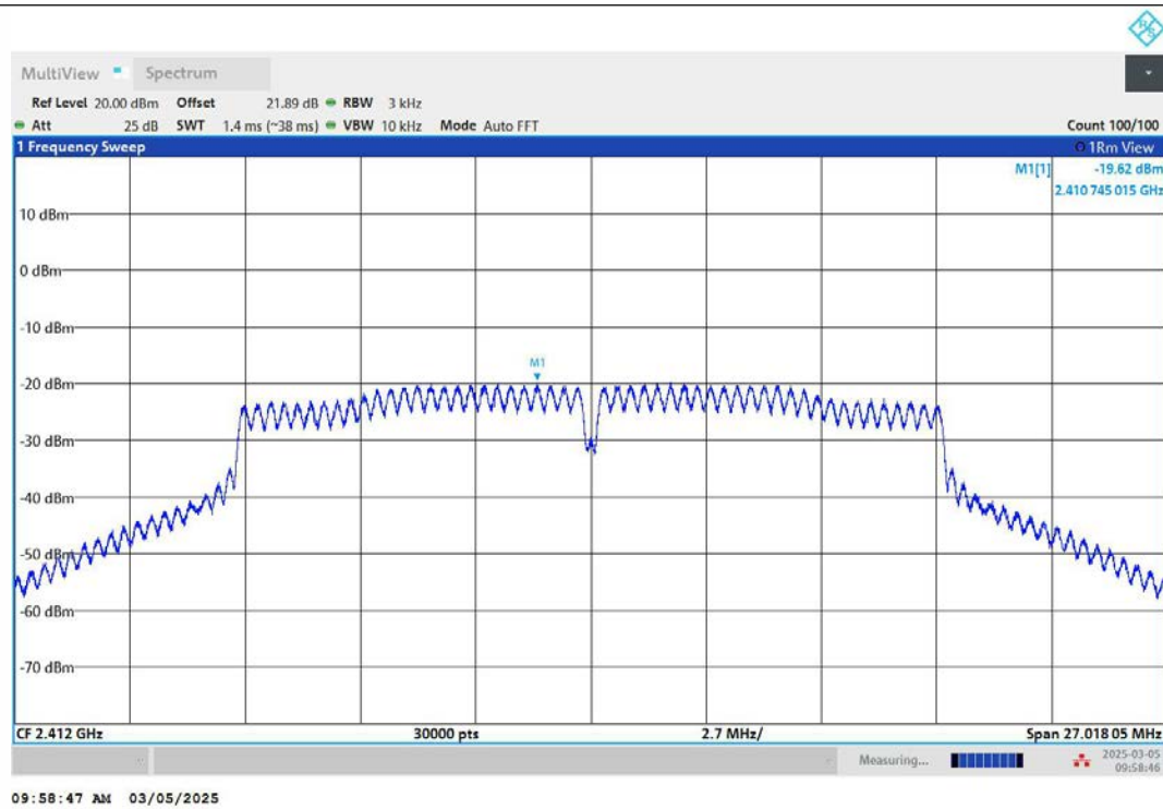
11G-Ant2-2412-PASS
