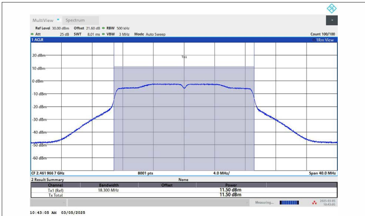
11N20MIMO-Ant2-2462-PASS
