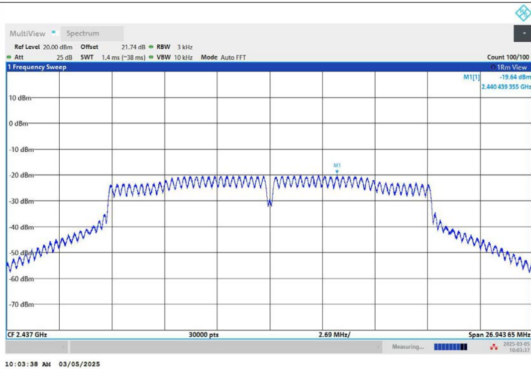
11G-Ant2-2437-PASS
