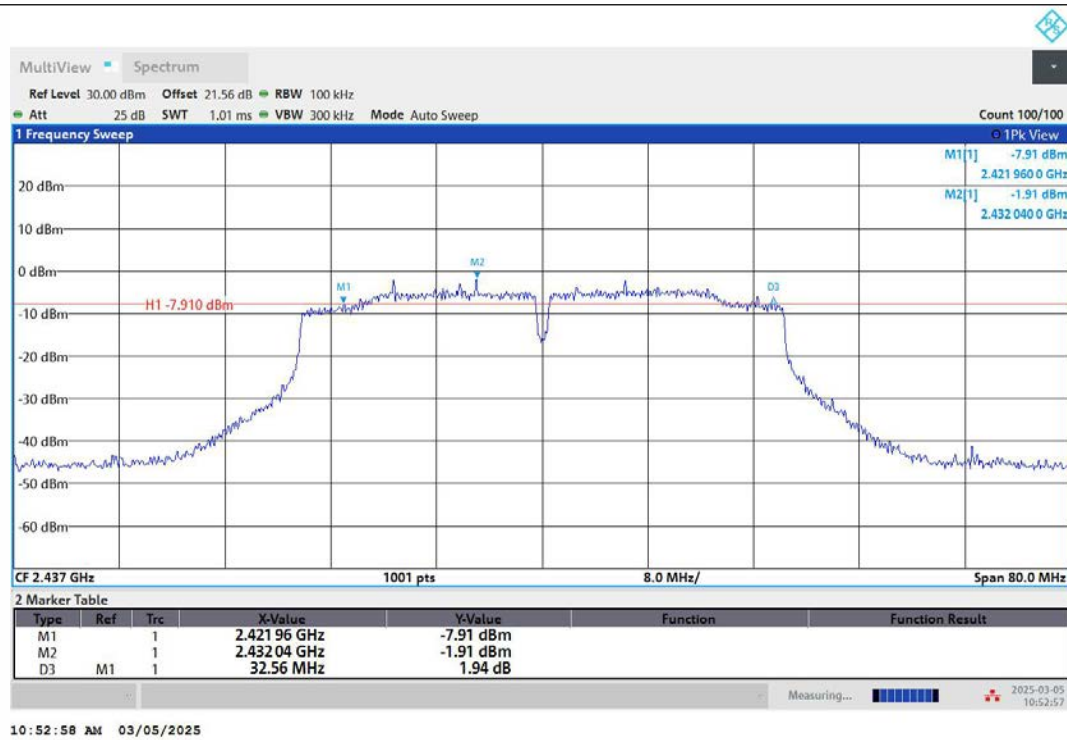
11N40MIMO-Ant2-2437-PASS
