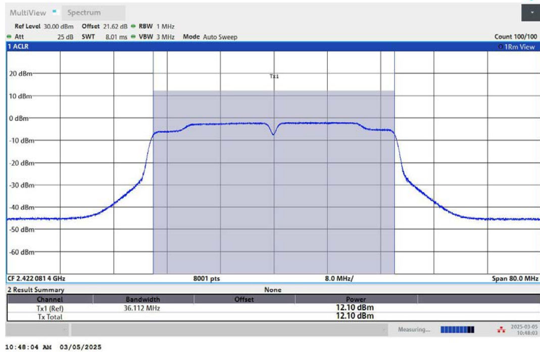
11N40MIMO-Ant2-2422-PASS
