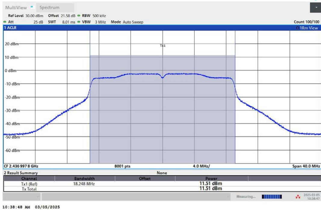
11N20MIMO-Ant2-2437-PASS
