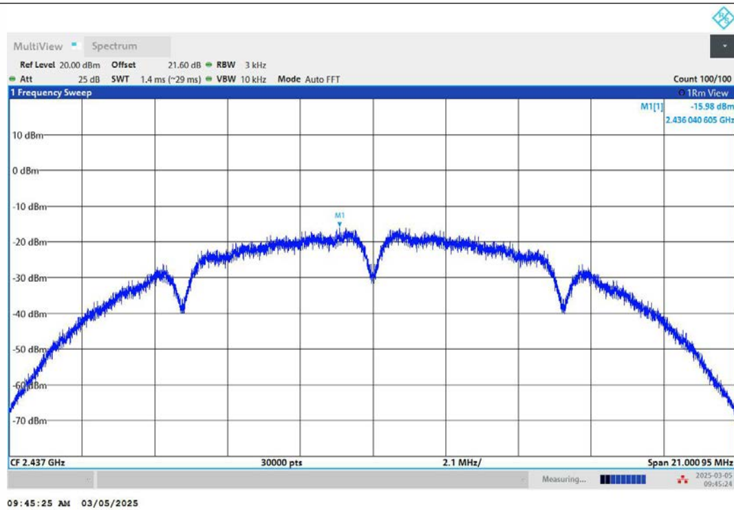
11B-Ant2-2437-PASS
