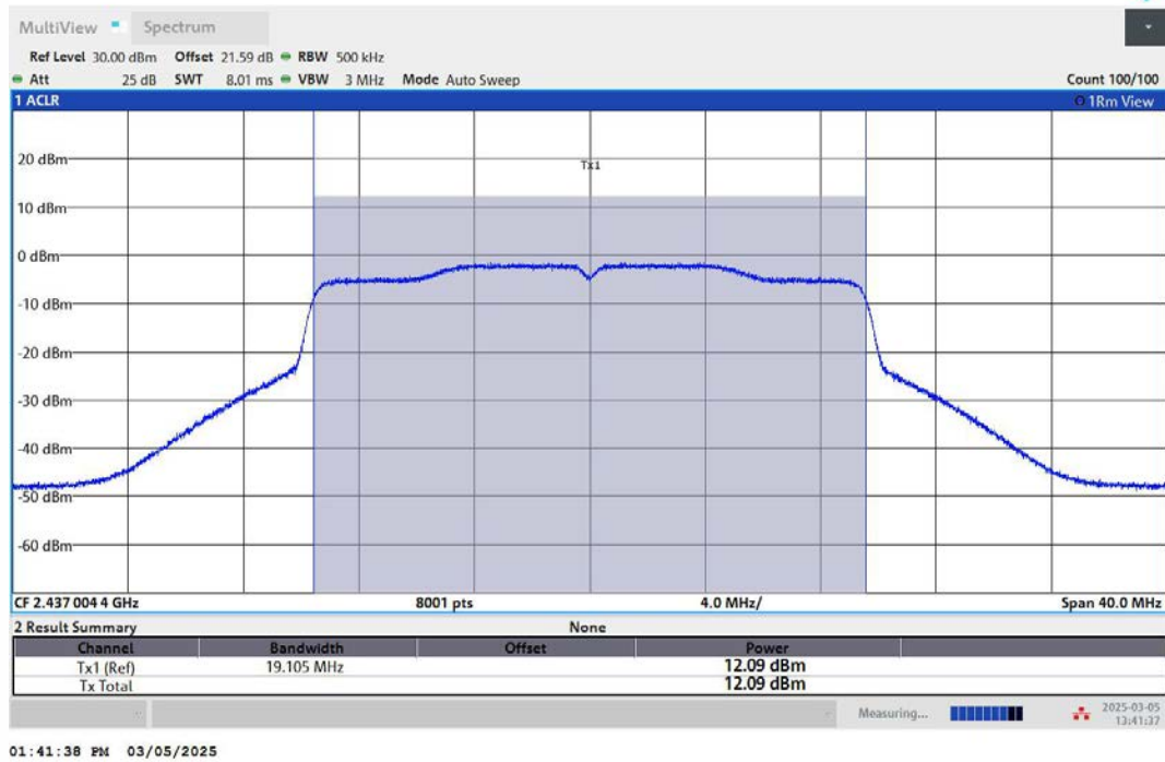
11AX20MIMO-Ant2-2437-PASS
