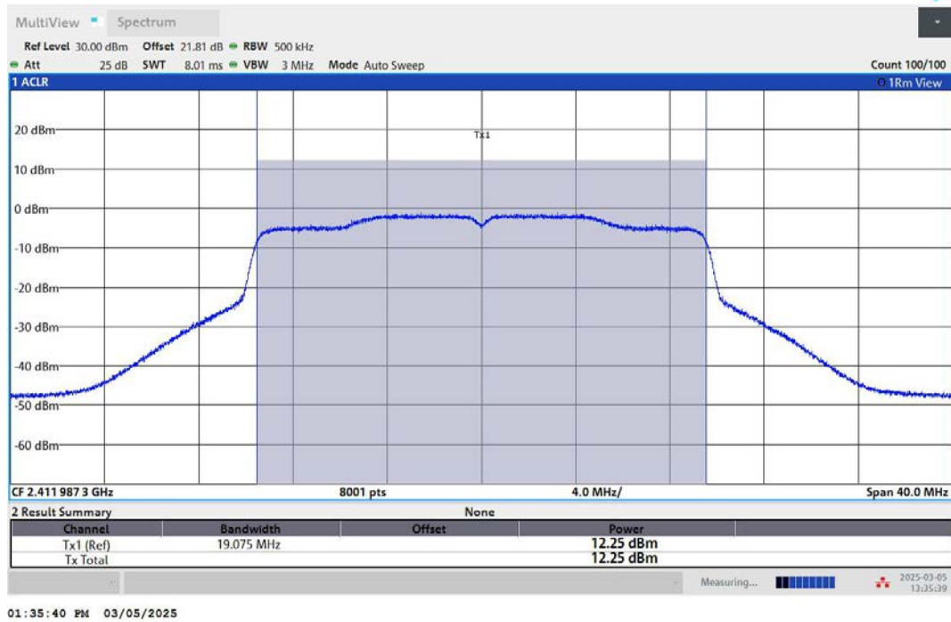
11AX20MIMO-Ant2-2412-PASS
