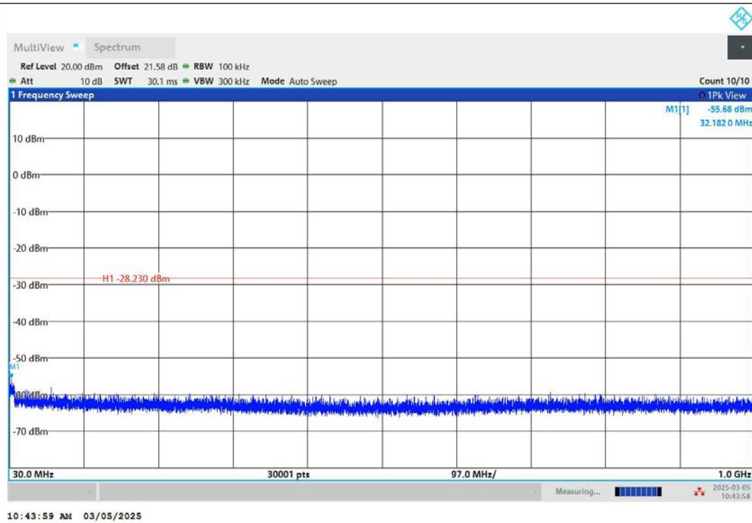
11N20MIMO-Ant2-2462-30~1000-PASS
