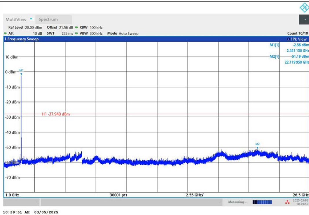
11N20MIMO-Ant2-2437-1000~26500-PASS
