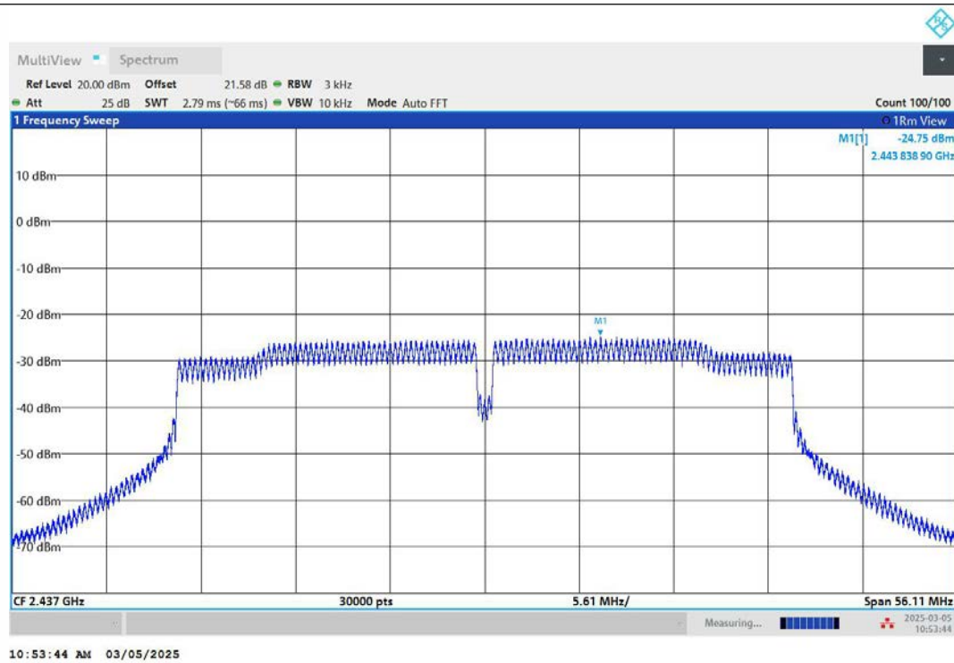
11N40MIMO-Ant2-2437-PASS
