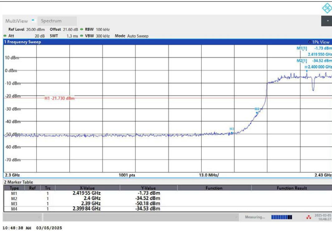
11N40MIMO-Ant2-2422-PASS
