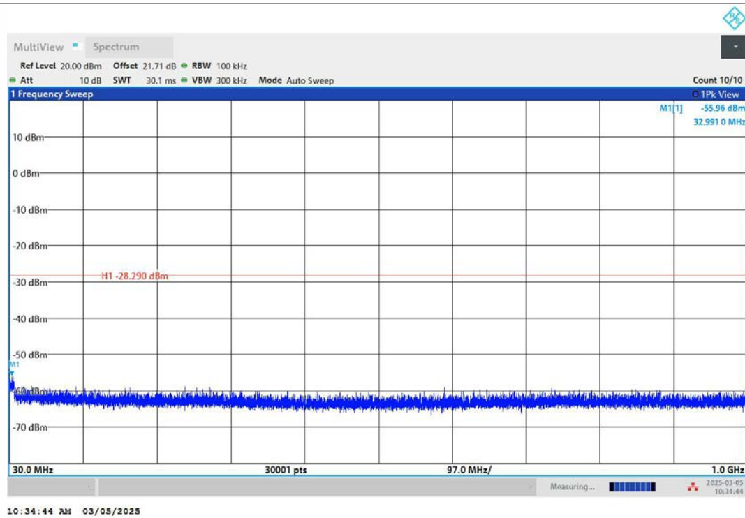
11N20MIMO-Ant2-2412-30~1000-PASS
