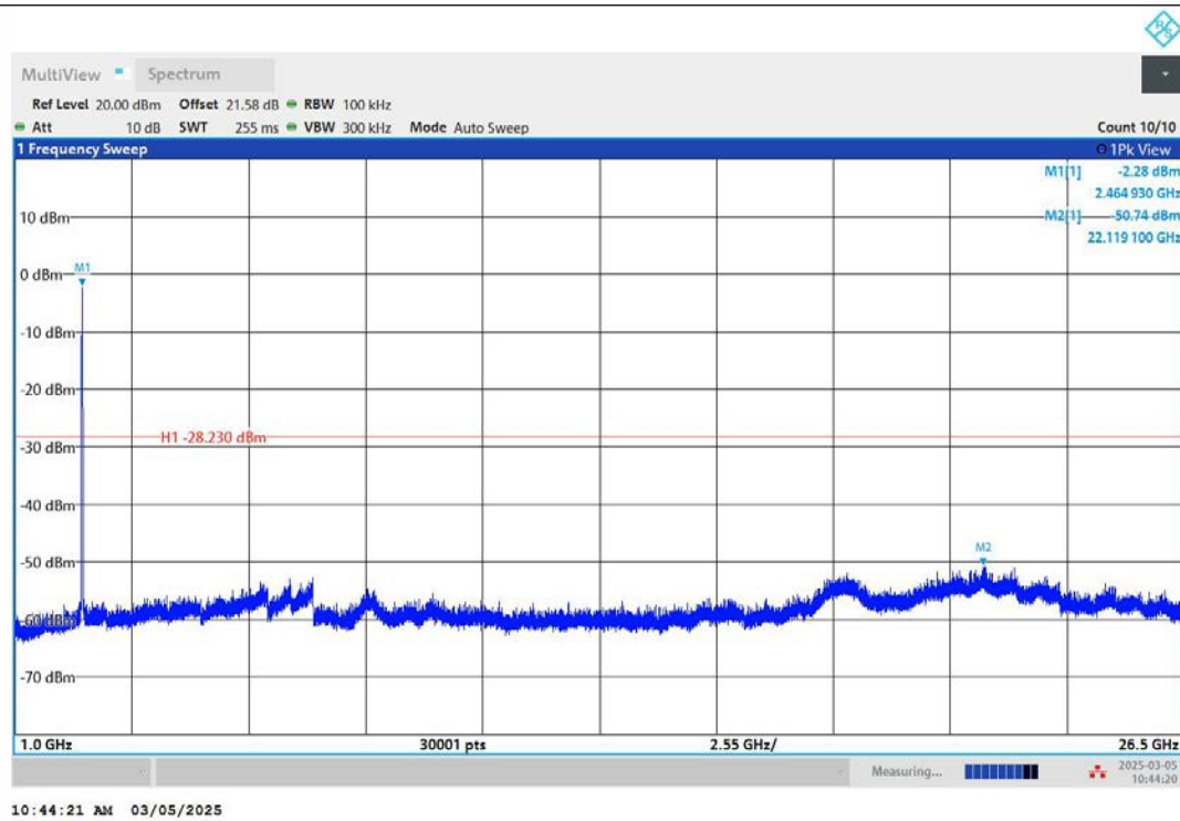
11N20MIMO-Ant2-2462-1000~26500-PASS
