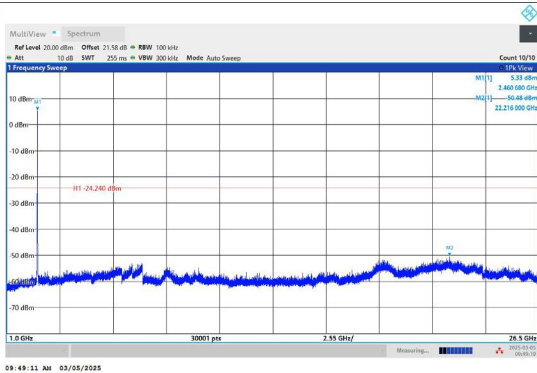
11B-Ant2-2462-1000~26500-PASS
