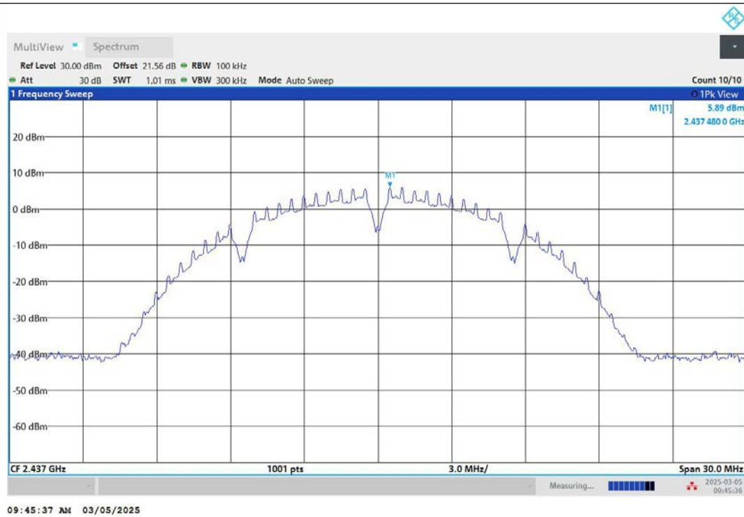
11B-Ant2-2437-0~Reference-PASS
