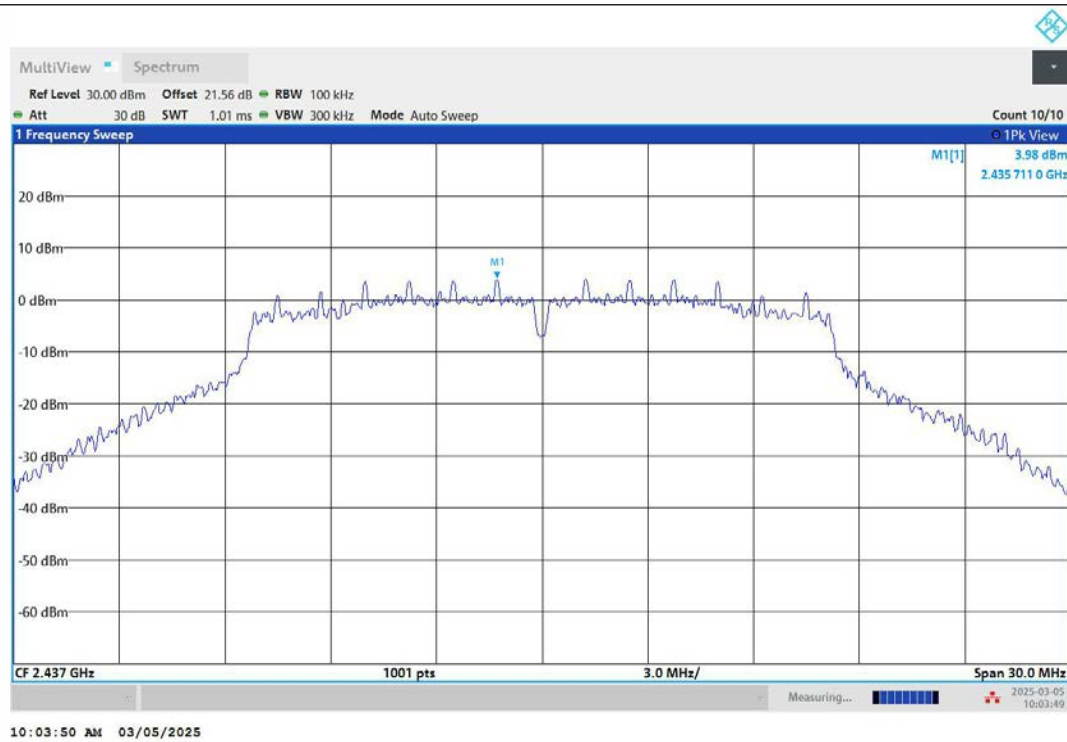
11G-Ant2-2437-0~Reference-PASS
