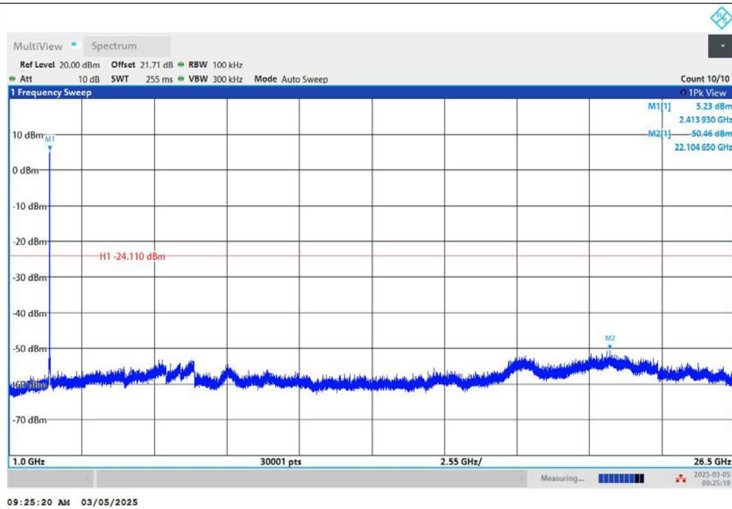
11B-Ant2-2412-1000~26500-PASS
