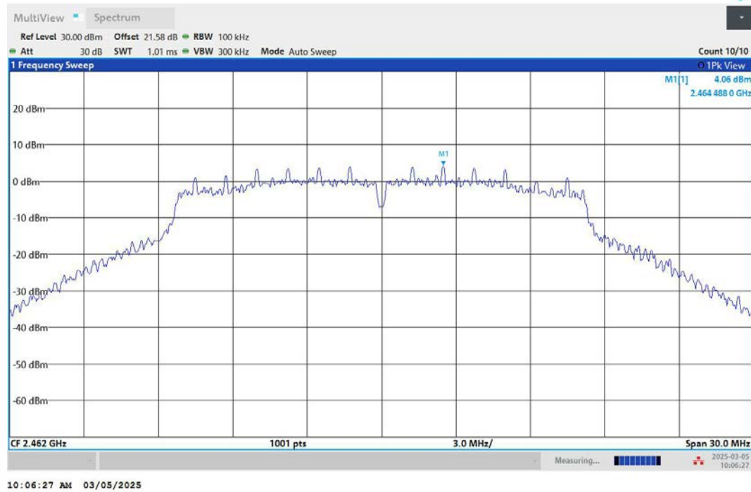
11G-Ant2-2462-0~Reference-PASS
