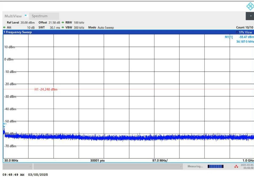
11B-Ant2-2462-30~1000-PASS
