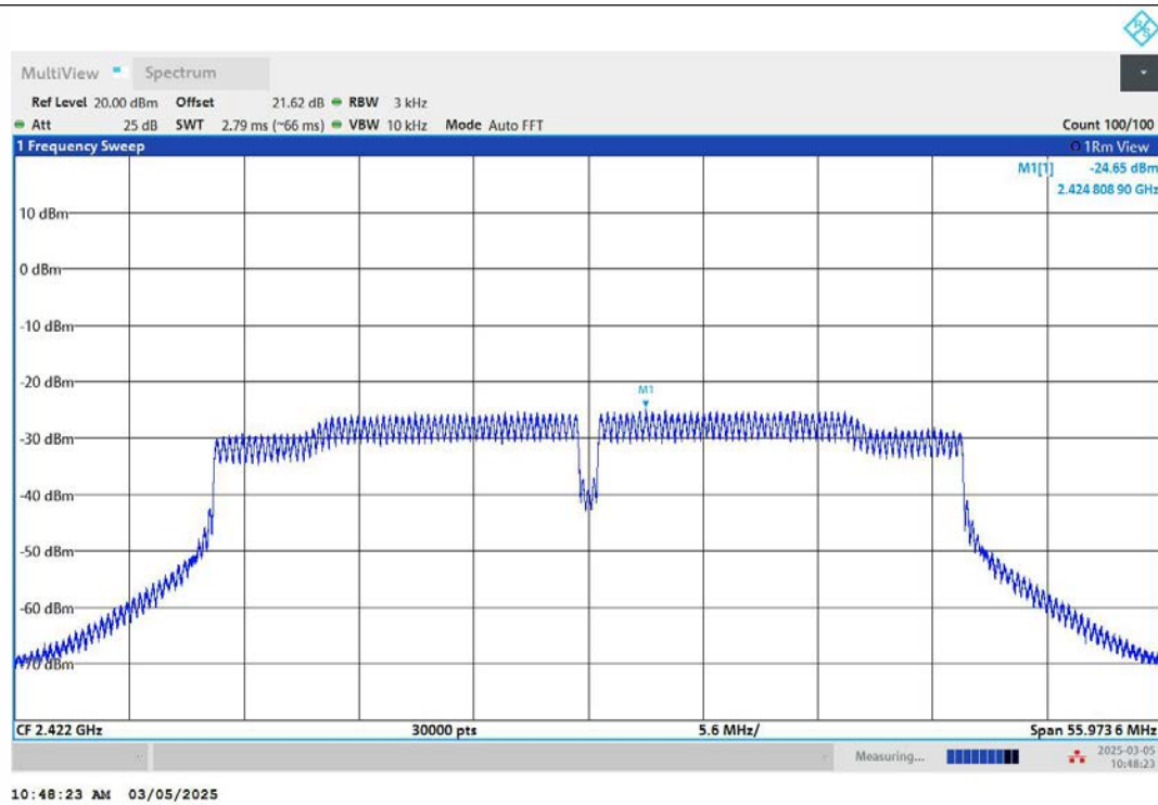
11N40MIMO-Ant2-2422-PASS
