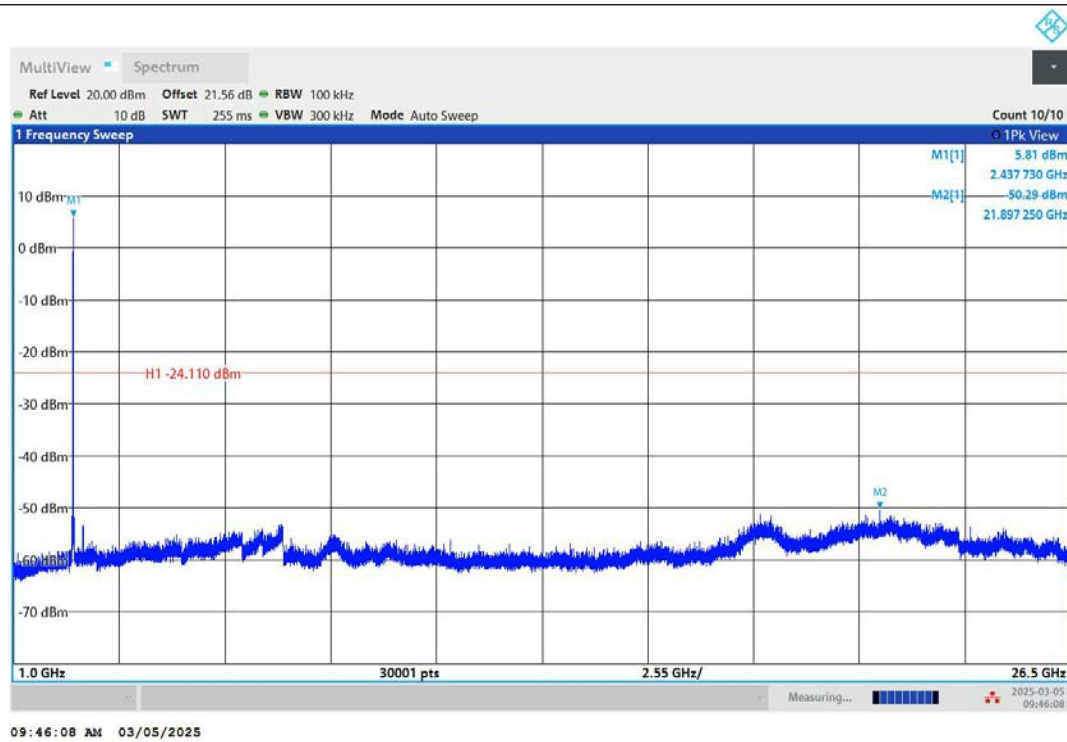
11B-Ant2-2437-1000~26500-PASS
