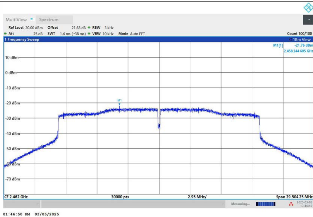
11AX20MIMO-Ant2-2462-PASS
