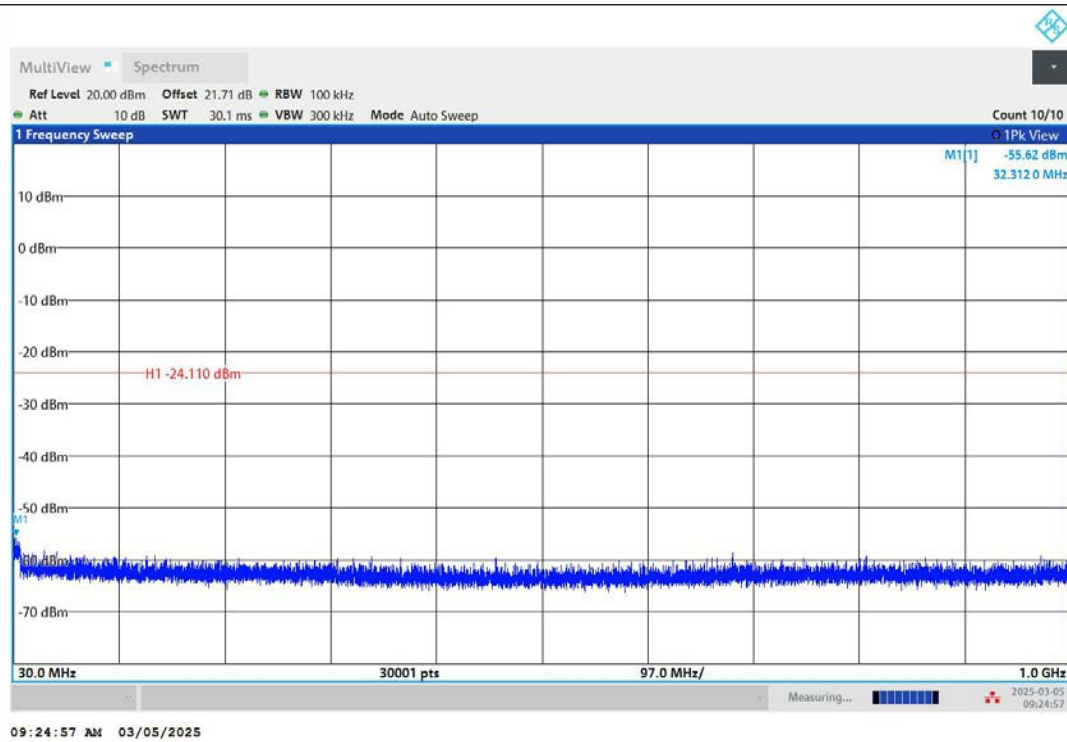
11B-Ant2-2412-30~1000-PASS
