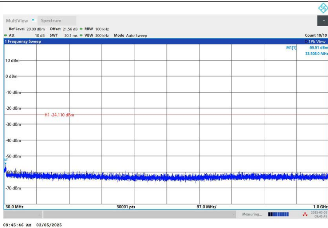
11B-Ant2-2437-30~1000-PASS
