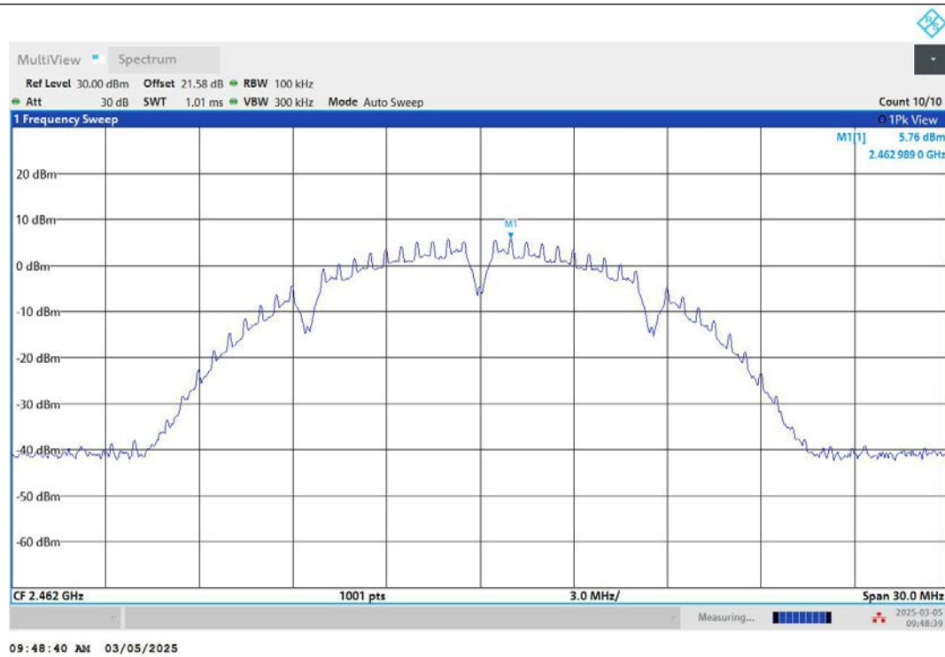
11B-Ant2-2462-0~Reference-PASS
