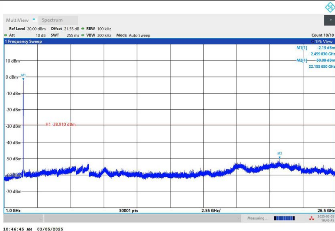
11N40MIMO-Ant1-2422-0~Reference-PASS
