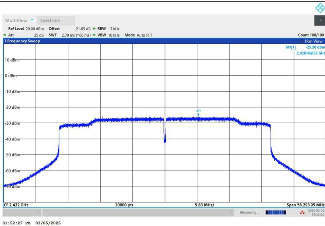
11AX40MIMO-Ant2-2422-PASS
