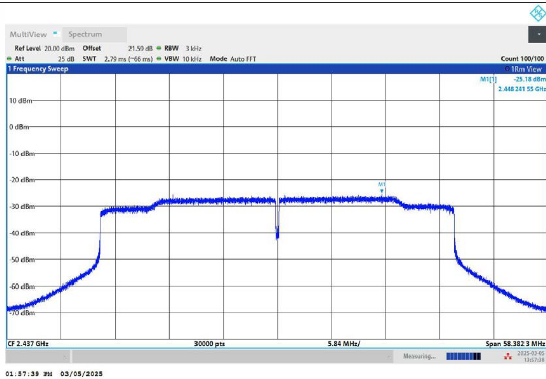
11AX40MIMO-Ant2-2437-PASS
