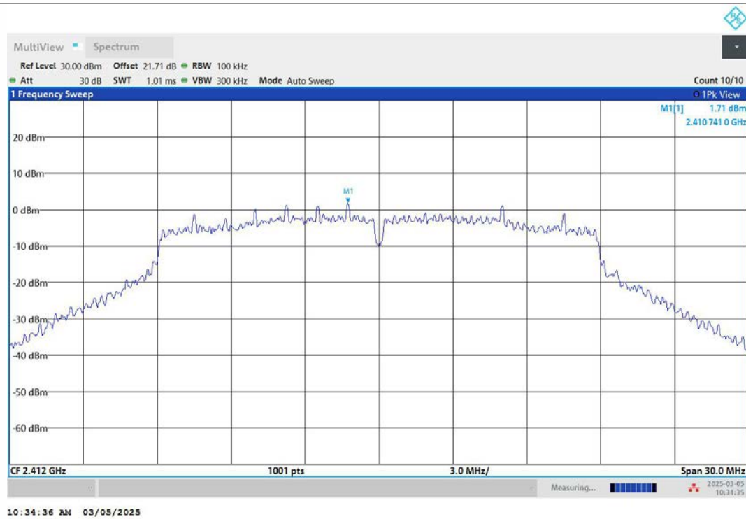
11N20MIMO-Ant2-2412-0~Reference-PASS
