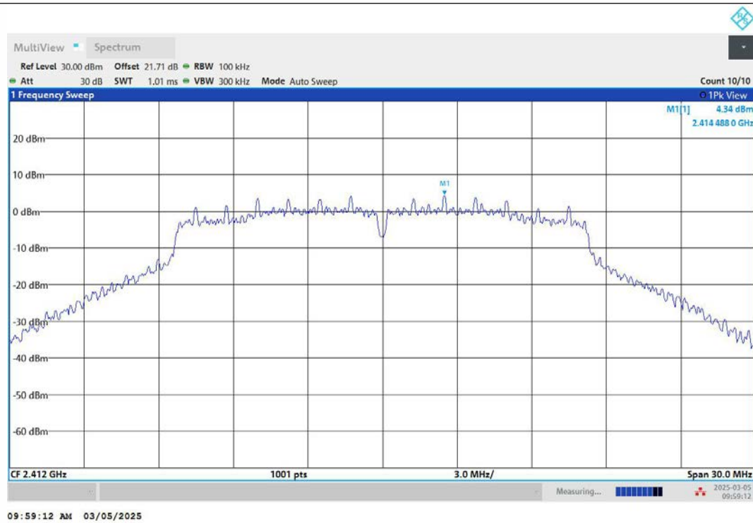
11G-Ant2-2412-0~Reference-PASS
