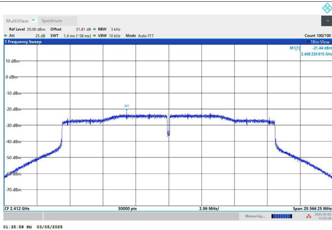
11AX20MIMO-Ant2-2412-PASS
