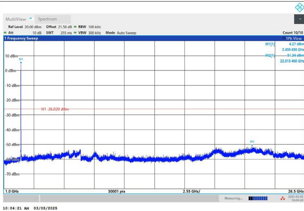
11G-Ant2-2437-1000~26500-PASS
