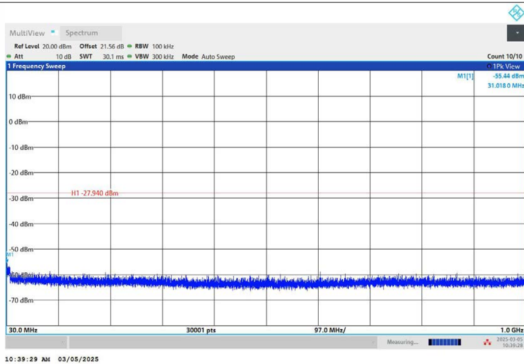
11N20MIMO-Ant2-2437-30~1000-PASS
