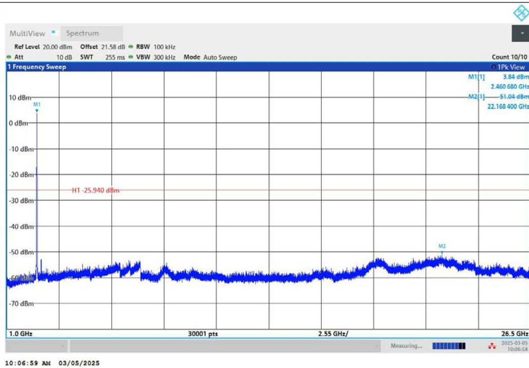
11G-Ant2-2462-1000~26500-PASS
