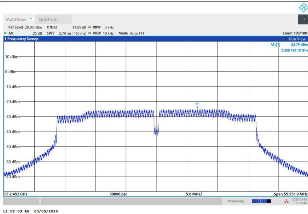
11N40MIMO-Ant2-2452-PASS
