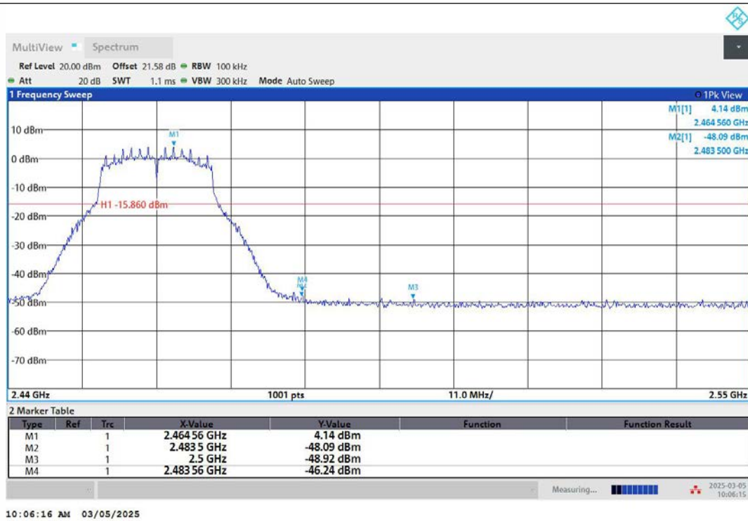
11G-Ant2-2462-PASS
