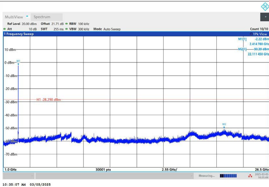
11N20MIMO-Ant2-2412-1000~26500-PASS
