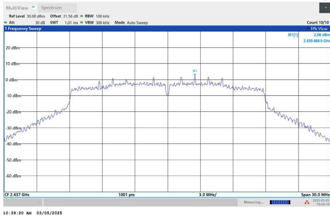
11N20MIMO-Ant2-2437-0~Reference-PASS
