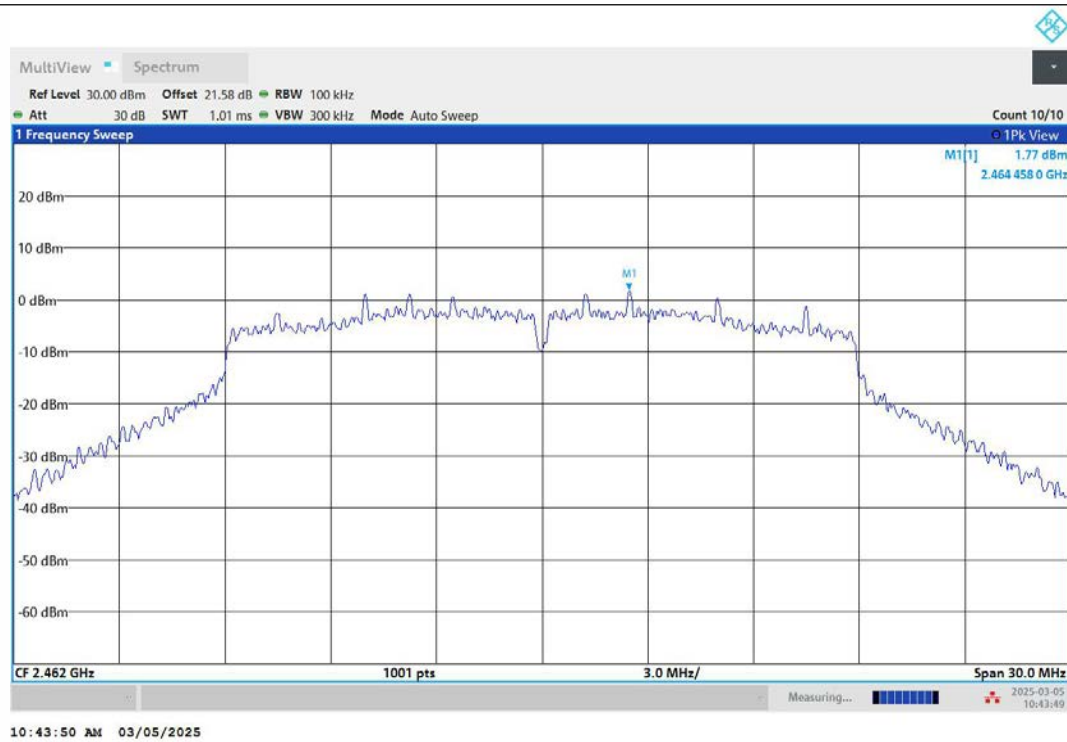
11N20MIMO-Ant2-2462-0~Reference-PASS
