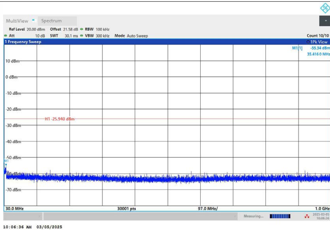
11G-Ant2-2462-30~1000-PASS
