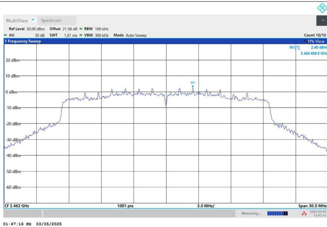
11AX20MIMO-Ant2-2462-0~Reference-PASS
