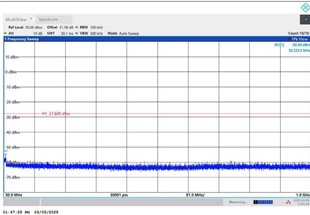
11AX20MIMO-Ant2-2462-30~1000-PASS
