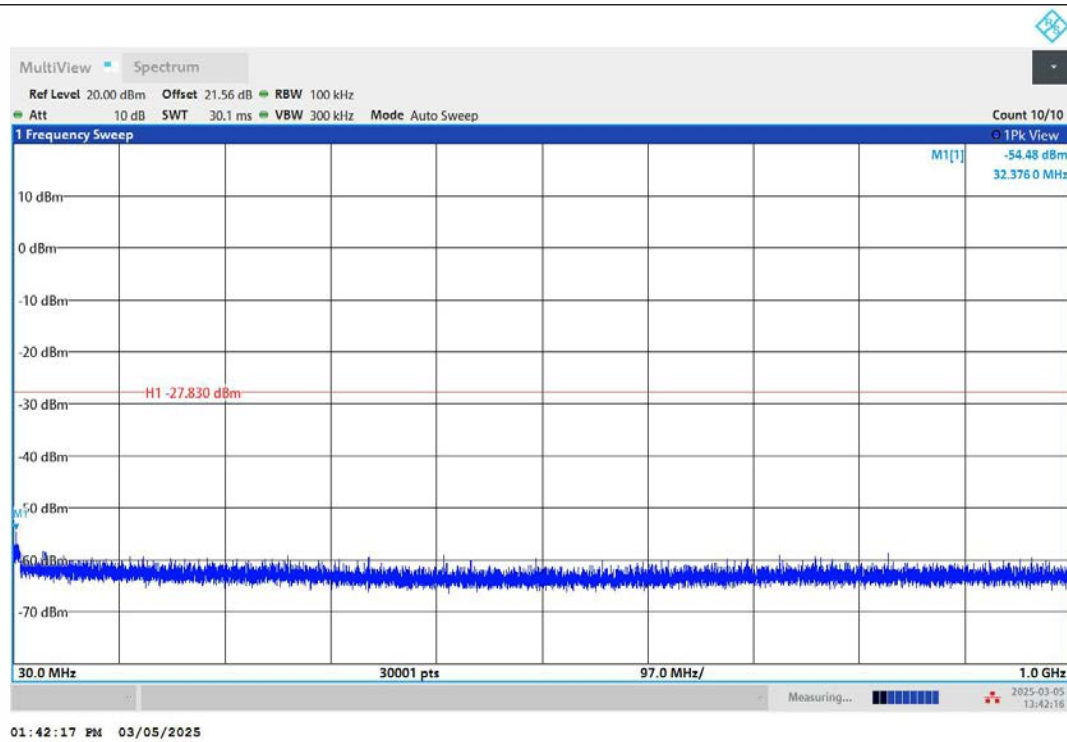
11AX20MIMO-Ant2-2437-30~1000-PASS
