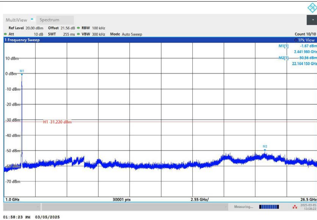
11AX40MIMO-Ant2-2437-1000~26500-PASS
