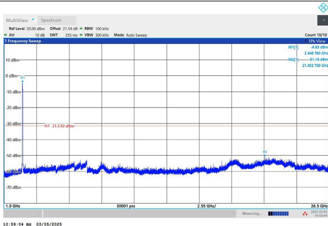
11N40MIMO-Ant1-2452-0~Reference-PASS
