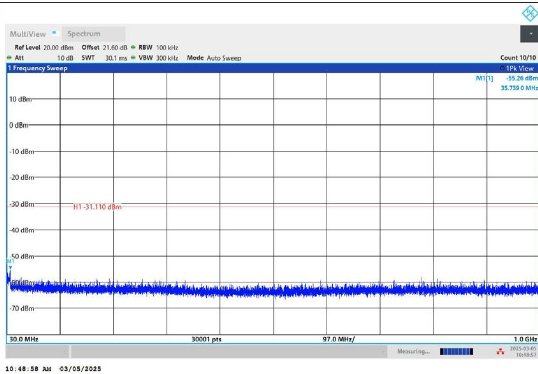
11N40MIMO-Ant2-2422-30~1000-PASS
