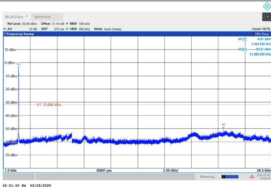
11AX40MIMO-Ant1-2452-0~Reference-PASS
