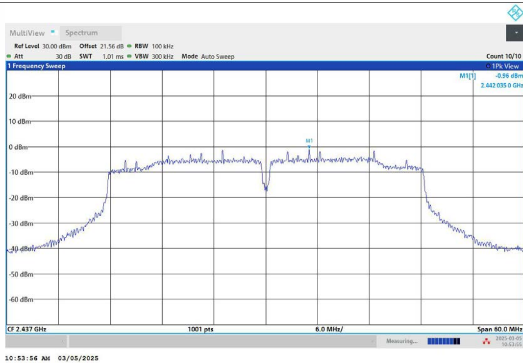
11N40MIMO-Ant2-2437-0~Reference-PASS
