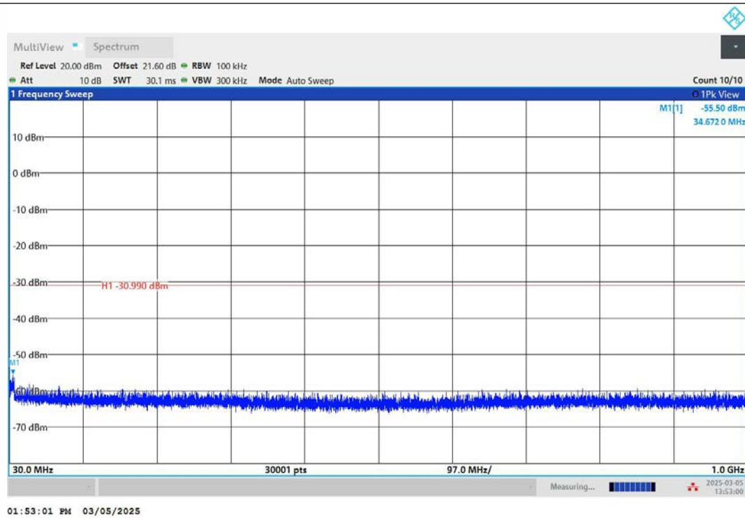
11AX40MIMO-Ant2-2422-30~1000-PASS
