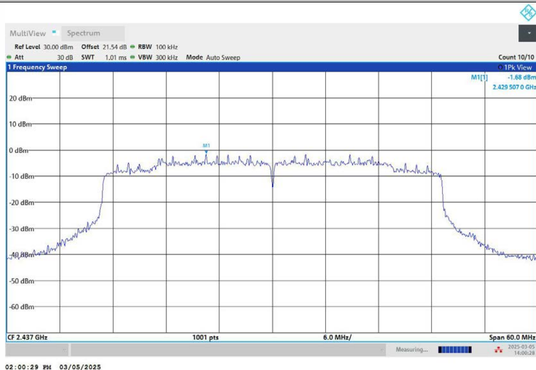
11AX40MIMO-Ant1-2437-30~1000-PASS
