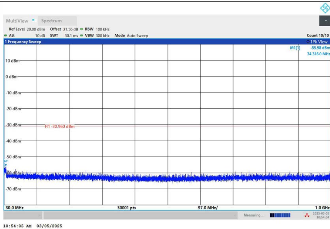
11N40MIMO-Ant2-2437-30~1000-PASS
