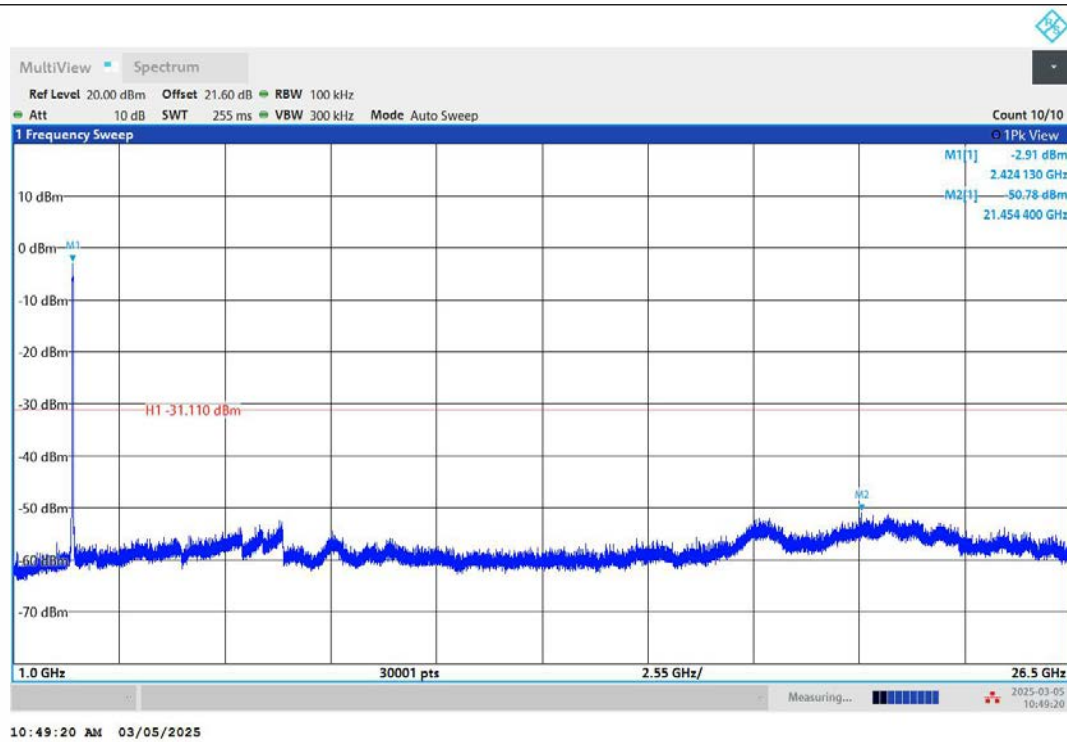
11N40MIMO-Ant2-2422-1000~26500-PASS
