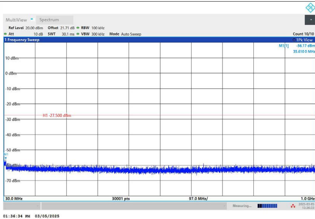
11AX20MIMO-Ant2-2412-30~1000-PASS
