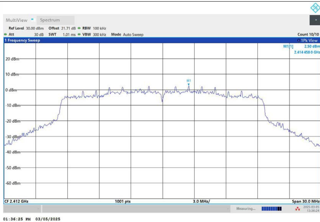
11AX20MIMO-Ant2-2412-0~Reference-PASS
