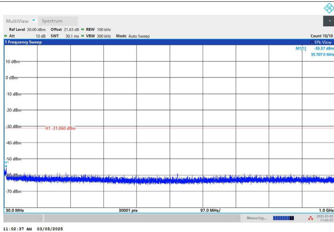
11N40MIMO-Ant2-2452-30~1000-PASS
