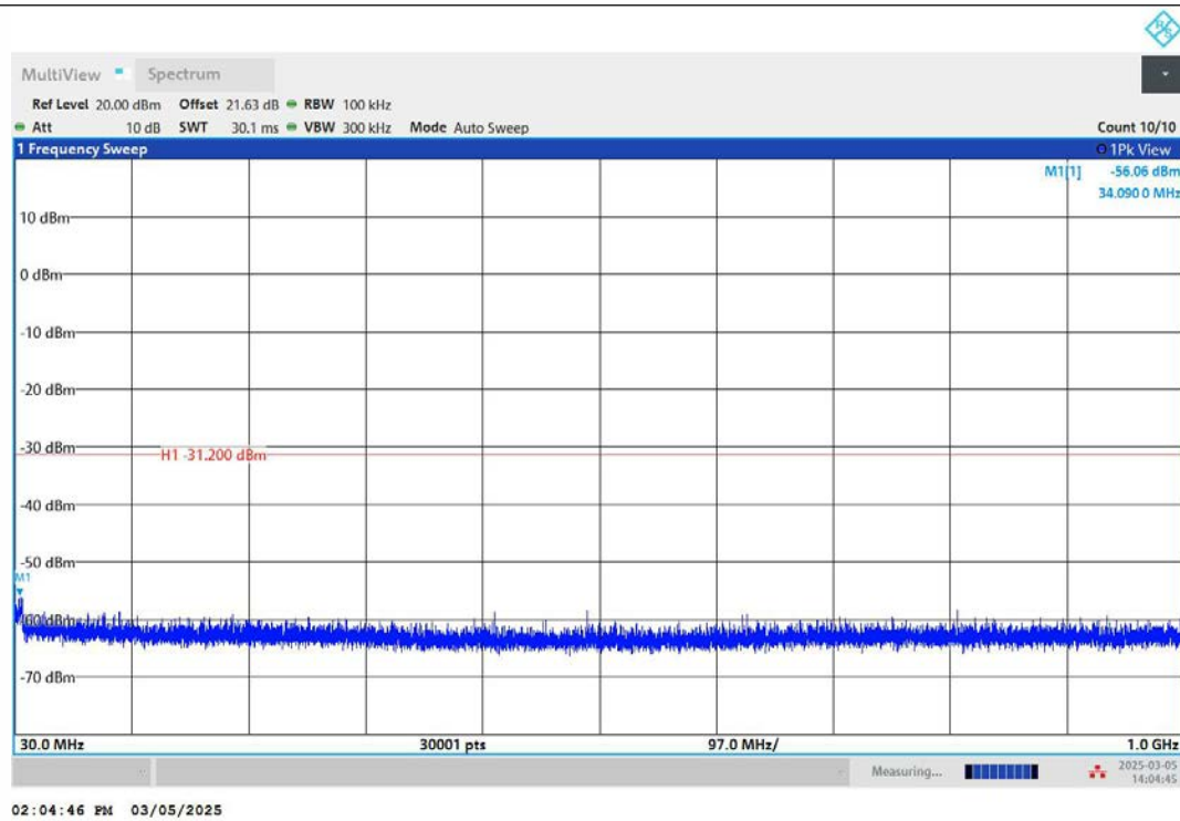
11AX40MIMO-Ant2-2452-30~1000-PASS
