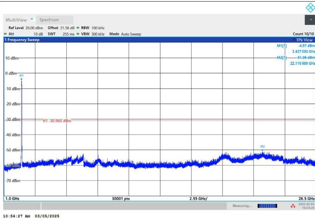
11N40MIMO-Ant2-2437-1000~26500-PASS
