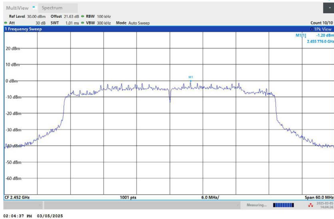
11AX40MIMO-Ant2-2452-0~Reference-PASS
