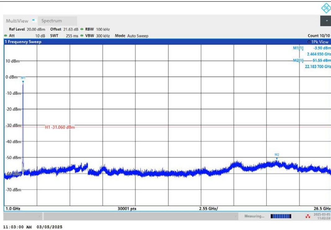
11N40MIMO-Ant2-2452-1000~26500-PASS
