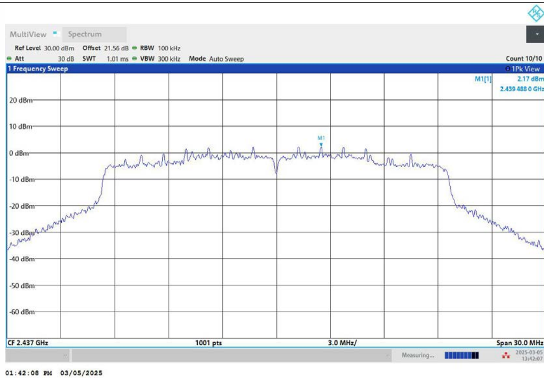
11AX20MIMO-Ant2-2437-0~Reference-PASS
