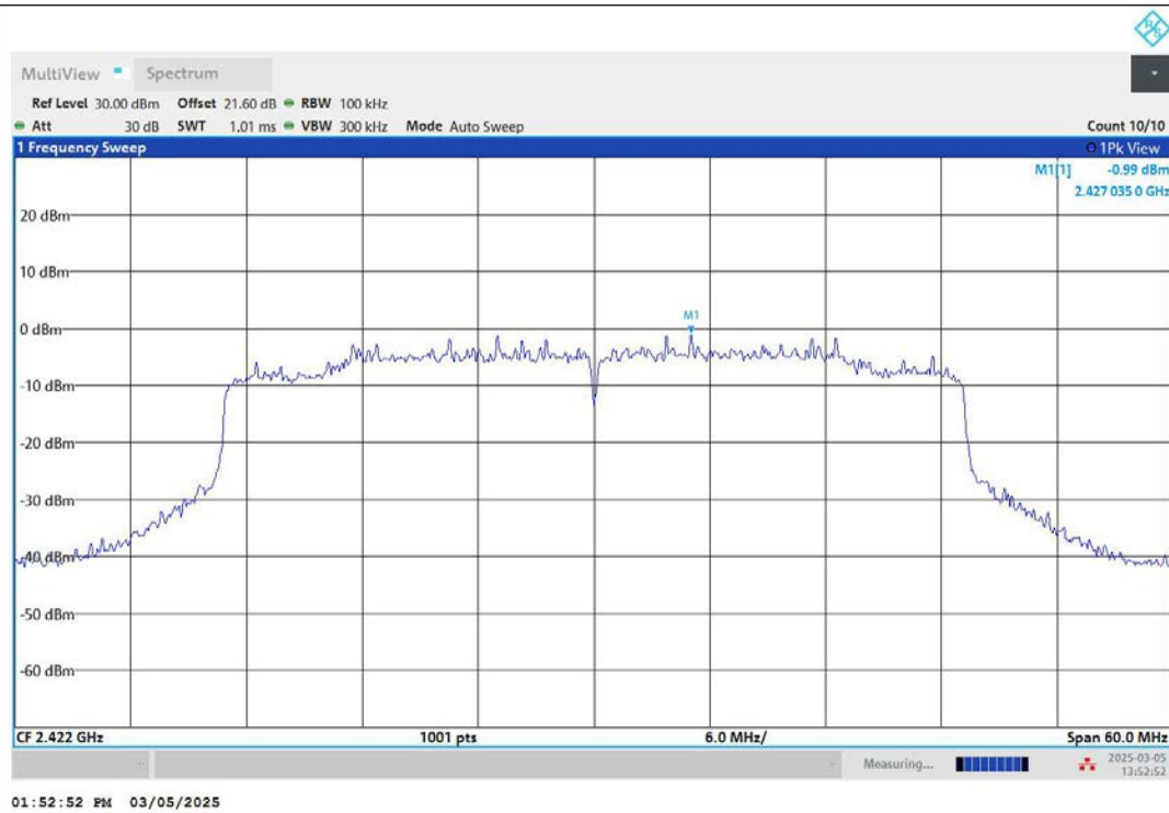
11AX40MIMO-Ant2-2422-0~Reference-PASS
