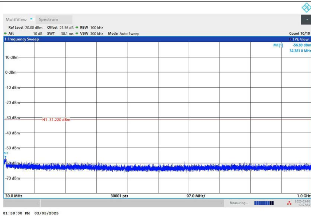
11AX40MIMO-Ant2-2437-30~1000-PASS
