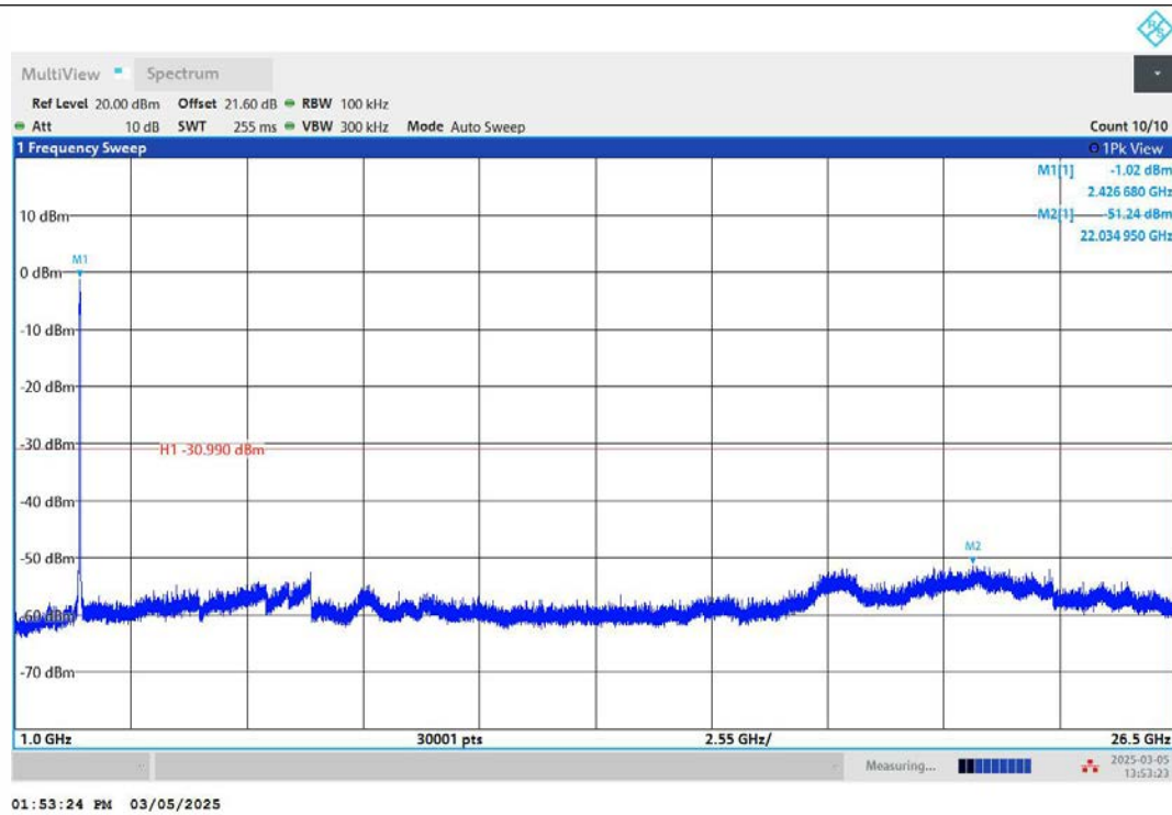
11AX40MIMO-Ant2-2422-1000~26500-PASS
