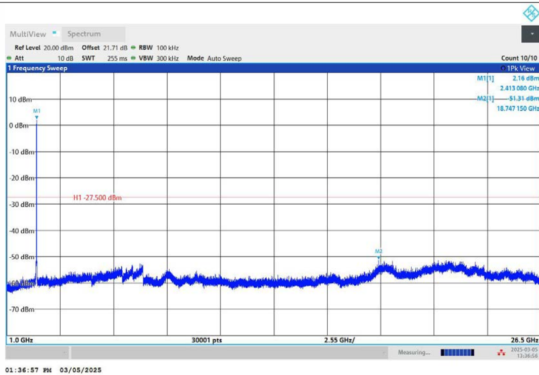
11AX20MIMO-Ant2-2412-1000~26500-PASS
