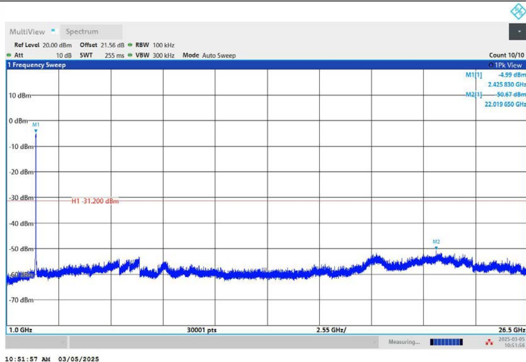
11N40MIMO-Ant1-2437-0~Reference-PASS
