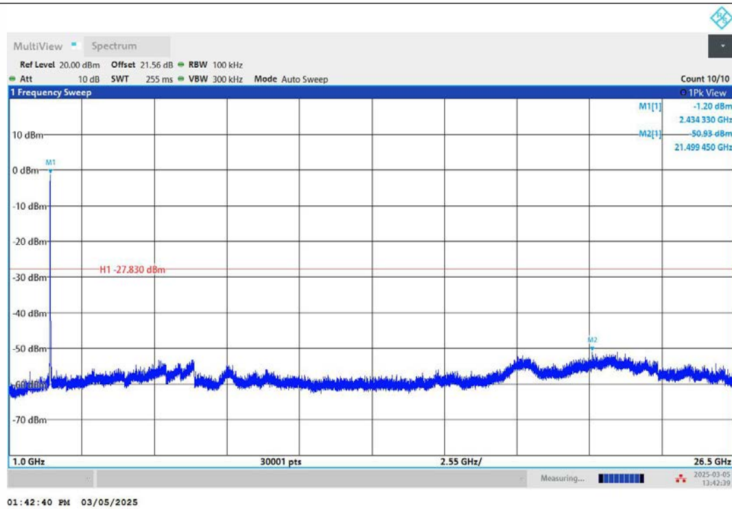
11AX20MIMO-Ant2-2437-1000~26500-PASS
