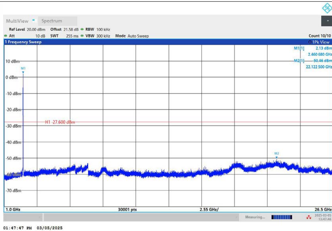
11AX20MIMO-Ant2-2462-1000~26500-PASS
