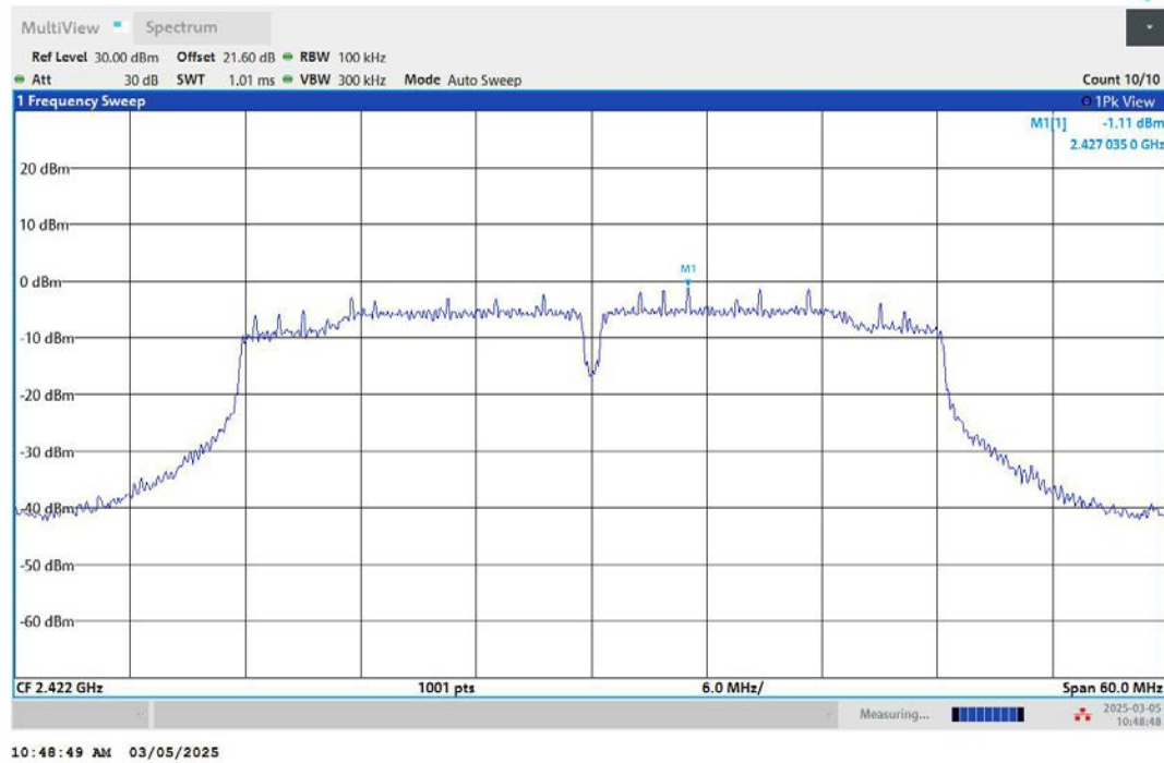
11N40MIMO-Ant2-2422-0~Reference-PASS
