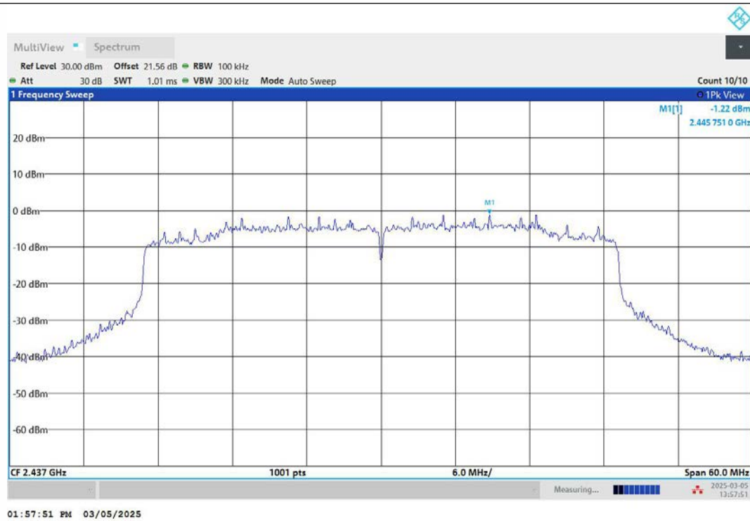
11AX40MIMO-Ant2-2437-0~Reference-PASS
